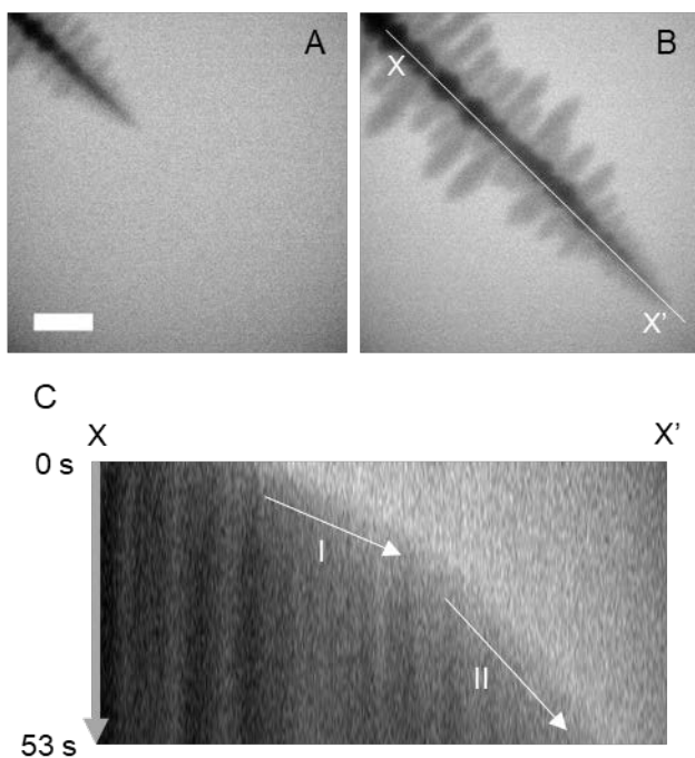
Supplementary Figure S2. Measurement of the maximum growth rate of a dendritic crystal.
