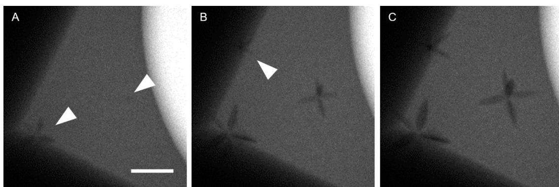
Figure 2. A series of bright-field TEM images of the crystallization of a dendrite from an aqueous solution of \text{NaClO}_3 mixing with acetone. This event is the same as that shown in Supplementary Video 1, recorded ten minutes after mixing the solutions. The three images were captured at about 10 (A), 15 (B), and 20 s (C), respectively, after the area had been irradiated by the electron beam. The white arrowheads indicate the positions at which crystallizations occurred. The edge of the a-SiN window is visible in the top and bottom left-hand corners of the image, and a bubble is visible in the top right-hand corner of each image. The electron dose rate was 37 \text{ e}^- \text{ nm}^{-2} \cdot \text{s}^{-1} . The scale bar is 2 \text{ }\mu\text{m} .
