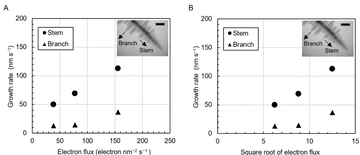
Figure 6. Growth rates of dendrites as a function of the electron dose rate (A) or the square root of the electron dose rate (B) under the experimental conditions. The inset shows a typical dendritic crystal and the directions in which the growth rate was measured. The scale bar in inset is 1 μm.
