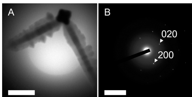
Figure 4. Identification of a crystal that formed in a mixed solution of water and acetone. (A) The dendritic crystal and (B) its SAED pattern, corresponding to the [001] SAED pattern of NaCl (ICDD PDF No. 5-628). The measured d-spacings d_{hkl} are d_{200} = 2.94 \text{ \AA} and d_{020} = 2.93 \text{ \AA} . The circular object in (A) is a selected-area diffraction aperture. The scale bars are 2 \text{ }\mu\text{m} (A) and 5 \text{ nm}^{-1} (B).
