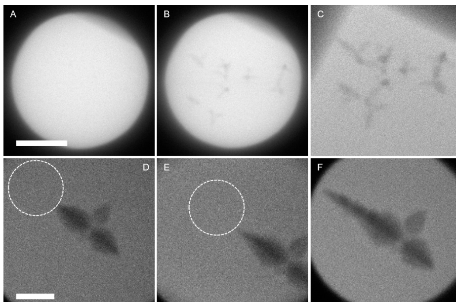
Figure 3. Electron-beam-induced crystallization. (A–C) Series of bright-field TEM images of beam-induced nucleation. This event is the same as that shown in Supplementary Video 2.
