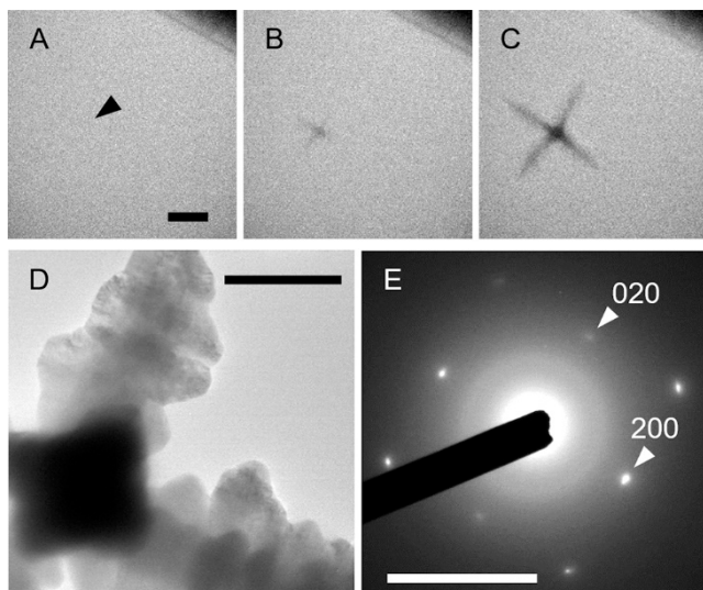
Figure 5. Crystallization of dendrites in a saturated acetone solution of \text{NaClO}_3 . (A–C) A series of bright-field TEM images of a crystallizing dendrite. Images were captured within 1 s (A), and at about 5 s (B) and 15 s (C) after the area had been irradiated by the electron beam. The black arrowheads indicate the positions at which nucleation occurred. The edge of the a-SiN window is visible in the top right-hand corner. The electron dose rate was 78 \text{ e}^- \text{ nm}^{-2} \cdot \text{s}^{-1} . The scale bar is 1 \mu\text{m} , and the scale of (B, C) is the same as that of (A). (D–E) Identification of a formed crystal: (D) dendritic crystal (which was different from the crystal in A–C) and (E) its SAED pattern, corresponding to that of NaCl (JCPDS Card No. 5-0628) with a crystallographic orientation of [001]. The measured d-spacings d_{hkl} are d_{200} = 2.81 \text{ \AA} and d_{020} = 2.84 \text{ \AA} . The scale bars are 1 \mu\text{m} (D) and 5 \text{nm}^{-1} (E).
