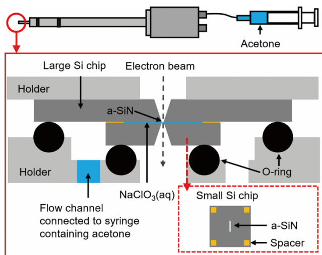
Figure 1. Schematic representations of the TEM holder and a cross-section of the liquid cell.
