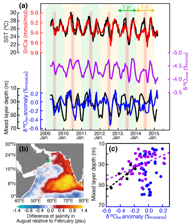
Figure 2. Modern coral records at a biweekly resolution from the Arabian Sea. (a) Sr/Ca (red line) and OISST v2.1 (black line, Banzon et al., 2020), \delta^{18}\text{O}_{\text{coral}} (purple line), \delta^{18}\text{O}_{\text{sw}} anomaly (blue line; values relative to the wintertime mean after detrending) and mixed layer depth measured by Argo float (black line). Yellow/green shadings indicate one year (January–December). Red shadings mark August. (b) Sea surface salinity anomalies in August 2013 relative to February 2014 (Aquarius OISST; 1 \times 1^\circ grid). Note the freshening (blue colors) of the surface waters along the Somalian and the southern Arabian coast. Charts are computed with Live Access Server LAS8.6. The star indicates the sample site of our fossil and modern Arabian corals. (c) Scatter plot of mixed layer depth versus monthly \delta^{18}\text{O}_{\text{sw}} anomalies and max- \delta^{18}\text{O}_{\text{sw-reduc}} (purple: SW monsoon seasons, blue: winter months, black: max- \delta^{18}\text{O}_{\text{sw-reduc}} ). The dotted black (purple) line: linear regression line of mixed layer depth versus max- \delta^{18}\text{O}_{\text{sw-reduc}} ( \delta^{18}\text{O}_{\text{sw}} anomaly in the SW monsoon seasons).
