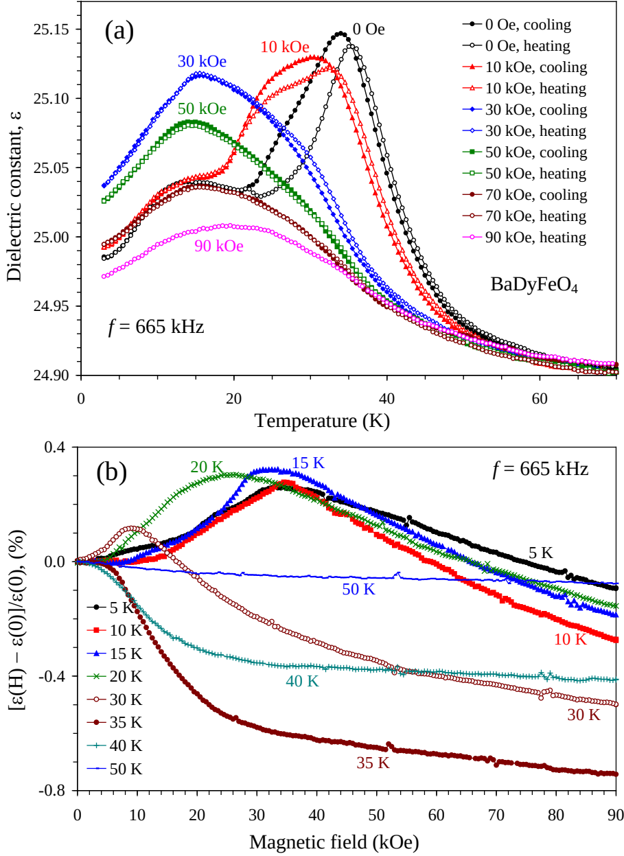
Figure 8. (a) Temperature dependence of dielectric constant in BaDyFeO 4 . Measurements were performed on cooling (filled symbols) and heating (empty symbols) at H = 0, 10, 30, 50, 70 , and 90 kOe. Curves at one frequency of 665 kHz are shown. (b) Magnetic-field dependence of relative changes of dielectric constant (magnetodielectric effects) in BaDyFeO 4 at T = 5, 10, 15, 20, 30, 35, 40 , and 50 K. Curves at one frequency of 665 kHz are shown.
