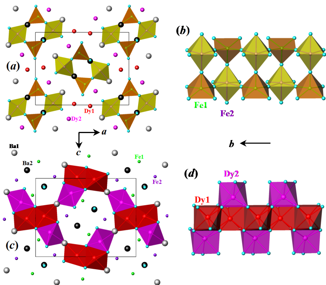
Figure 1. Crystal structure of \text{BaDyFeO}_4 . (a) Connection of the \text{Fe1O}_5 and \text{Fe2O}_6 polyhedra viewed along the b axis. (b) One chain of the \text{Fe1O}_5 and \text{Fe2O}_6 polyhedra along the b axis. (c) Connection of the \text{Dy1O}_7 and \text{Dy2O}_7 polyhedra viewed along the b axis. (d) One chain of the \text{Dy1O}_7 and \text{Dy2O}_7 polyhedra along the b axis.
