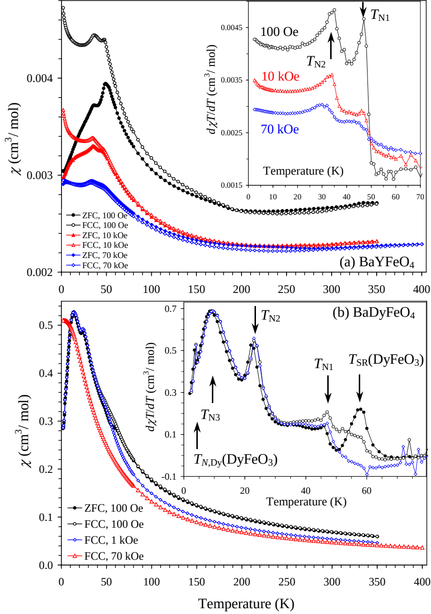
Figure 3. ZFC (filled symbols) and FCC (empty symbols) dc magnetic susceptibility ( \chi = M/H ) curves of (a) BaYFeO 4 and (b) BaDyFeO 4 at different magnetic fields. The insets show the d(\chi T)/dT versus T curves to emphasize magnetic anomalies. T_N : Néel temperature, T_{SR} : spin-reorientation transition temperature.
