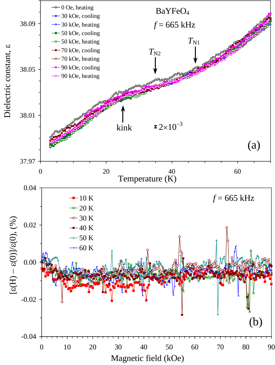
Figure 9. (a) Temperature dependence of dielectric constant in BaYFeO 4 . Measurements were performed on cooling (filled symbols) and heating (empty symbols) at H = 0, 30, 50, 70 , and 90 kOe. Curves at one frequency of 665 kHz are shown. An error bar of 2 \times 10^{-3} is shown – a dielectric constant anomaly of this order was detected in Ref. [8]. (b) Magnetic-field dependence of relative changes of dielectric constant (magnetodielectric effects) in BaYFeO 4 at T = 10, 20, 30, 40, 50 , and 60 K. Curves at one frequency of 665 kHz are shown.
