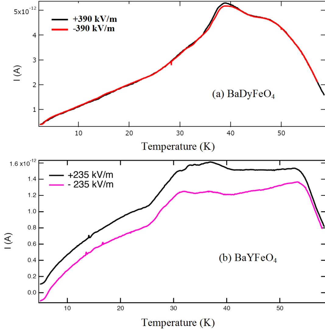
Figure 10. Results of pyroelectric current measurements in (a) \text{BaDyFeO}_4 and (b) \text{BaYFeO}_4 .
