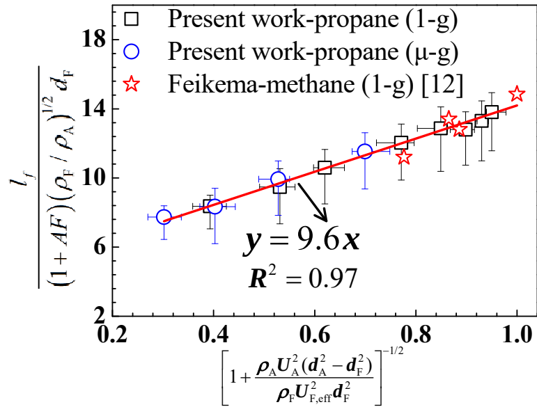
Figure 9. Correlation of the critical flame length (axial location) at blowout in both normal gravity and microgravity.
