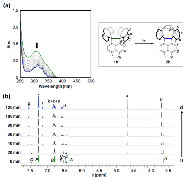
Figure 2. (a) Change in UV/Vis spectrum of 1b (green) to 2b (blue) in CHCl 3 (every 5 min) and (b) change in 1 H NMR spectrum of 1b (green) to 2b (blue) in CDCl 3 upon photoirradiation at 365 nm (Spectrofluorometer: 150 W, Xe lamp, slit width: 10 nm). The residual proton signal of the solvent (CHCl 3 , \delta = 7.26 ppm) is marked with an asterisk.
