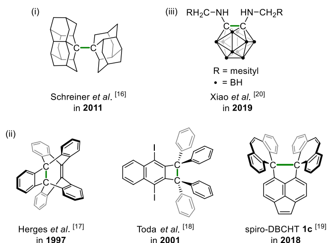
Figure 1. Previously reported molecules. Three approaches have been used to make compounds with an elongated C–C bond, which is surrounded only by (i) sp 3 -hybridized carbons, (ii) sp 2 -hybridized carbons, or (iii) heteroatoms.
