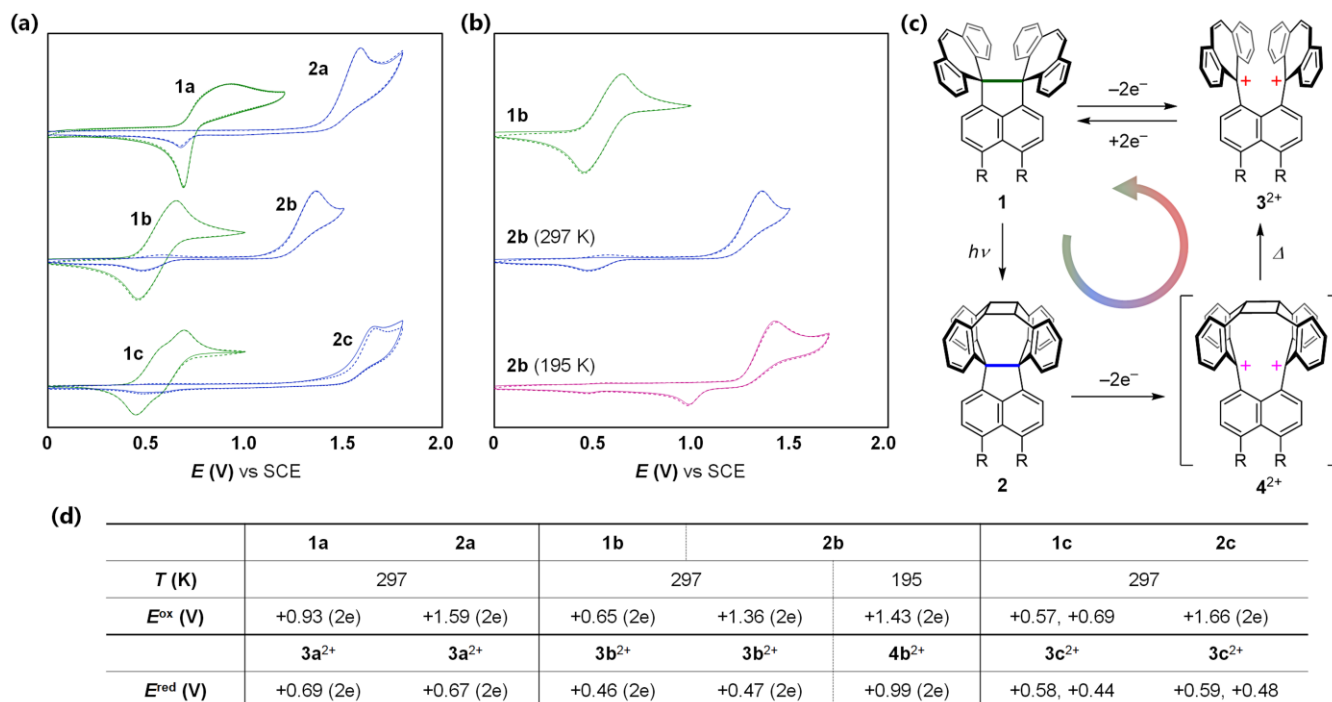
Figure 3. Cyclic voltammograms of (a) 1 and 2 at 297 K and (b) 1b , 2b (at 297 K), and 2b (at 195 K) in CH 2 Cl 2 containing 0.1 M Bu 4 NBF 4 as a supporting electrolyte (scan rate 0.1 V s -1 , Pt electrode). The second cycles are shown by a dotted line. (c) Mechanism of redox interconversion. (d) Redox potentials are summarized and peak potentials are shown as E^{\text{ox}} and E^{\text{red}} . [a (R = H); b (R,R = CH 2 -CH 2 ); c (R,R = CH=CH)]
