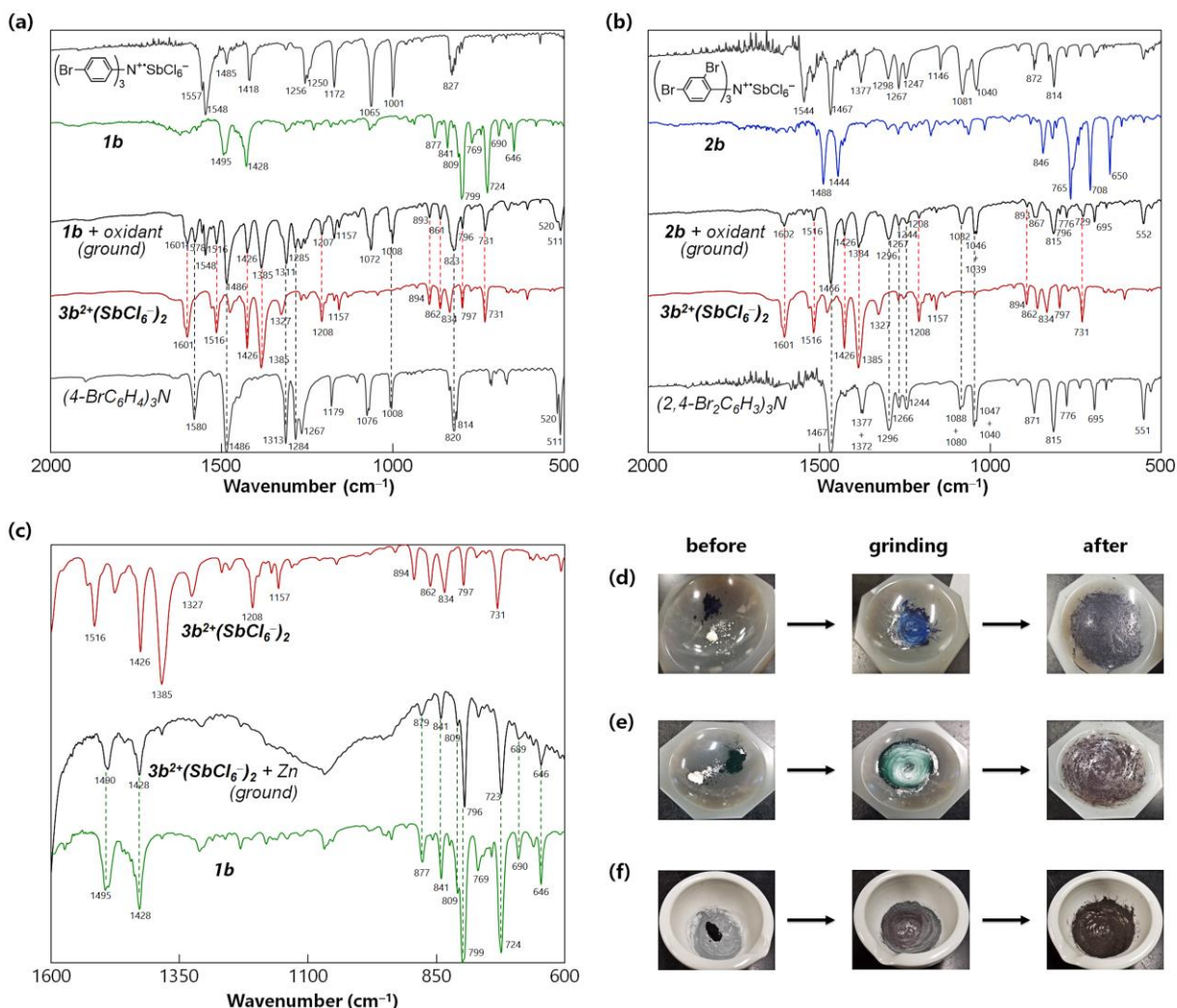
Figure 5. (a) Solid-state oxidation of 1b with two equivalents of (4-BrC 6 H 4 ) 3 N + SbCl 6 - was confirmed by IR spectroscopy. (b) Solid-state oxidation of 2b with two equivalents of (2,4-Br 2 C 6 H 3 ) 3 N + SbCl 6 - as a stronger oxidant was confirmed by IR spectroscopy. (c) Solid-state reduction of 3b 2+ (SbCl 6 ) 2 with an excess amount of Zn powder was confirmed by IR spectroscopy. Photographs of mechano-oxidation of (d) 1b with (4-BrC 6 H 4 ) 3 N + SbCl 6 - and (e) 2b with (2,4-Br 2 C 6 H 3 ) 3 N + SbCl 6 - , and (f) mechano-reduction of 3b 2+ (SbCl 6 ) 2 with an excess amount of Zn powder.
