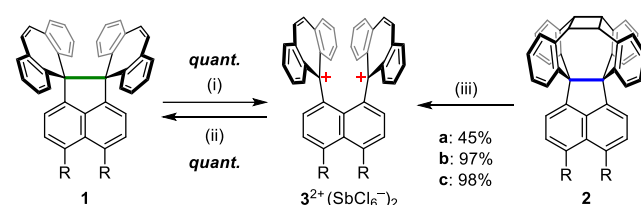
Scheme 2. Redox interconversion among 1 , 2 , and 3 2+ (SbCl 6 ) 2 . (i) (4-BrC 6 H 4 ) 3 N + SbCl 6 - (2.0 eq)/CH 2 Cl 2 . (ii) Zn (excess)/CH 3 CN or THF. (iii) (2,4-Br 2 C 6 H 3 ) 3 N + SbCl 6 - (2.0 eq)/CH 2 Cl 2 . [a (R = H); b (R,R = CH 2 -CH 2 ); c (R,R = CH=CH)]
