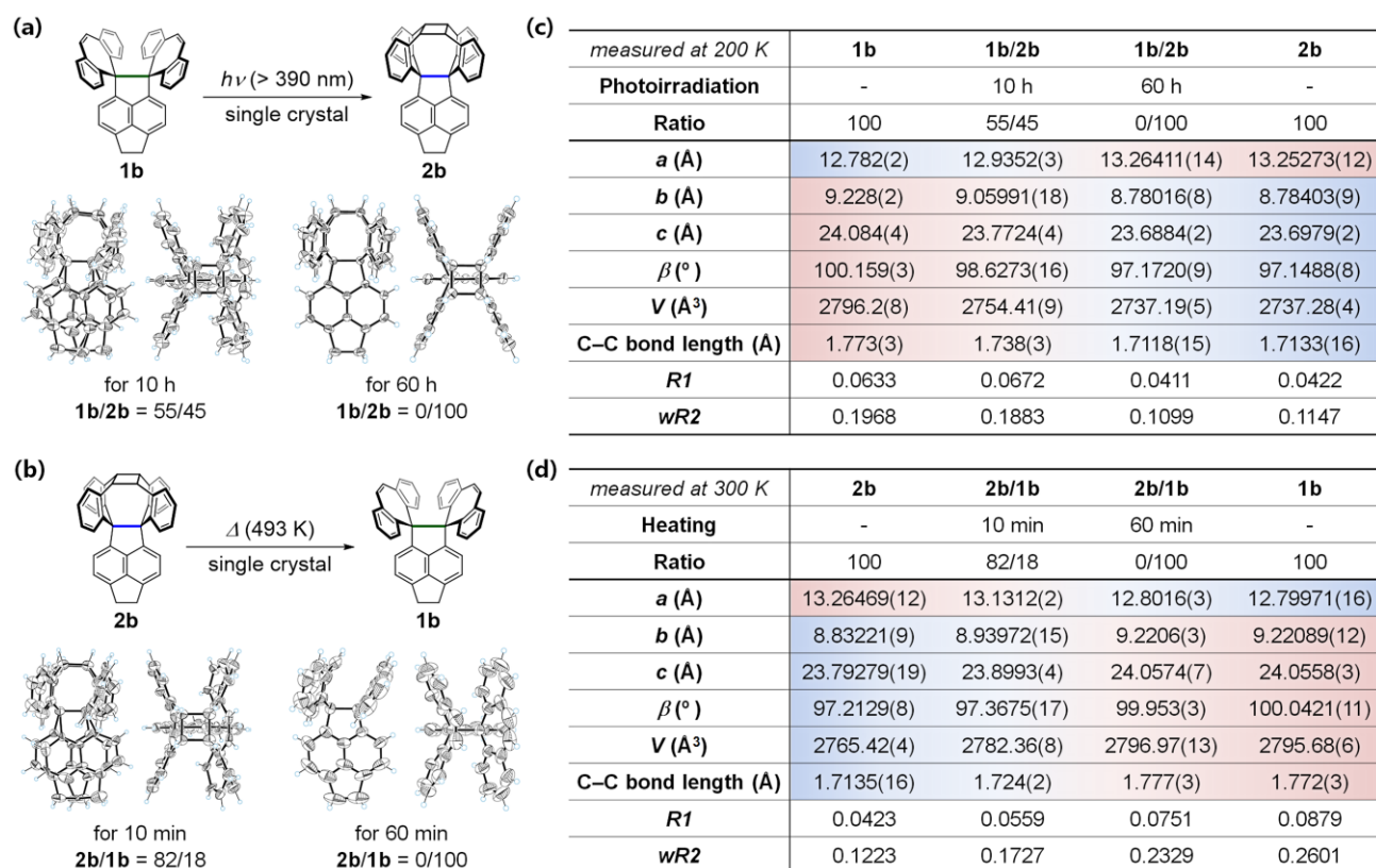
Figure 4. (a) Upon photoirradiation of a single crystal of 1b with \lambda > 390 nm for 10 h and 60 h, the SCSC photocycloaddition reaction proceeded in respective yields of 45% and 100%, which were determined by a single-crystal X-ray analysis at 200 K. (b) When a single crystal of 2b was heated at 493 K for 10 min and 60 min, SCSC thermal cycloreversion proceeded in respective yields of 18% and 100%, which were determined by a single-crystal X-ray analysis at 300 K. Thermal ellipsoids are shown at the 30% probability level for intermediates and the 50% probability level for completely converted samples. (c,d) The crystallographic data for 1b and 2b are summarized in the table.
