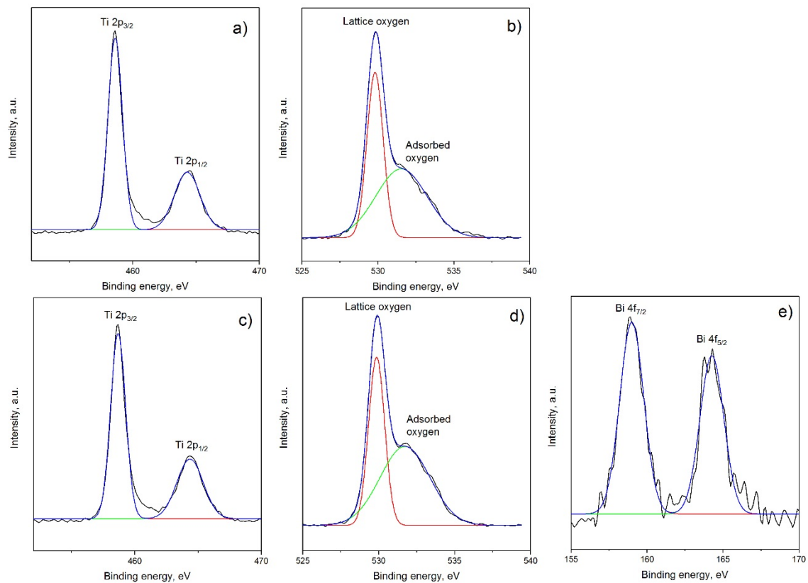
Figure 4. High resolution XPS spectra of PC500-based samples: a) Ti 2p spectrum of sample PC500; b) O 1s spectrum of sample PC500; c) Ti 2p spectrum of sample PC500Bi30; d) O 1s spectrum of sample PC500Bi30; e) Bi 4f spectrum of sample PC500Bi30
