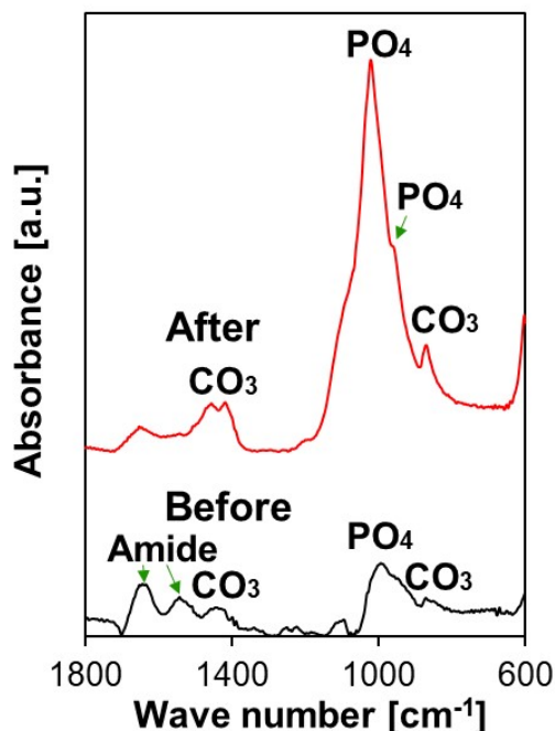
Figure 4. FT-IR spectra of the surfaces of the dentin substrates before and after the LAB process.
