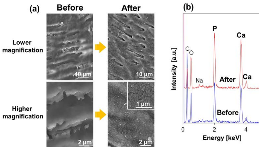
Figure 2. (a) Higher and lower magnifications of SEM images, (b) SEM-EDX spectra of the surfaces of the dentin substrates before and after the LAB process. The C peak in (b) corresponds to the carbon coating and the substrates.
