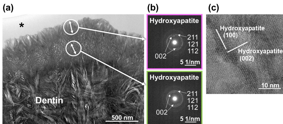
Figure 10 (a) Cross-sectional bright-field TEM image, (b) SAED patterns obtained from the circled areas in (a), and (c) HRTEM image (upper region of the surface layer), of the LAB-processed dentin substrate. Two-way arrows in (a) indicate the direction of c -axis orientation of hydroxyapatite nanocrystals, and * indicates the protective ink layer.
