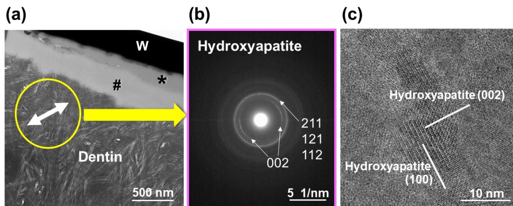
Figure 7 (a) Cross-sectional bright-field TEM image, (b) SAED pattern obtained from the circled area in (a), and (c) HRTEM image of the unprocessed dentin substrate. Two-way arrow in (a) indicates the direction of c -axis orientation of hydroxyapatite nanocrystals. W, *, and # in (a) indicate the W coating, the protective ink layer, and the organic layer, respectively.
