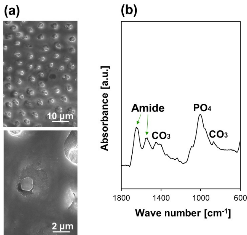
Figure 5 (a) Higher (bottom) and lower (top) magnifications of SEM images and (b) FT-IR spectrum of the surface of the dentin substrate after the comparison test; the substrate was immersed in the CP solution for 30 min without laser irradiation.
