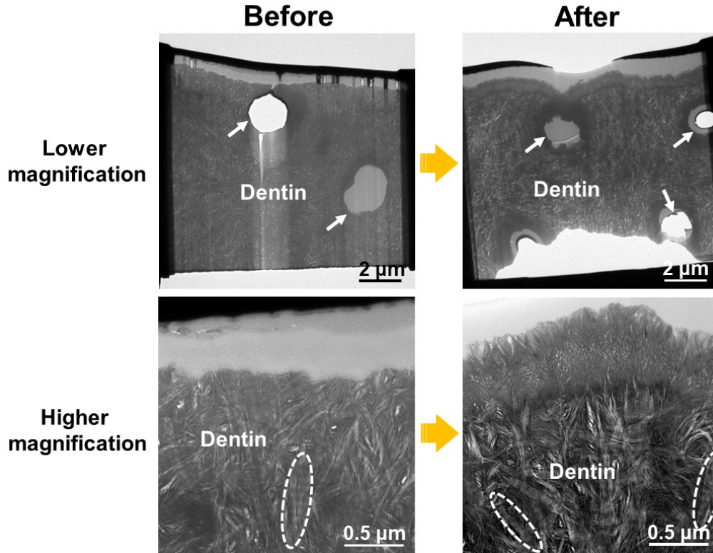
Figure 9 Higher and lower magnifications of cross-sectional bright-field TEM images of the dentin substrates before and after the LAB process. Arrows indicate dentinal tubules, and dotted circles indicate D-band structure typical of type I collagen fibrils.
