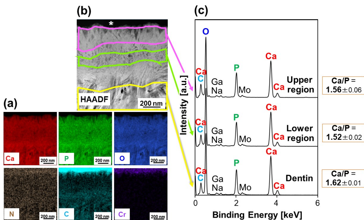
Figure 11 (a) Cross-sectional STEM-EDX elemental mappings (Ca, P, O, N, C, Cr), the corresponding HAADF image, and (c) STEM-EDX spectra of the boxed areas in (b), of the LAB-
