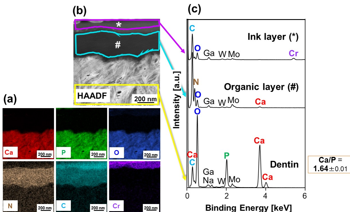
Figure 8 (a) Cross-sectional STEM-EDX elemental mappings (Ca, P, O, N, C, Cr), (b) the corresponding HAADF image, and (c) STEM-EDX spectra of the boxed areas in (b), of the unprocessed dentin substrate. * and # in (b) indicate the protective ink layer and the organic layer, respectively. The averaged Ca/P elemental ratio in the right-most box in (c) was calculated from the peak areas of Ca and P in the STEM-EDX spectra.
