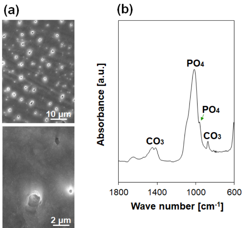
Figure 6 (a) Higher (bottom) and lower (top) magnifications of SEM images and (b) FT-IR spectrum of the surface of the dentin substrate after the comparison test; the substrate was irradiated with pulsed laser light for 30 min in ultrapure water.
