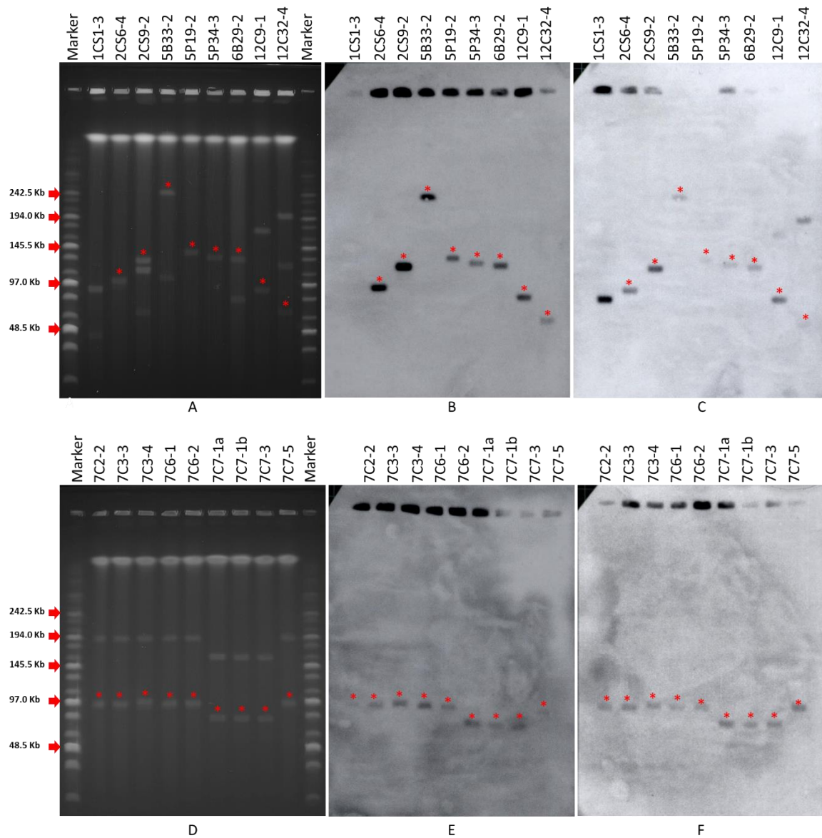
Figure 4. Plasmid profiles of qnr -harboring E. coli . S1-PFGE profiles of isolates with (A) qnrS1 and (D) qnrB4 stained by Ethidium bromide. Lanes 1 and 11: Midrange marker; Southern blot hybridization with a (B) qnrS1 -specific, (E) qnrB4 -specific and (C and F) IncF repB -specific probes. Lanes 2 – 10: nine and eight selected E. coli harboring qnrS1 and qnrB4 , respectively. (*)- indicate location of qnr determinants in plasmid.
