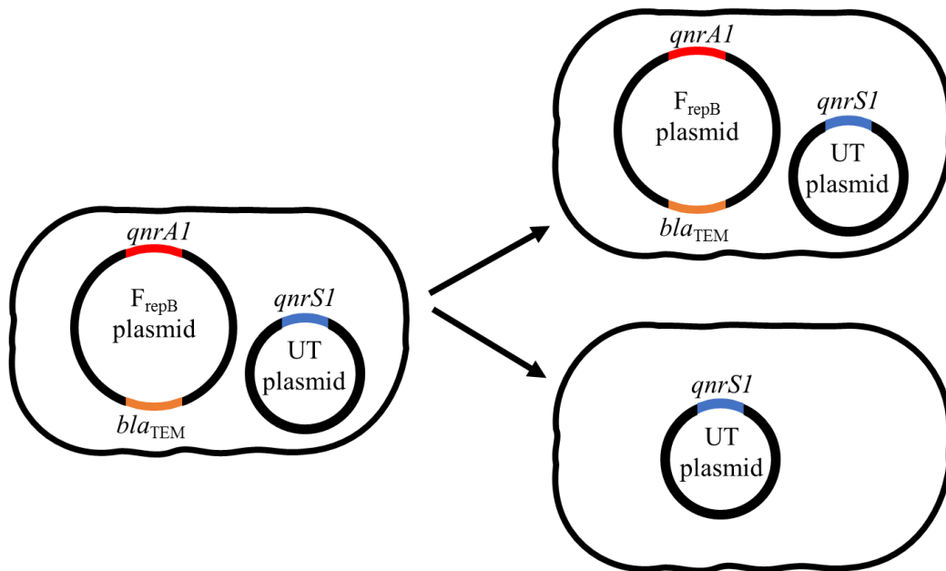
Figure 5. (A) PCR analysis of E. coli harboring both qnrA1 and qnrS1 and its transconjugant. (B) Schematic representation of plasmid segregation of resistant E. coli harboring qnrA1 and qnrS1 . UT – un-typable
