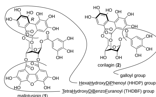
Figure 1. Structures of mallotusinin (1) and corilagin (2).
