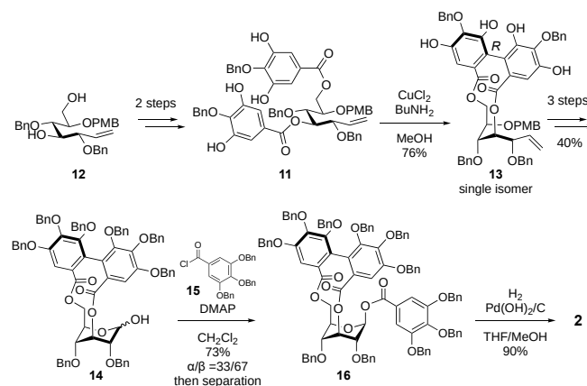
Scheme 2. Previously established route for synthesizing corilagin ( 2 ). Ph = phenyl, Bn = benzyl, PMB = p -methoxybenzyl, Bu = butyl, Me = methyl, DMAP = 4-dimethylaminopyridine, THF = tetrahydrofuran.
