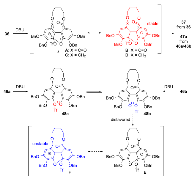
Scheme 6. Proposed mechanism of production of 37/47a from 36/46a/46b .
