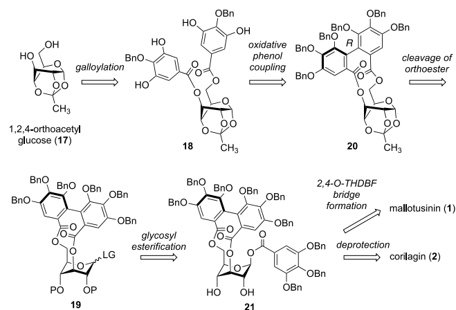
Scheme 3. Synthetic strategy of mallotusin ( 1 ) and corilagin ( 2 ).
