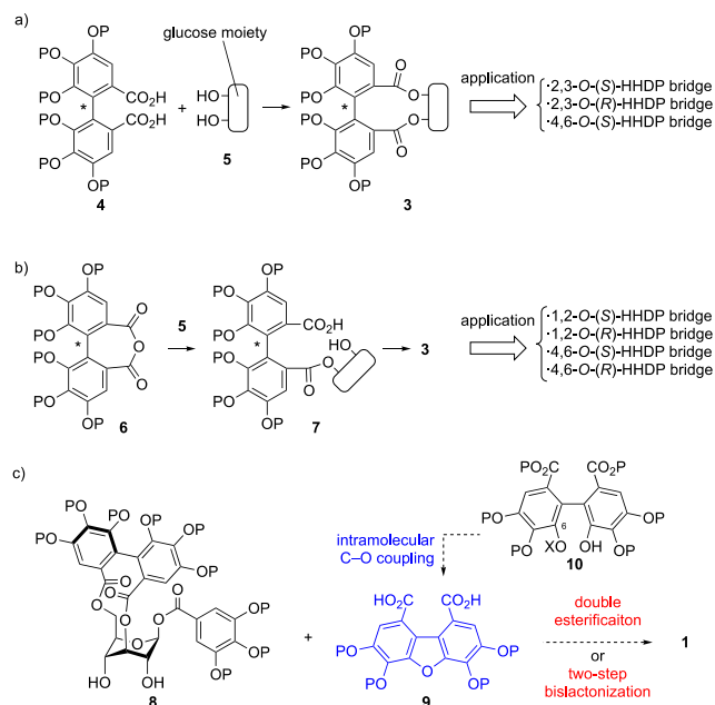
Scheme 1. (a) Double esterification strategy. (b) Two-step bislactonization strategy. (c) Synthetic strategy of the 2,4-O-THDBF bridge of 1 . P = protecting group. X = trifluoromethanesulfonyl (Tf) or its analog.
