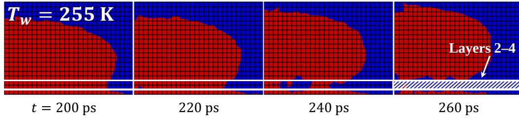
Fig. 4. Evaporating and separating position of droplet.
