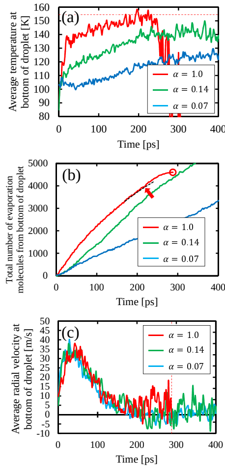
Fig. 15. Time evolutions of (a) average temperature at bottom of droplet, (b) total number of net evaporation molecules from bottom of droplet, and (c) average radial velocity at T_w = 213 K. Dashed line in (a) represents critical temperature of argon. Circle in (b) and dashed line in (c) represent the time when Leidenfrost effect occurred.
