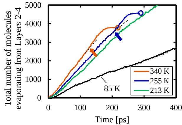
Fig. 11. Time evolutions of total number of net evaporating molecules ( \alpha = 0.14 ) from Layers 2–4 for each wall temperature. Circles represent the time when Leidenfrost effect occurred. Sharp increases occurred at points indicated by solid arrows for T_w = 255 and 340 K. Dashed lines are approximate curves up to these points.
