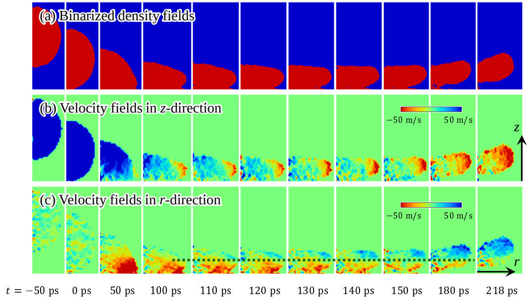
Fig. 6. (a) Binarized density fields of droplet for \alpha = 0.14 at T_w = 340 K. Corresponding velocity fields in (b) z -direction and (c) r -direction. Dotted green line shown in (c) divides droplet into upper and lower parts. Outward velocity occurred at lower part and inward velocity occurred at upper part.
