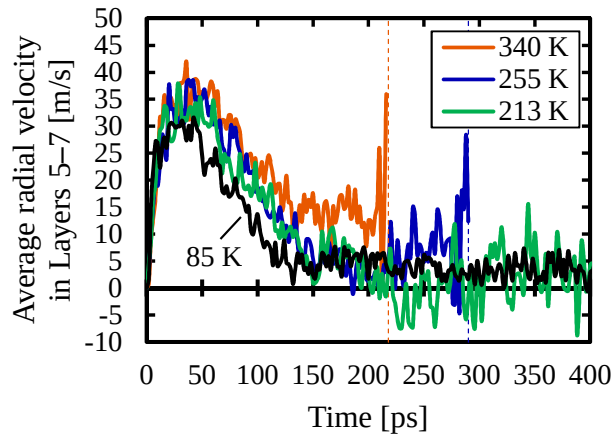
Fig. 13. Time evolutions of average radial flow in Layers 5–7. Dashed lines represent the time when Leidenfrost effect occurred. Significant increases occurred before Leidenfrost effect occurred.
