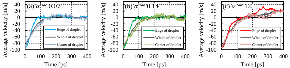
Fig. 16. Time evolutions of average velocity of edge, whole, and center of droplet at T_w = 213 K for (a) \alpha = 0.07 , (b) \alpha = 0.14 , and (c) \alpha = 1.0 . Circle in (c) represents the time when Leidenfrost effect occurred.
