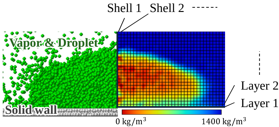
Fig. 2. Parts of simulation domain (left side) and calculated density field (right side). Layer 1 and shell 1 are set at bottom and innermost of control volumes, respectively.
