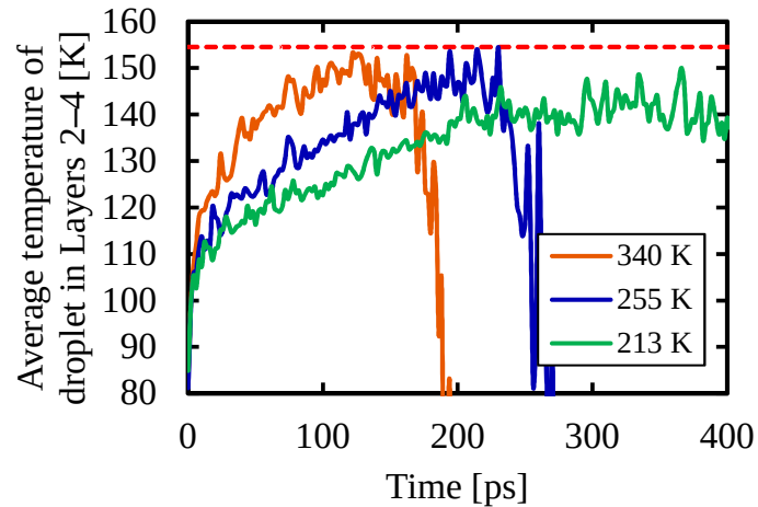
Fig. 9. Time evolutions of average temperature of droplet in Layers 2–4 for \alpha = 0.14 . Dashed red line represents critical temperature of argon ( T_c = 154.5 \text{ K} ).
