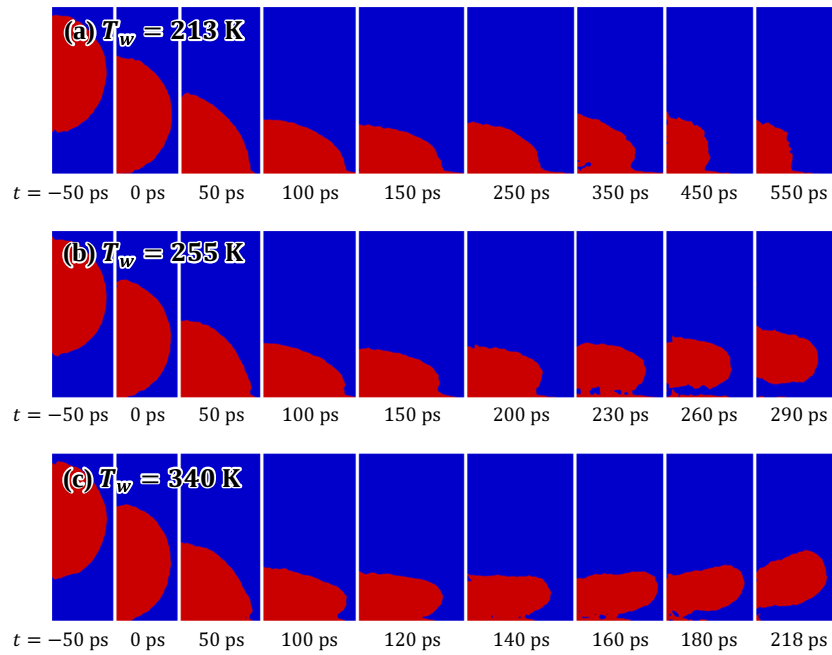
Fig. 3. Binarized density field of impacting droplet on heated wall for \alpha = 0.14 at (a) T_w = 213 K, (b) T_w = 255 K, and (c) T_w = 340 K.
