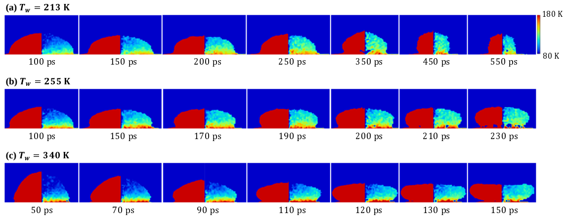
Fig. 8. Binarized density fields (left side) and corresponding temperature fields (right side) for \alpha = 0.14 at T_w = (a) 213, (b) 255, and (c) 340 K.
