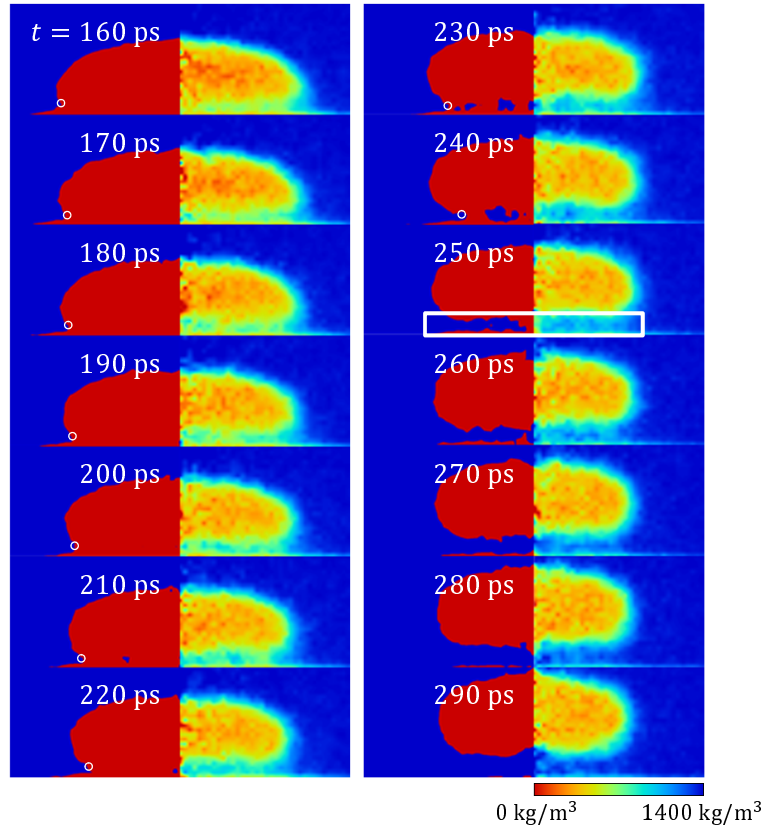
Fig. 12. Binarized density fields (left side) and continuous density field (right side) of impacting droplet at T_w = 255 K for \alpha = 0.14 . Circles on binarized density fields in left column represent intended positions of three-phase contact line (TPCL).
