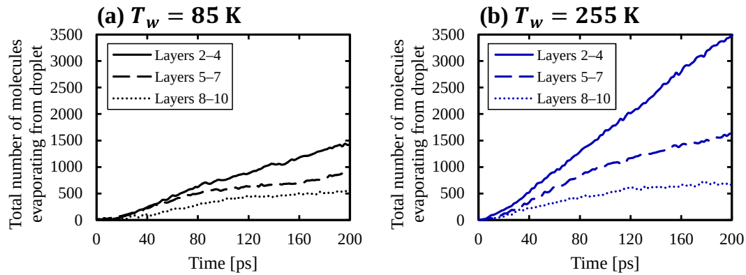
Fig. 10. Time evolutions of total number of net evaporation molecules from each layers for \alpha = 0.14 at (a) T_w = 85 \text{ K} , and (b) T_w = 255 \text{ K} .
