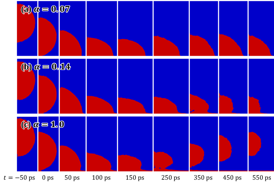
Fig. 14. Binarized density field of impacting droplet on heated wall at T_w = 213 K for (a) \alpha = 0.07 , (b) \alpha = 0.14 , and (c) \alpha = 1.0 .
