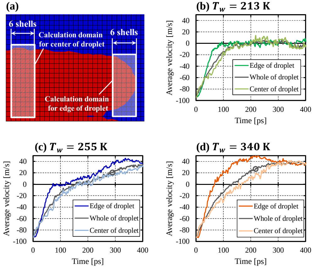
Fig. 5. (a) Schematic of calculation domains for average velocities in z -direction of edge and center of droplet. Time evolutions of average velocity of edge, whole, and center of droplet for \alpha = 0.14 at (b) T_w = 213 K, (c) T_w = 255 K, and (d) T_w = 340 K. Circles in (c) and (d) represent the time Leidenfrost effect occurred.
