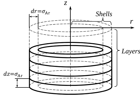
Fig. 1. Control volumes of this MD simulation. There are 63 layers and 63 shells.
