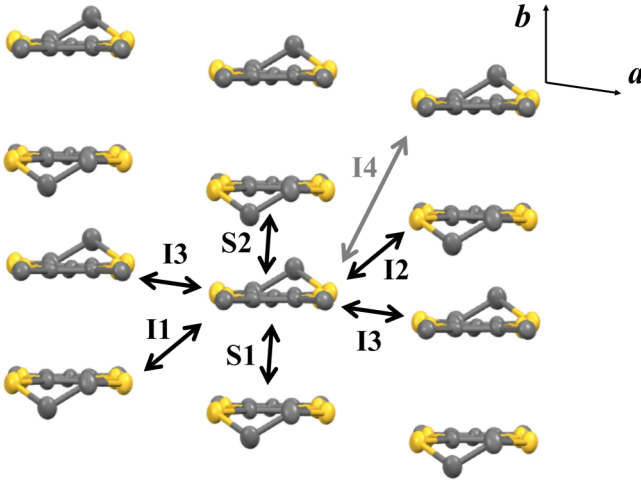
FIG. 2. Definition of the symbols for the overlap integrals of (DMET-TTF) 2 AuBr 2 .
