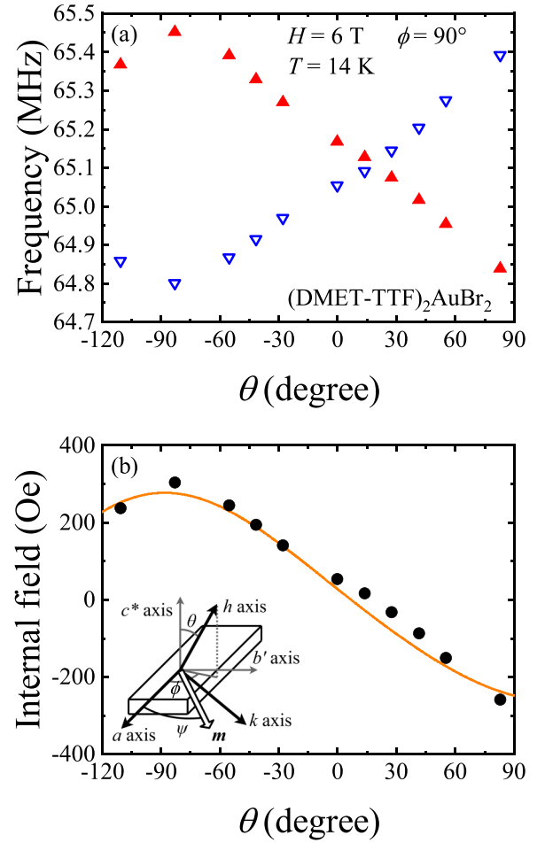
FIG. 10. (a) Field angle dependence of NMR shift at 14 K in (DMET-TTF) 2 AuBr 2 . The open and solid triangles correspond to the up and down spins. (b) Angular dependence of an internal field at 14 K in (DMET-TTF) 2 AuBr 2 . The solid curve is the fitting curve with parameters of m = 0.061 \mu_B/\text{molecule} and \psi = 2^\circ . Inset: Sample and ( a , b' , c^* ) and ( a , k , h ) axis measurement configuration.
