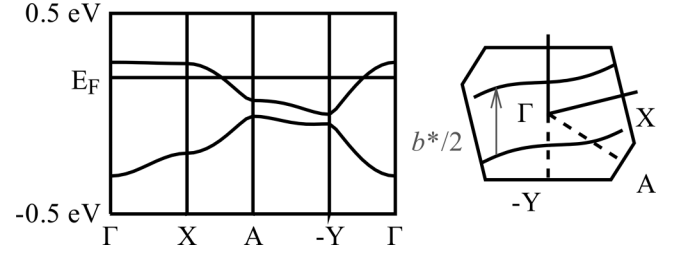
FIG. 3. Band dispersion and Fermi surface of (DMET-TTF) 2 AuBr 2 . b^* is a reciprocal lattice vector.
