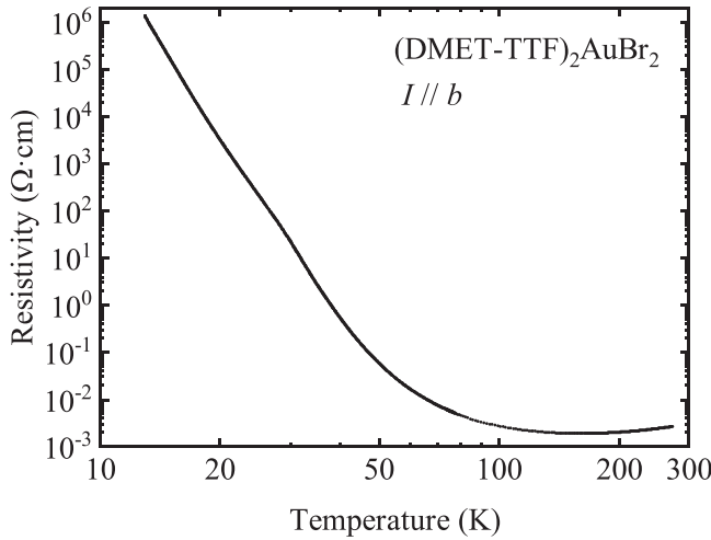
FIG. 4. Temperature dependence of the resistivity in (\text{DMET-TTF})_2\text{AuBr}_2 . The current flows parallel to the b axis.
