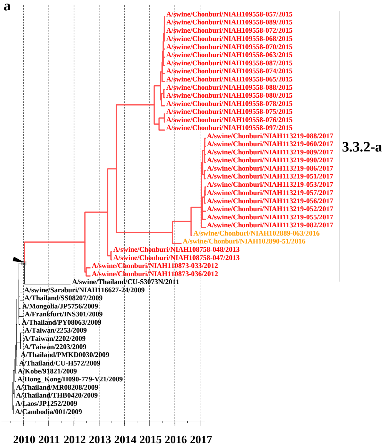
Fig. 12. Detail trees from the entire H1 HA MCC tree made of the genes of viruses isolated in this study and downloaded from the GISAID databases. Genetic groups 3.3.2a, 3.3.2b, and 3.3.2c are shown in lines colored with light red (a), pink (b), and blue (c), respectively, in each panel. Strain names of isolates from farms B, C, and D are shown in red, orange, and blue, respectively. The gray box in each tree indicates the divergence time estimated by using BEAST.
