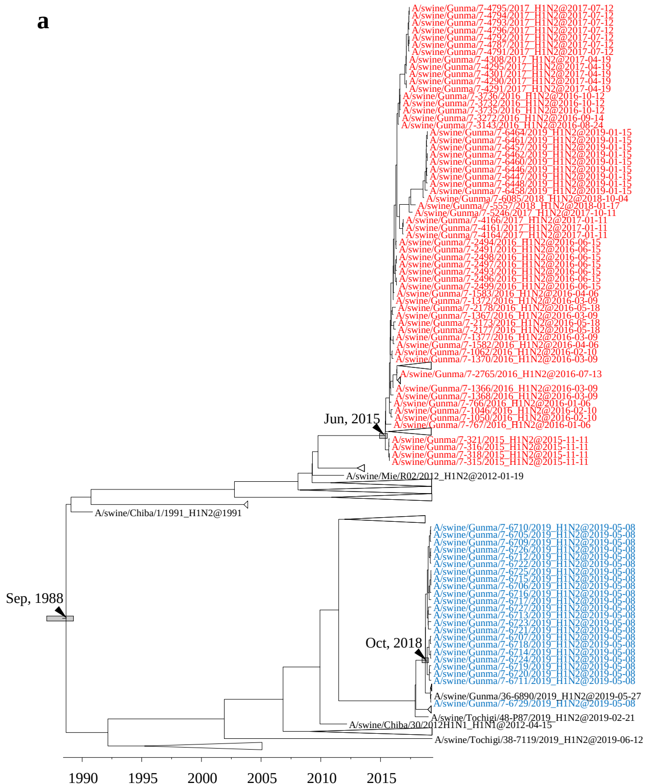
Fig. 7. Detail of MCC trees of H1 HA genes in the 1A.1 classical swine lineage (a) and 1A.3.3.2 A(H1N1)pdm09 lineage (b) (farm 007). Colored text indicates H1N1 and H1N2 IAVs-S isolated at farm 007.
