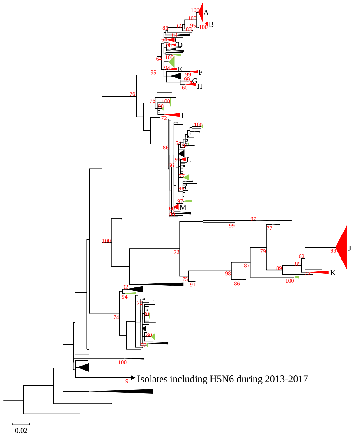
Fig. 25. Entire N6 NA ML tree composed of genes of viruses analyzed in this study and downloaded from the GISAID databases.
