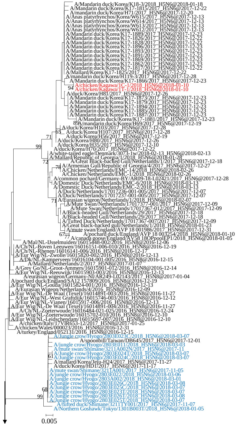
Fig. 18. Details of ML trees based on the H5 HA (a) and N6 NA (b) genes.
