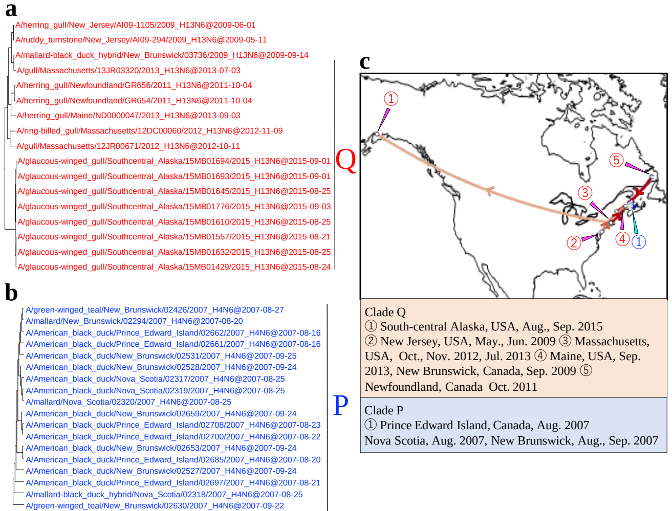
Fig. 30. Detail of MCC trees of N6 NA genes in clades Q and P and visualized location-annotated MCC trees for selected clades on the world map.
