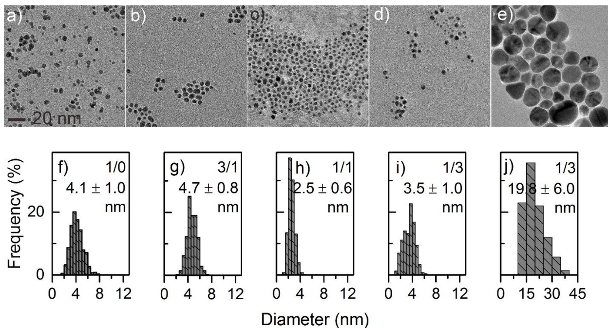
Figure S3. (a-e) TEM images and (f-j) size distributions of sputtered Au nanoparticles dispersed in OA/OAm liquids of (a, f) 1/0, (b, g) 3/1, (c, h) 1/1, and (d, i) 1/3 (v/v) after 15 days of storage. (e) and (j) are big Au nanoparticles in the sample Au OA/OAm 1/3.
