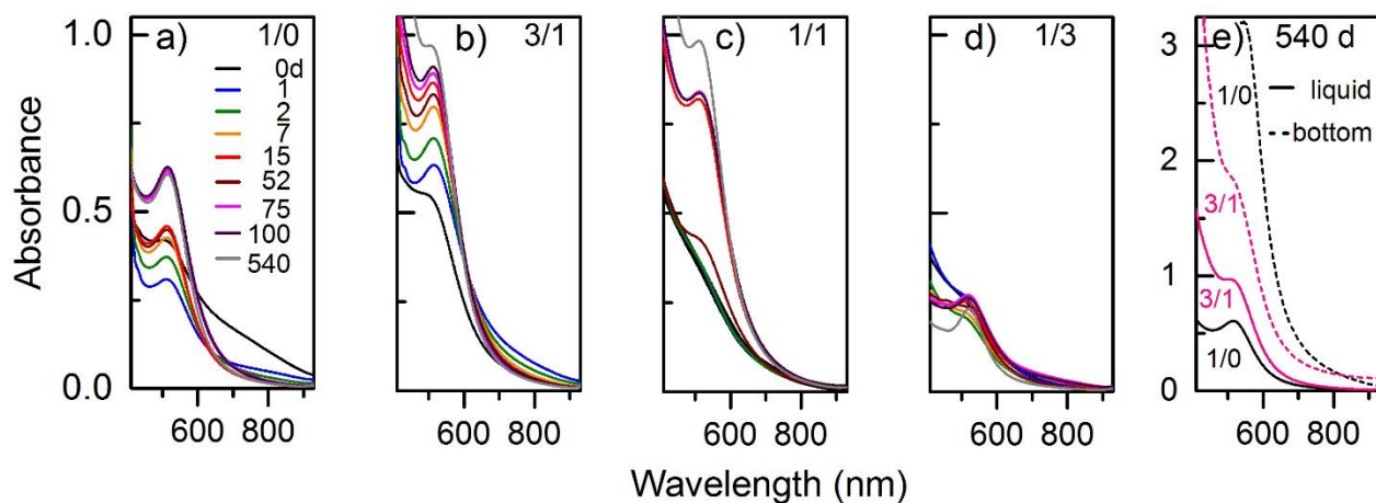
Figure S8. (a-d) UV-Vis spectra of Au OA/OAm during storage. Gradual decrease of absorbance at long wavelength during storage of the dispersion can be observed in accordance with an increase in LSPR peak in Au OA/OAm 1/0 and 3/1. (e) Comparison of the UV-Vis absorption of the bottom liquid and the bulk liquid after storage for 540 days.
