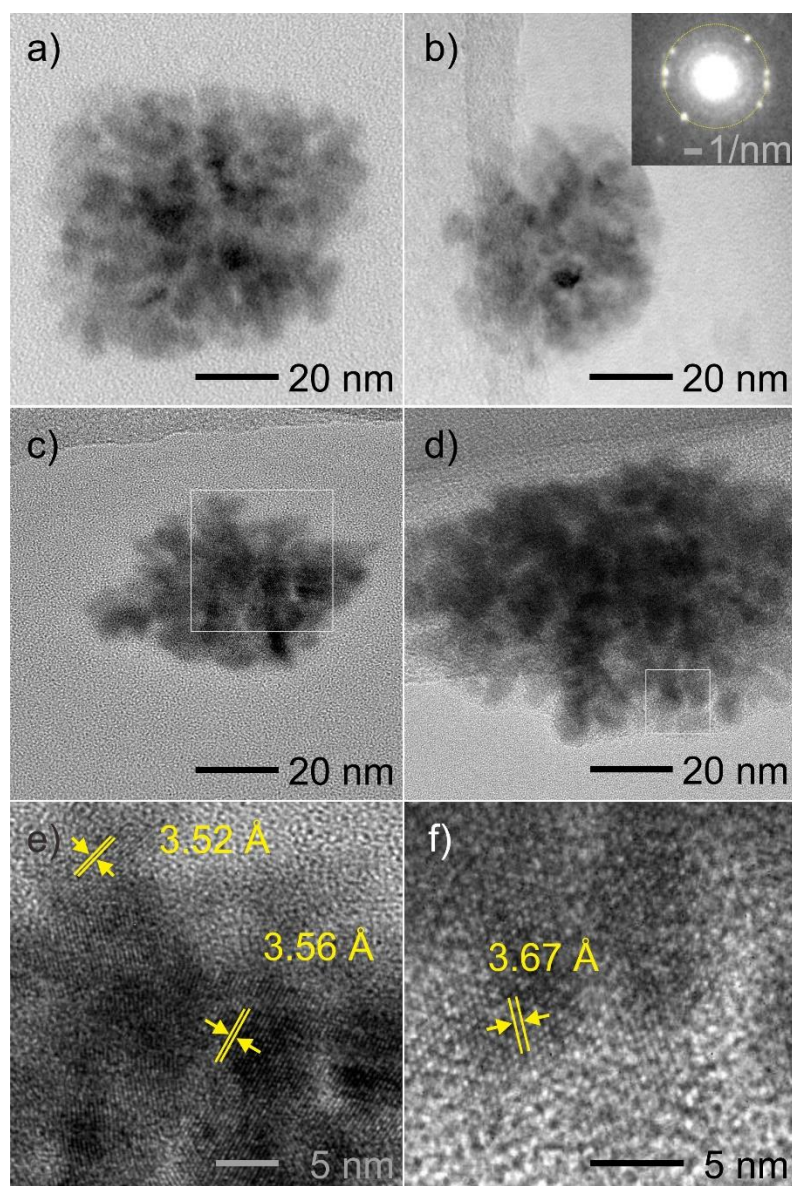
Figure S12. (a,b) TEM images of Cu OA/OAm 1/0 (v/v). Inset of (b) is the SAED pattern of the particles in (b). (c-f) HR-TEM images of Cu OA/OAm 1/1 (v/v) wherein (e) and (f) is the magnified images of the parts marked with white squares in (c) and (d), respectively. The diffraction spots in the inset of (b) line in the ring corresponds to d-spacing of 1.74~1.79 Å, which can be found in various oxides of Cu, e.g., CuO (112) planes, Cu 2 O (211) planes, Cu 4 O (312) planes, and Cu 64 O with (119), (254), (038), and (440) planes. The lattice spacing of 3.52 and 3.56 Å (e) belongs to (030) and (220) planes, respectively, in Cu 64 O, and that of 3.67 Å (f) can be assigned for (014) planes in Cu 64 O.
