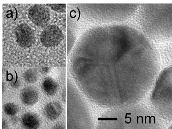
Figure S10. HR-TEM images of (a) Au OA/OAm 3/1, (b) Au OA/OAm 1/3 nanoparticles with small size, single crystal structure and (c) big size with multiple twin planes. All samples are after 15 days of storage.
