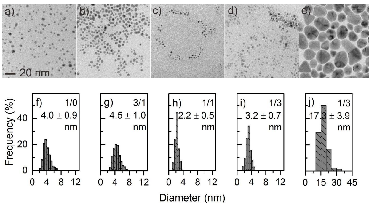
Figure S2. (a-e) TEM images and (f-j) size distributions of sputtered Au nanoparticles dispersed in OA/OAm liquids of (a, f) 1/0, (b, g) 3/1, (c, h) 1/1, and (d, i) 1/3 (v/v) after 7 days of storage. (e) and (j) are big Au nanoparticles in the sample Au OA/OAm 1/3.
