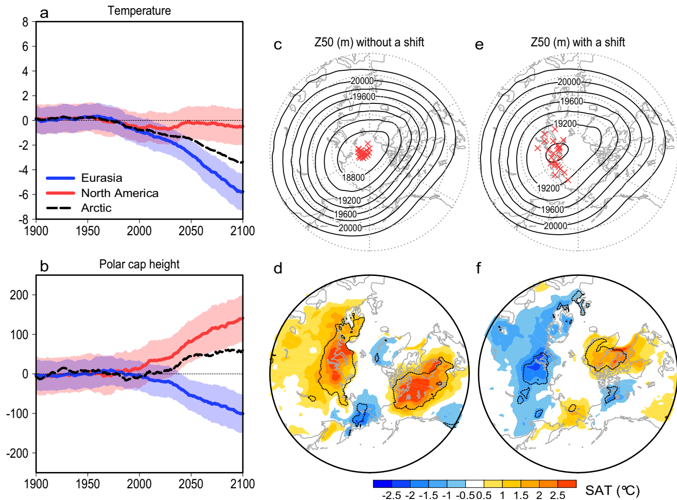
Figure 4. Time series of 50–10 hPa mean (a) temperature (°C) and (b) polar cap height (m) anomalies over Eurasia (100°–150°E, 60°–70°N; blue line), North America (60°–110°W, 60°–70°N; red line), and the Arctic (poleward of 60°N; black dashed line) from 1900 to 2100, relative to the 1901–2000 mean. All the lines and shadings indicate the multi-model mean and \pm 2 standard error (95% confidence range) among the models, respectively, with 21-year running means. Composite mean of 50-hPa geopotential height (m) for the years (c) without and (e) with a polar vortex shift toward Eurasia, based on HIST experiment. Red crosses denote a position of minimum geopotential height. (d and f) As in (c and e), but for composite mean anomalies with 30-year ensemble mean in surface air temperature (°C). Dotted contours indicate statistical significance at the 95% level.
