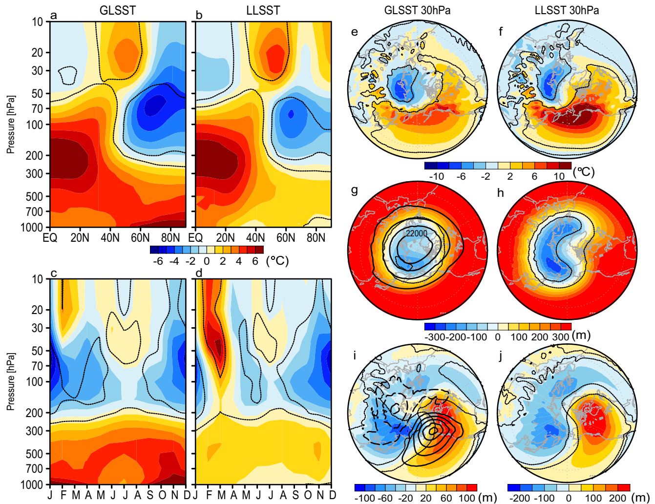
Figure 2. Vertical section of wintertime zonal-mean temperature response in (a) global SST warming and sea ice loss (GLSST) and (b) tropical SST warming (LLSST). (c and d) as in (a and b), but for time-vertical section of the Arctic temperature response. Response of wintertime temperature at 30 hPa in (e) GLSST and (f) LLSST. (g–j) as in (e and f), but for (g, h) geopotential height and (i, j) non-zonal component of geopotential height. Dotted contours indicate statistical significance at the 99% level. Thick contours denote the climatology in HIST experiment (contour interval is 500 m in (g), and 100 m with the zero contour omitted in (i); solid for positive and dashed for negative).
