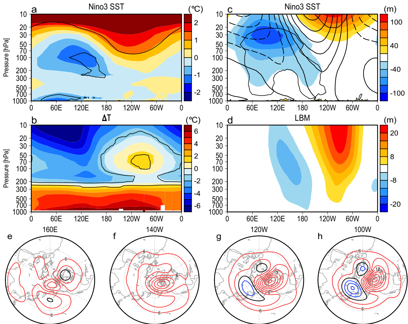
Figure 3. Longitude-vertical section of regressed anomalies of (a) temperature and (c) geopotential height averaged between 60° and 70°N onto standardized Niño-3 SST (5°S–5°N, 90°–150°W) among the individual CMIP5 models in 2070–2099 climatology. (b) As in (a), but for temperature difference between the means over 2070–2099 and 1970–1999. Dotted contours indicate statistical significance over the 95% level in (a and c), and ≥80% model agreement on the sign of the difference in (b). Thick contours in (c) denote the climatological total waves (contour interval is 150 m; solid for positive, dashed for negative, and thick solid for zero). (d) as in (c), but for LBM response to an idealized heating centered over the equator at 100°W. As in (d), but for 30-hPa geopotential height to idealized heating centered over the equator at (e) 160°E, (f) 140°W, (g) 120°W, and (h) 100°W. Contour interval is 3 m; red for positive, blue for negative, and black for the zero contours.
