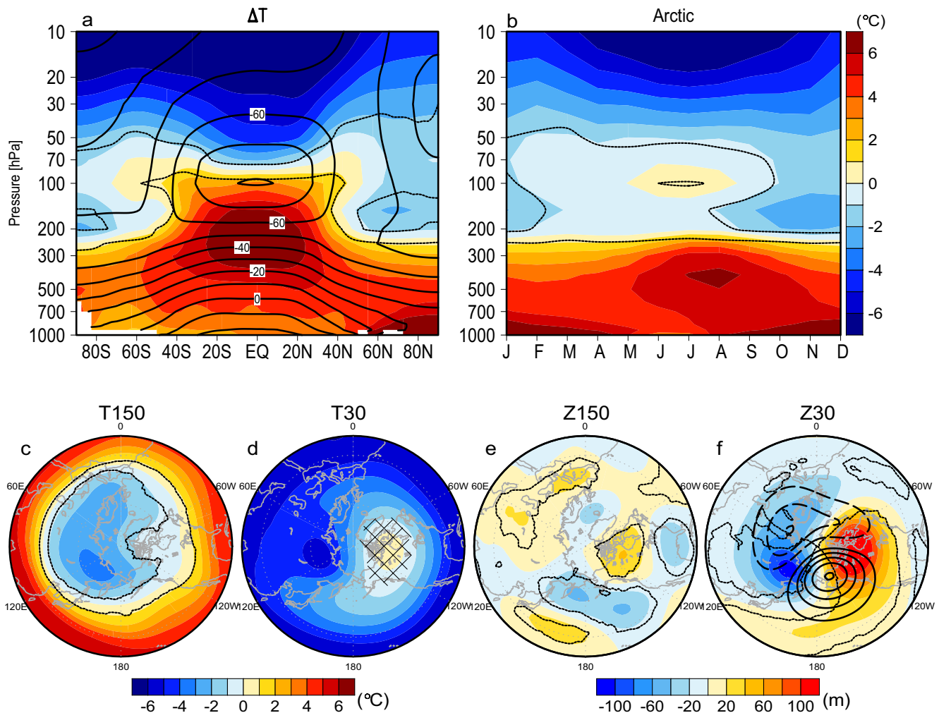
Figure 1. (a) Vertical section of zonal-mean temperature difference between the means over 2070–2099 and 1970–1999 from CMIP5 models in boreal winter (December–February). Solid contours denote the historical temperature climatology (1970–1999). As in (a), but for (b) time-vertical section of the Arctic temperature difference (poleward of 60°N) as a function of calendar month and (c) 150-hPa and (d) 30-hPa temperature differences. (e and f) as in (c and d), but for non-zonal component of geopotential height differences (shaded) and the historical climatology (contour interval is 100 m, with the zero contour omitted; solid for positive and dashed for negative). Dotted contours and hatching indicate \geq 80\% and < 80\% model agreement on the sign of the difference, respectively.
