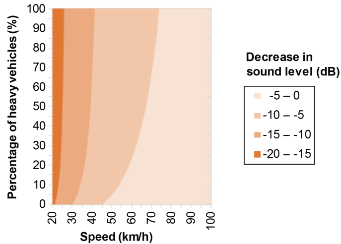
Figure 4.5: Decrease in sound level at different percentages of heavy vehicles and traffic speeds. High sound level reduction is estimated at higher percentages of heavy vehicles and lower traffic speeds.
