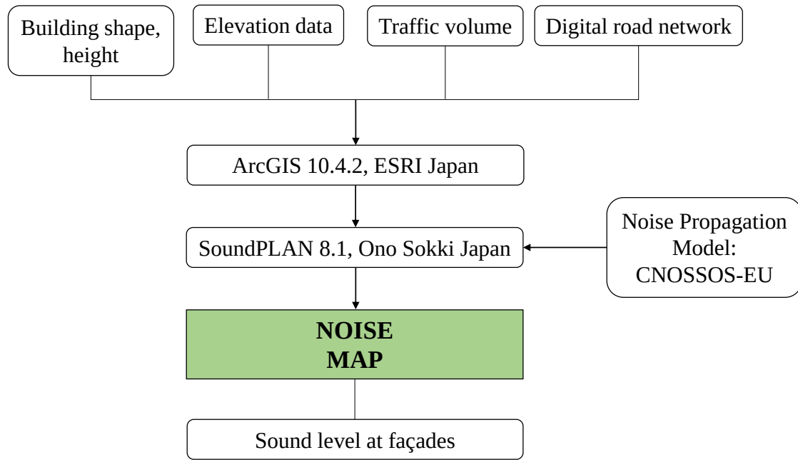
Figure 3.2: Schematic diagram of developing a noise map.
