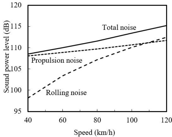
Figure 4.3: An example of sound power level vs vehicle speed. Rolling noise, propulsion noise, and total noise emission of a heavy vehicle were calculated with CNOSSOS-EU at an air temperature of 10°C.
