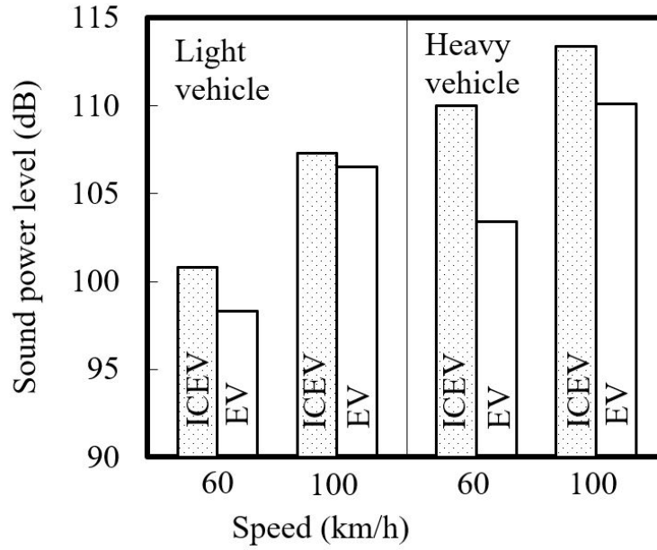
Figure 4.4: Sound power level of a light/heavy ICEV/EV at 60 km/h and 100 km/h with air temperature of 10°C. The sound power level of the EV was calculated by setting the sound power of the propulsion noise to zero.
