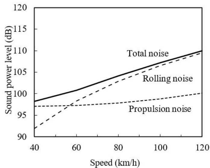
Figure 4.2: An example of sound power level vs vehicle speed. Rolling noise, propulsion noise, and the total noise emission of a light vehicle were calculated with CNOSSOS-EU at an air temperature of 10°C.
