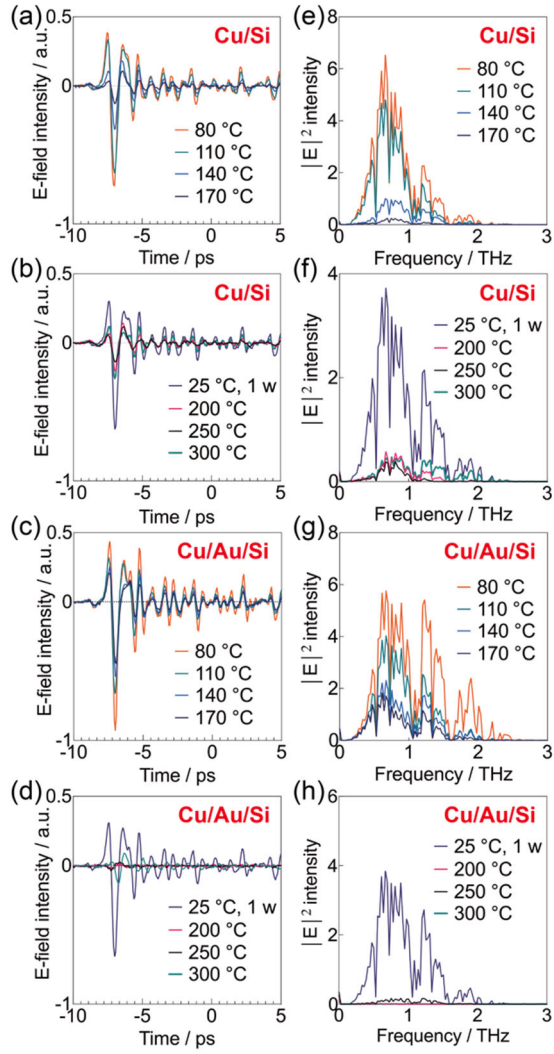
Fig. 3. THz-TDS measurement of the annealed (a-b) Cu/Si and (c-d) Cu/Au/Si structures and (e-h) the corresponding emission spectra at different annealing conditions.
