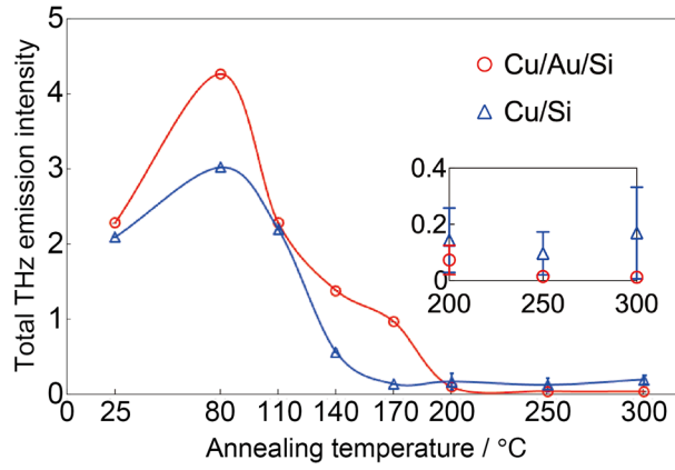
Fig. 4. Total THz wave emission intensity of annealed Cu/Si and Cu/Au/Si structures against different annealing conditions. Solid lines are the guide for the eye.
