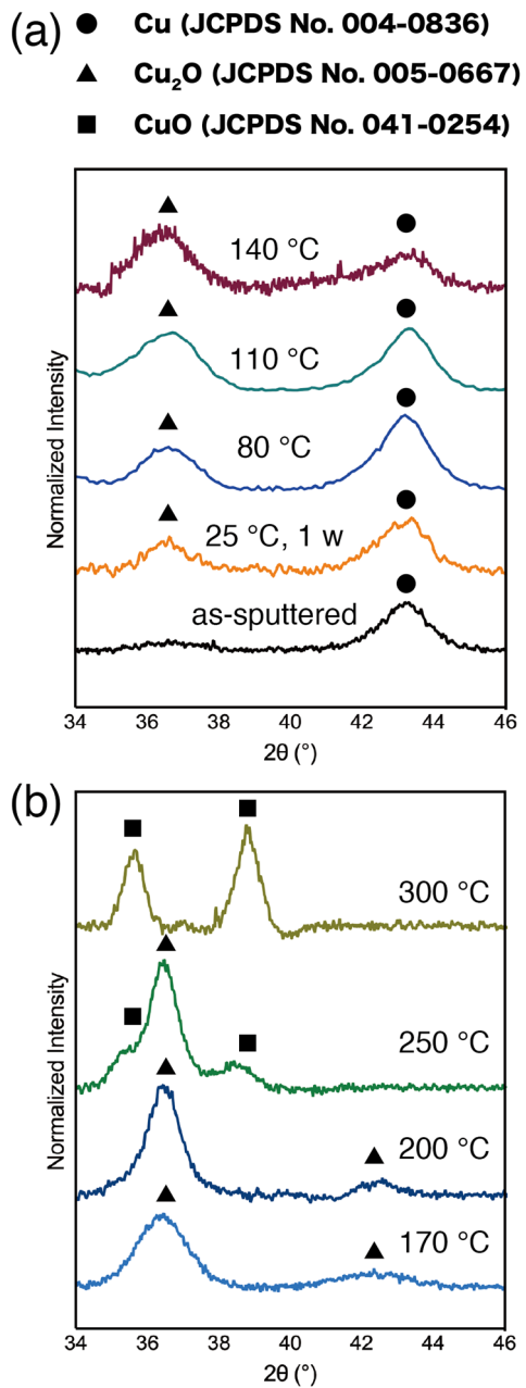
Fig.1. XRD patterns of Cu films at different conditions: (a) as-sputtered, keep in ambient for 1 week, annealed at 80, 110, 140, (b) 170, 200, 250 and 300 °C.
