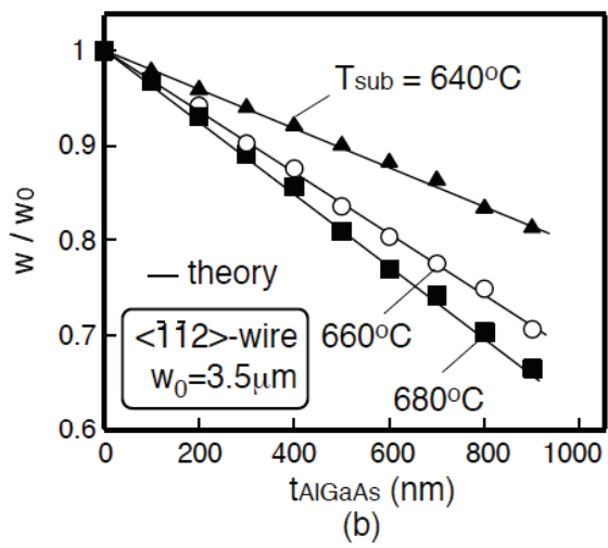
Figure 7: Normalized lateral wire width plotted as a function of the supply thickness of AlGaAs layer for (a) \langle \bar{1}10 \rangle -oriented wires and (b) \langle \bar{1}\bar{1}2 \rangle -oriented wires.
