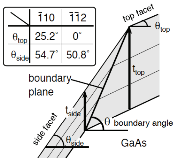
Figure 5: Model for evolution of facet boundary planes.
