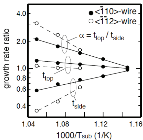
Figure 6: Plots of normalized vertical growth rates vs. substrate temperature.
