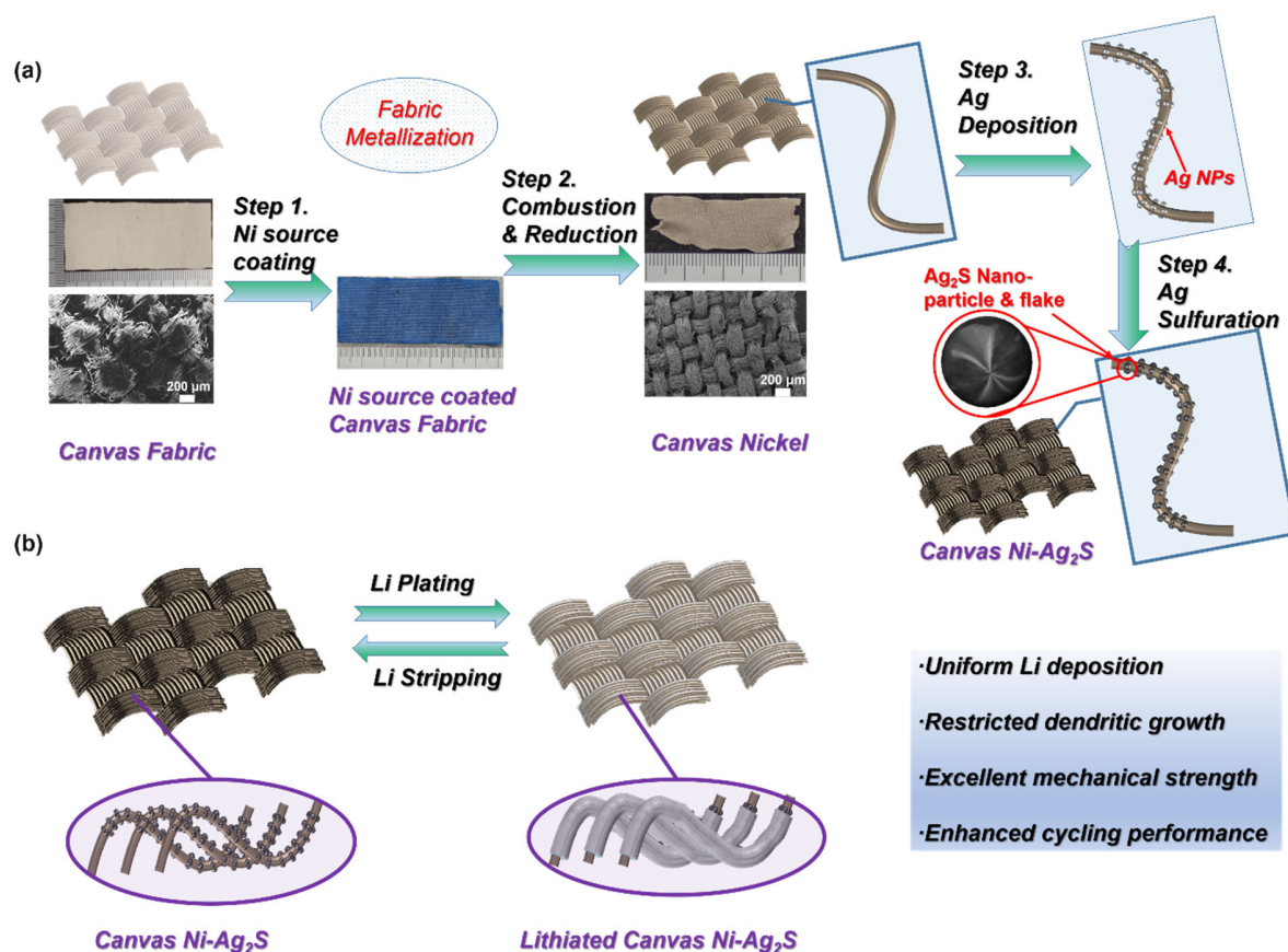
Fig. 1. (a) Scheme of the preparation of Canvas-Ni and Canvas Ni-Ag 2 S frameworks. Optical photos of the fabric template and the Canvas Ni are included. (b) Graphical representation of the uniform electrodeposition behavior of Li on the Canvas Ni-Ag 2 S electrode during plating and stripping.
