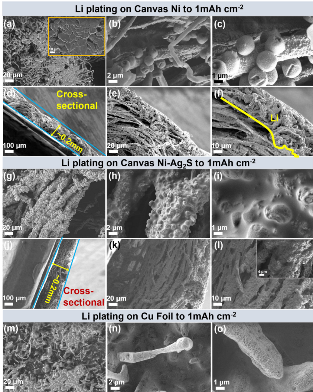
Fig. 3. SEM images of the Li electrodeposition behavior on different electrodes. a-c) Top view and d-f) cross-sectional observation for the Canvas Ni after Li plating to a restricted capacity of 1
