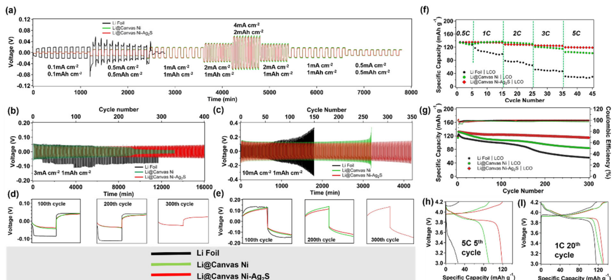
Fig. 4. Electrochemical cycle performance of different electrodes containing Li metal. a, b, c) Voltage profiles of bare Li foil symmetric cells (black), Li@Canvas Ni symmetric cells (green) and Li@Canvas Ni-Ag 2 S symmetric cells (red) a) at different current densities with different capacities; b) at 3 mA cm -2 with a capacity of 1 mA h cm -2 and c) at 10 mA cm -2 with a capacity of 1 mA h cm -2 ; d) shows the zoomed-in voltage profiles at different cycles correspond to (b); e) shows the zoomed-in voltage profiles at different cycles correspond to (c). f) Rate performance and g) long-term cycle performance of full cells using LCO as cathode. Voltage profiles corresponding to Li Foil | LCO full cell (black), Li@Canvas Ni | LCO full cell (green) and Li@Canvas Ni | Ag 2 S-LCO full cell (red) at h) 5th cycle with the rate of 5 C and i) 20th cycle with the rate of 1 C.
