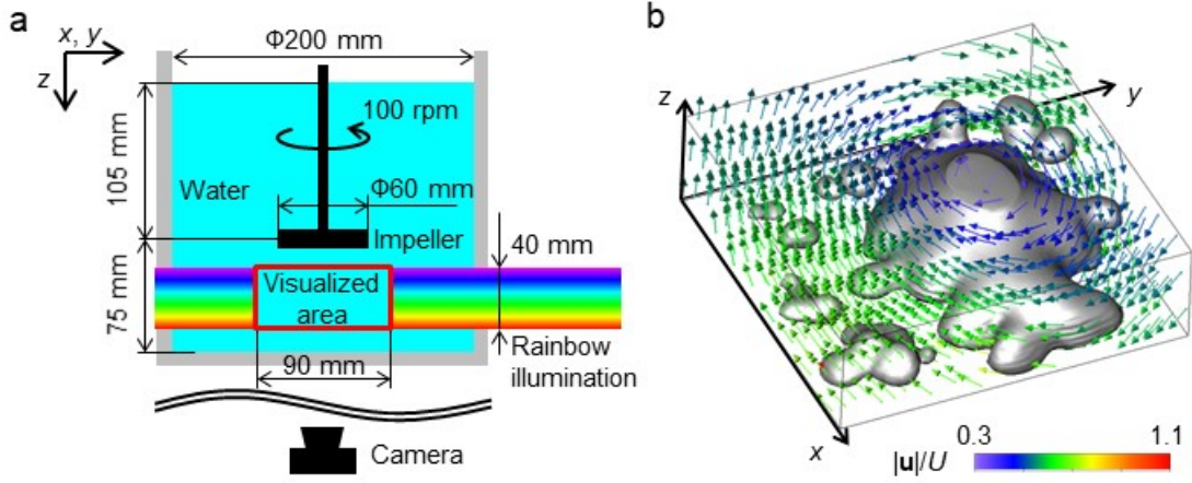
Fig. 4. Demonstration of rainbow volumetric PTV with defocusing technique. (a) Experimental setup. (b) Instantaneous 3D–3C velocity vector field, where the gray surface is the iso-surface indicating |\text{rot}(\mathbf{u}/U)| = 0.1
