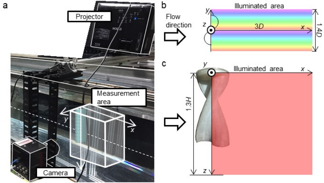
Fig. 15. Twisted Savonius turbine experiments performed in a towing tank. (a) Picture of facility setup. (b) Top and (c) side views of measurement area, where D and H are the diameter and height of the turbine, respectively.
