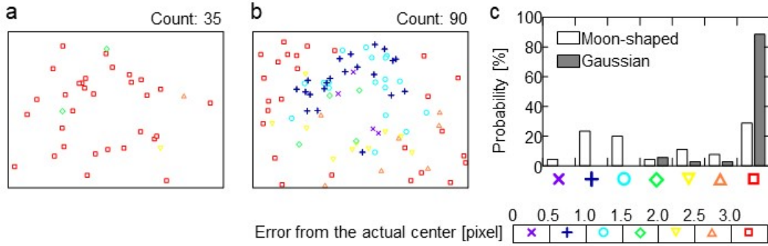
Fig. 10. Comparison of the values calculated by the algorithm to detect particles and their center locations. (a–c) Particles detected using the (a) Gaussian and (b) moon-shaped masks. (c) The probabilities of error based on the actual particle centers.
