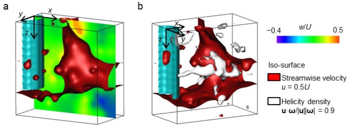
Fig. 17. Sample results. (a) Vertical velocity w interpolated by BER. (b) Visualized streamwise vortex, where \boldsymbol{\omega} is vorticity.
