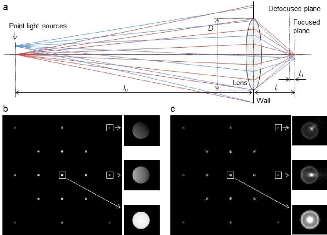
Fig. 5. Particle images distorted by defocusing. (a) Schematic diagram of ray tracing with a convex lens and simulated particle images at the defocused plane. (b) Images without consideration of the aberration caused by the lens. (c) Images with consideration of spherical aberration.
