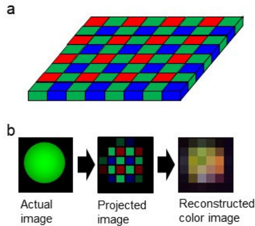
Fig. 1. Cause of false color on the Bayer sensor. (a) RGBG mosaic-type Bayer sensor normally used in a digital camera. (b) Process of false color generation on a particle caused by the Bayer sensor. The color in the reconstructed image is modified to be a different color. This effect is called color contamination.
