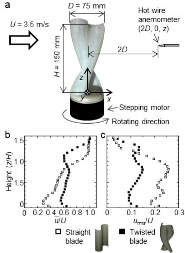
Fig. 14. Effect of the twisted blade of a Savonius turbine on flow in the downstream region, where the tip speed ratio of the turbine is 0.4. (a) Experimental setup, where x - and z -axes are set as the streamwise direction of main flow and the rotating axis of turbine, respectively. (b) Time-averaged streamwise velocity. (c) Turbulence intensity.
