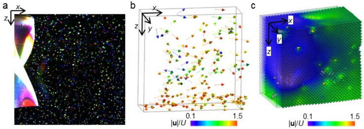
Fig. 16. Processing to obtain 3D-3C instantaneous velocity field. (a) Snap picture of particles illuminated by two-cycle rainbow illumination in the depth direction. (b) Instantaneous velocity vector \mathbf{u}(u, v, w) obtained by the PTV. (c) Interpolated velocity vector field obtained by converting PTV data to a regular grid format using the algorithm proposed by Ido and Murai (2006).
