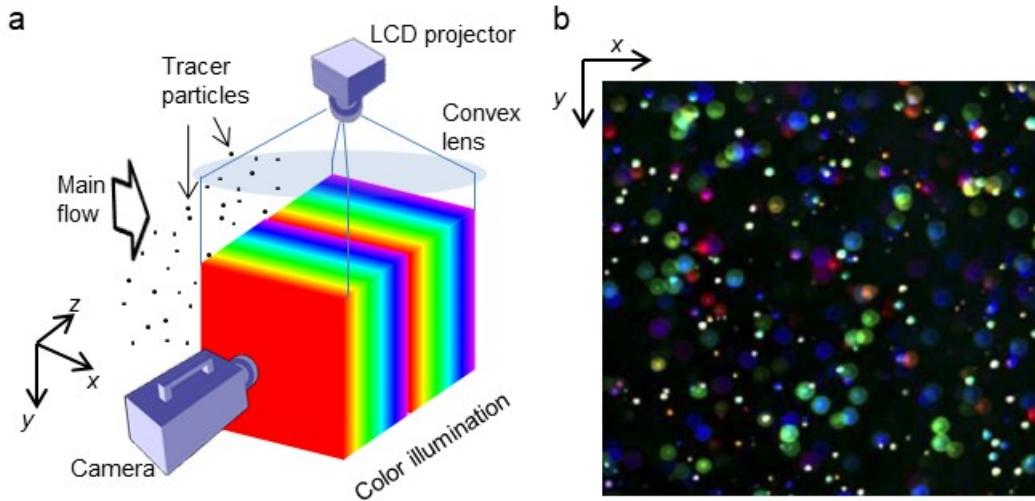
Fig. 12. Two-cycle rainbow color PTV with defocusing technique. (a) Schematic diagram of facility setup, where divergence of light was eliminated by inserting convex lens. (b) Part of a picture obtained from the camera.
