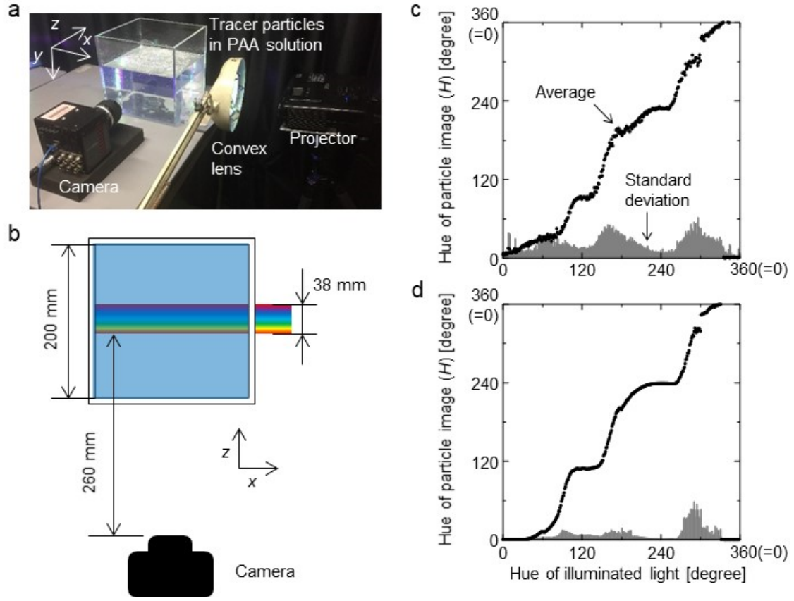
Fig. 3. Improved identification of particle scattering colors achieved by defocusing. (a) Picture and (b) schematic diagram of experimental setup for hue calibration. (c–d) Hue calibration curves with (c) focused images and (d) defocused images, where gray error bars indicate the standard deviation.
