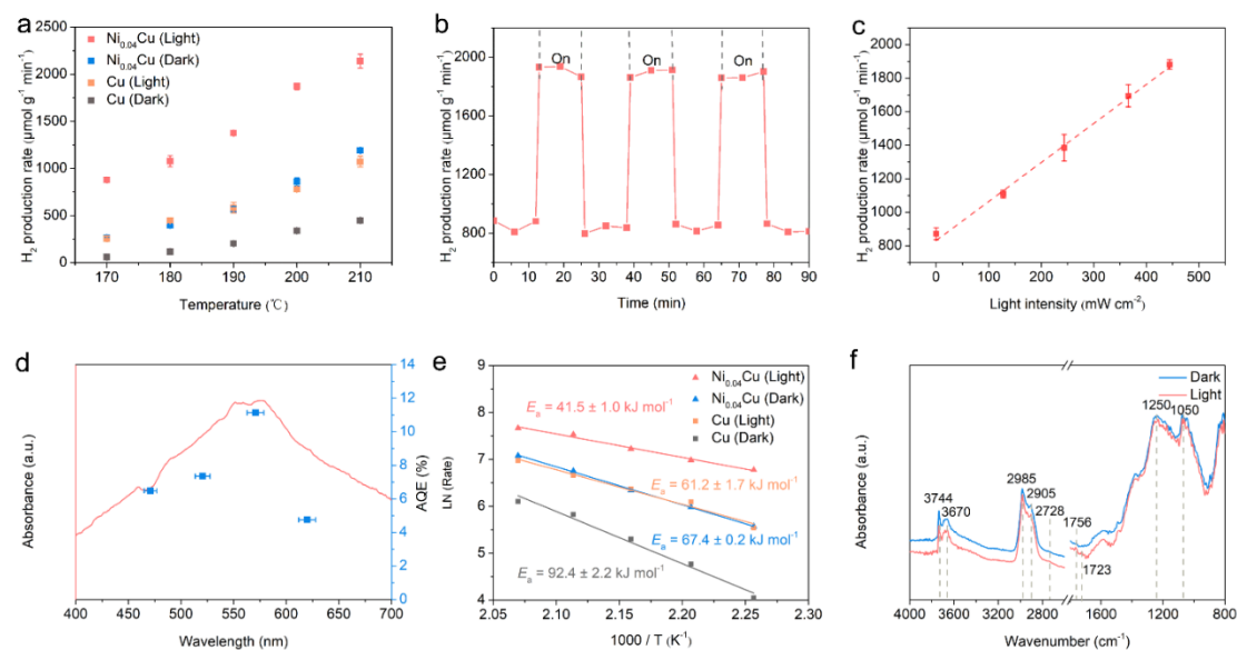
Figure 3. Mechanistic investigation for hot carriers assisted ethanol dehydrogenation reaction. (a) Reaction rate of H_2 production on the Cu and Ni-Cu bimetallic catalysts as a function of temperature under the purely thermal condition (dark) and under photo-assisted thermal condition (light), (b) H_2 production rate on \text{Ni}_{0.04}\text{Cu} catalyst with and without visible light irradiation at 200^{\circ}\text{C} , (c) Dependence of H_2 production rate of \text{Ni}_{0.04}\text{Cu} at 200^{\circ}\text{C} on light intensity, (d) Light absorption and AQE values of \text{Ni}_{0.04}\text{Cu} at 200^{\circ}\text{C} with light irradiation in different wavelength ranges, (e) Arrhenius plots for H_2 production rate under dark and light conditions over pure Cu and \text{Ni}_{0.04}\text{Cu} catalysts, error bars represent the standard deviation of three measurements with the same catalysts, (f) In-situ DRIFT spectra of \text{Ni}_{0.04}\text{Cu} catalysts under dark and light conditions.
