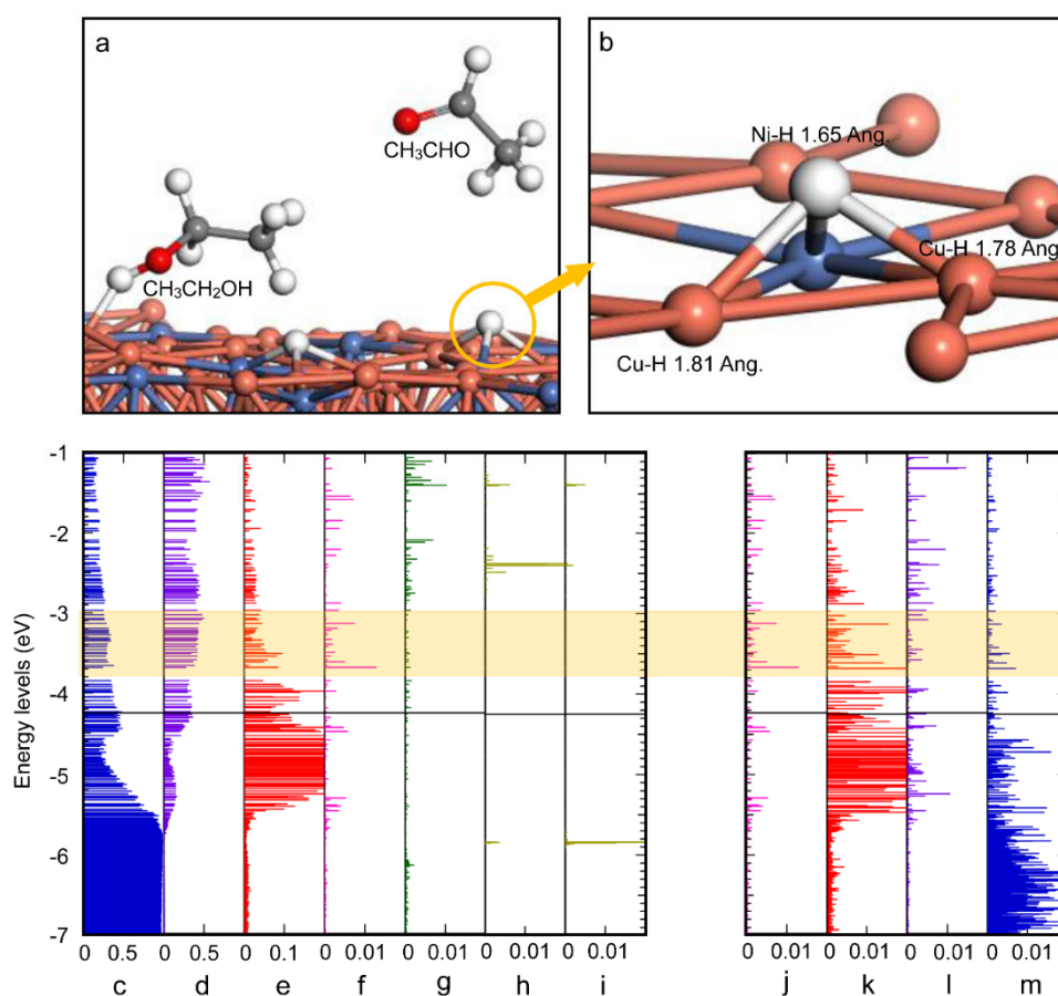
Figure 4. First-principles molecular dynamics simulation of Ni 0.04 Cu in the reaction molecular of CH 3 CH 2 OH and CH 3 CHO. (a) Snapshot of the equilibrium structure at 200 °C of the Cu metal doped with Ni atoms, which is intended to mimic Cu 1-δ Ni δ /SiO 2 systems, in the presence of ethanol and acetaldehyde molecules. The color code is white for H, red for O, gray for C, brown for Cu, and cyan for Ni, (b) Local adsorbate structure
