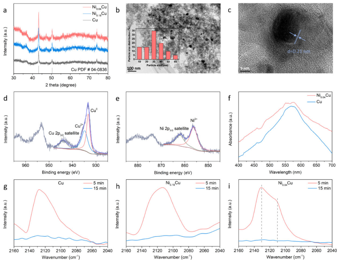
Figure 1. Characterization of Ni-Cu bimetallic catalysts. (a) XRD patterns of pristine Cu and Ni-Cu bimetallic catalysts, (b and c) TEM and HRTEM images of \text{Ni}_{0.04}\text{Cu} catalysts, (d and e) XPS patterns of \text{Ni}_{0.04}\text{Cu} catalysts, (f) UV-Vis DRS patterns of pristine Cu and Ni-Cu bimetallic catalysts, (g) CO-DRIFT spectra of pristine Cu catalysts, (h) CO-DRIFT spectra of \text{Ni}_{0.18}\text{Cu} catalysts, (i) CO-DRIFT spectra of \text{Ni}_{0.04}\text{Cu} catalysts.
