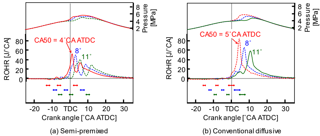
Figure 7. The in-cylinder gas pressure and the rate of heat release (ROHR) for different combustion phases (IMEP \approx 0.4 MPa).
