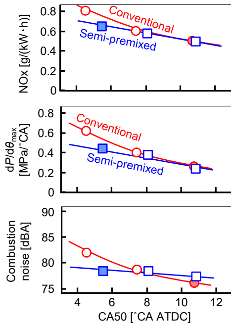
Figure 9. The NOx emissions, the maximum rate of pressure rise, dP/d\theta_{max} , the combustion noise, and the exhaust gas emissions at a low load (1500 rpm, IMEP \approx 0.4 MPa).
