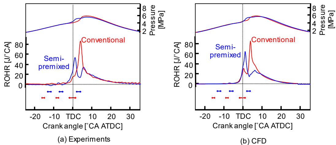
Figure 11. The semi-premixed and the conventional modes for the analysis on mechanism of thermal efficiency improvement with the semi-premixed mode (1500 rpm, IMEP \approx 0.4 MPa).
