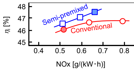
Figure 10. The trade-off relation between the NOx and the indicated thermal efficiency at a low load (1500 rpm, IMEP \approx 0.4 MPa).
