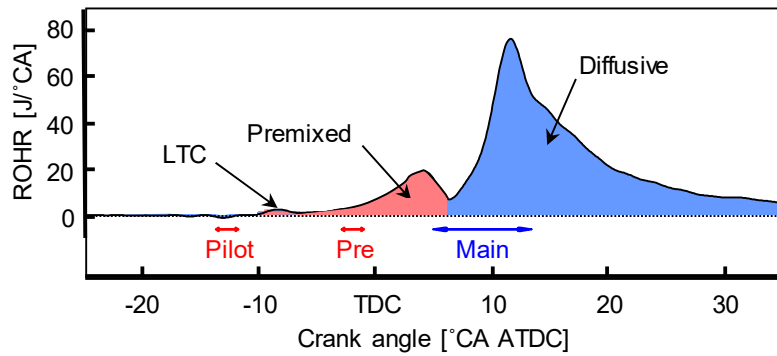
(b) Conventional diffusive diesel combustion mode
