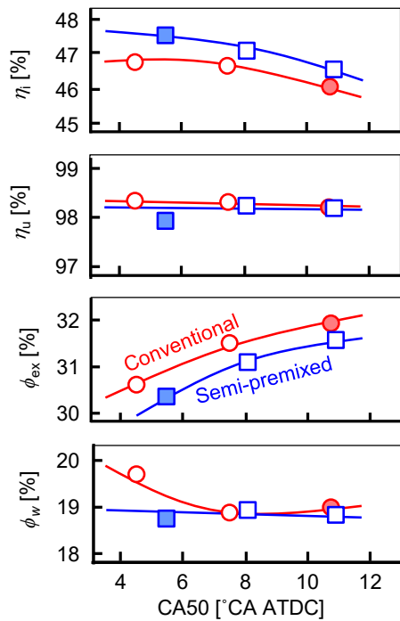
Figure 8. The influence of the combustion phase on the thermal efficiency related parameters (indicated thermal efficiency, \eta_i , combustion efficiency, \eta_u , exhaust loss, \phi_{ex} , and cooling loss, \phi_w ) at a low load (1500 rpm, IMEP \approx 0.4 MPa).
