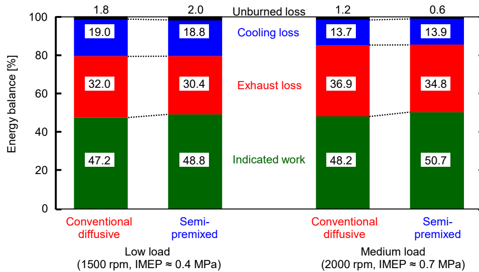
Figure 5. The energy balances at the same conditions as in Figure 4.
