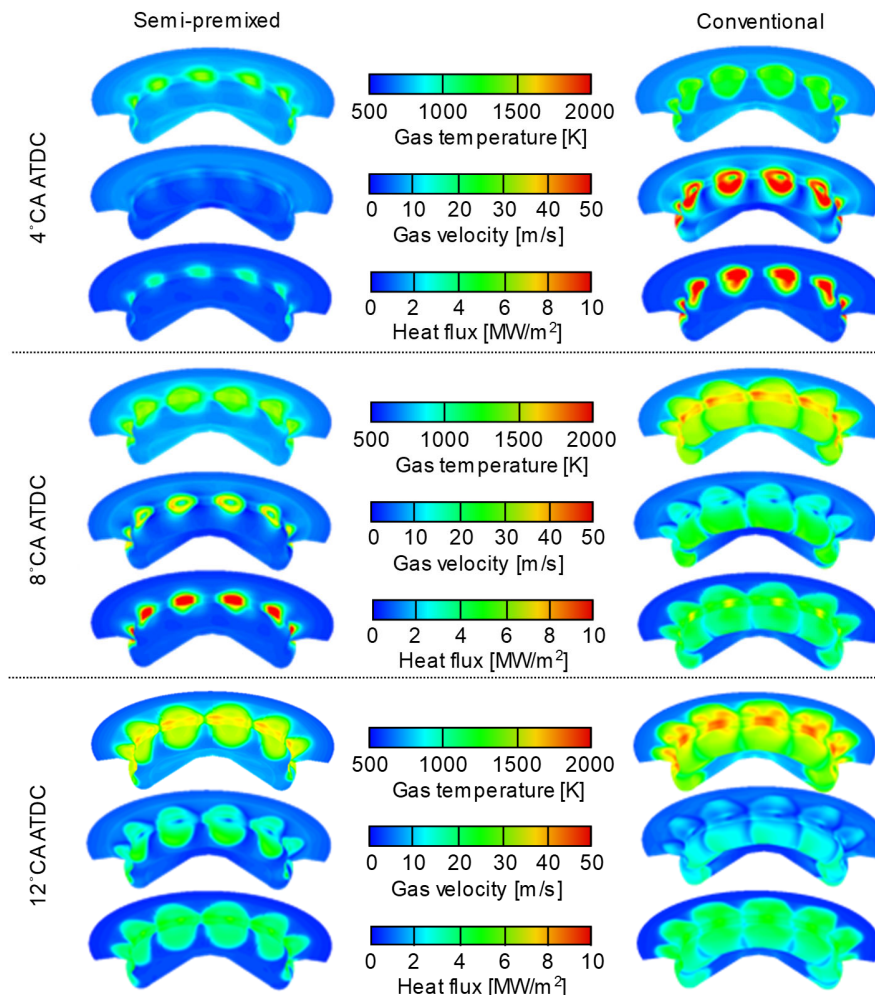
Figure 14. Plots of gas temperature, velocity, and heat flux along the piston top surface (1500 rpm, IMEP \approx 0.4 MPa).
