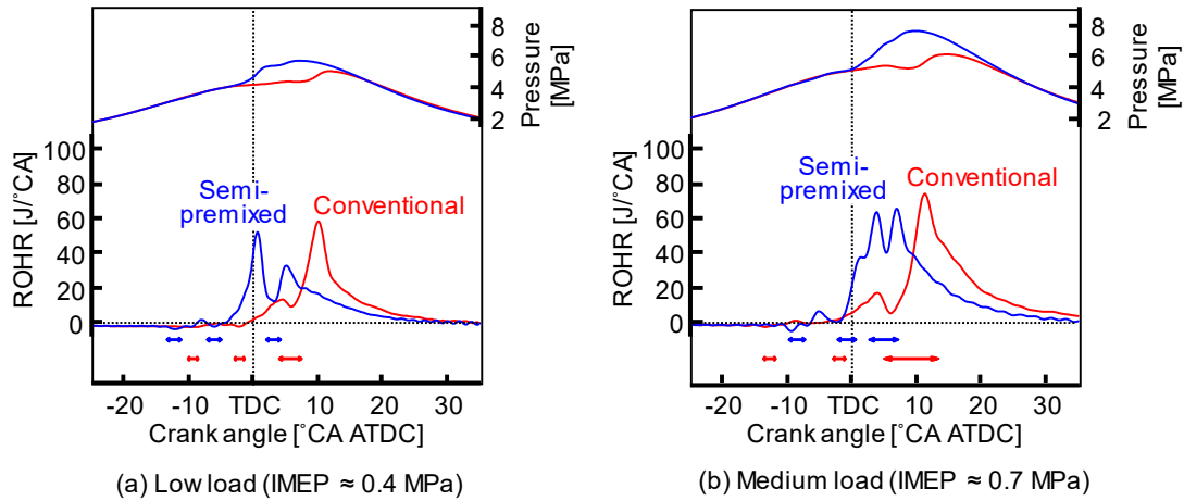
Figure 4. The in-cylinder gas pressure and the rate of heat release (ROHR) from the semi-premixed diesel combustion and the conventional diffusive diesel combustion
