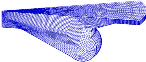
Figure 3. Computational mesh of the stepped-lip re-entrant combustion chamber release.
