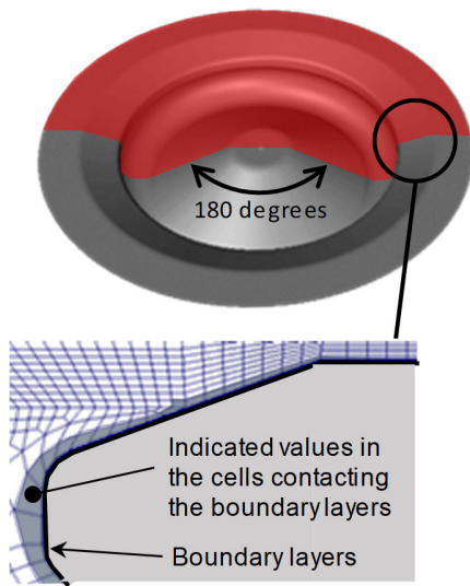
Figure 15. Indicated area of piston surface in Figure14.
