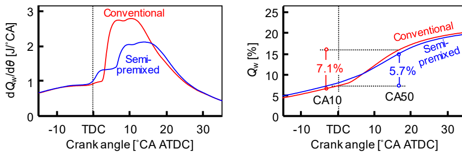
Figure 13. The rate of cooling loss, dQ_w/d\theta and the integrated cooling loss normalized by the total energy supply, Q_w with the calculation (1500 rpm, IMEP \approx 0.4 MPa).
