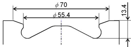
Figure 1. The stepped-lip re-entrant type combustion chamber.
