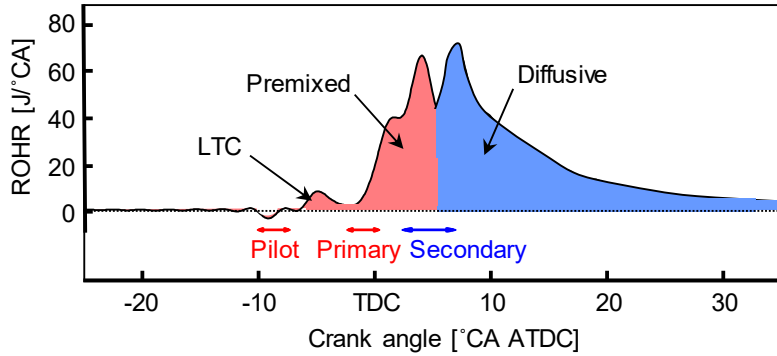
(a) Semi-premixed diesel combustion mode
