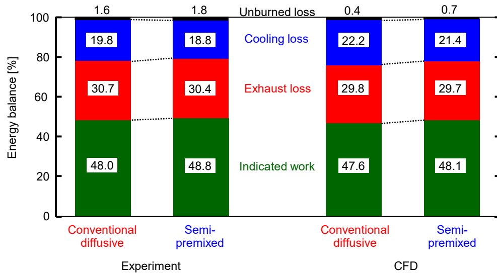
Figure 12. The energy balances at the conditions in Figure 11
