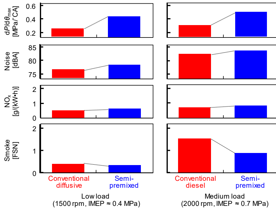
Figure 6. The maximum rate of pressure rise, dP/d\theta_{max} , the combustion noise, the NO x and smoke emissions at the same conditions as in Figure 4.
