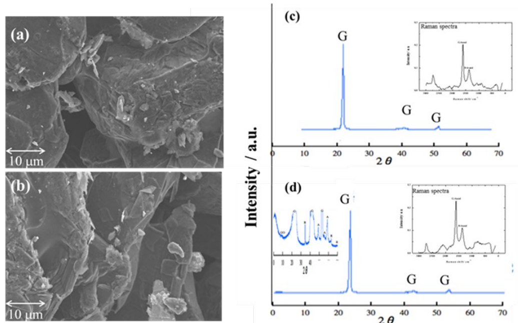
Figure 1. SEM imagines: (a) Porous carbon; (b) TiO 2 doped graphite porous carbon.
