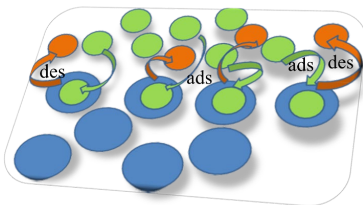
Figure 1.4 The kinetic model of Langmuir of adsorption acknowledges occurring between gas at equilibrium with a surface: adsorption (ads), and desorption (des).
