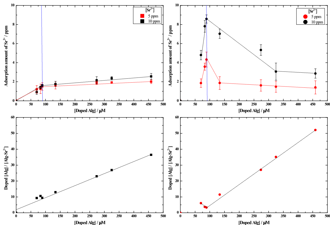
Figure 3. \text{Sr}^{2+} adsorption amount using doped alginate with \text{TiO}_2 doped porous carbon: (a) without potential; (b) with -0.5 V v.s. Ag/AgCl (sat'd KCl) potential charged in 120 min process. Langmuir isotherm of \text{Sr}^{2+} adsorption of alginate doped \text{TiO}_2 doped porous carbon plate ( 1\text{cm} \times 1\text{cm} \times 0.2\text{cm} ): (c) without potential; (d) with -0.5 V v.s. Ag/AgCl charge applied in \text{SrCl}_2 in 120 min process.
