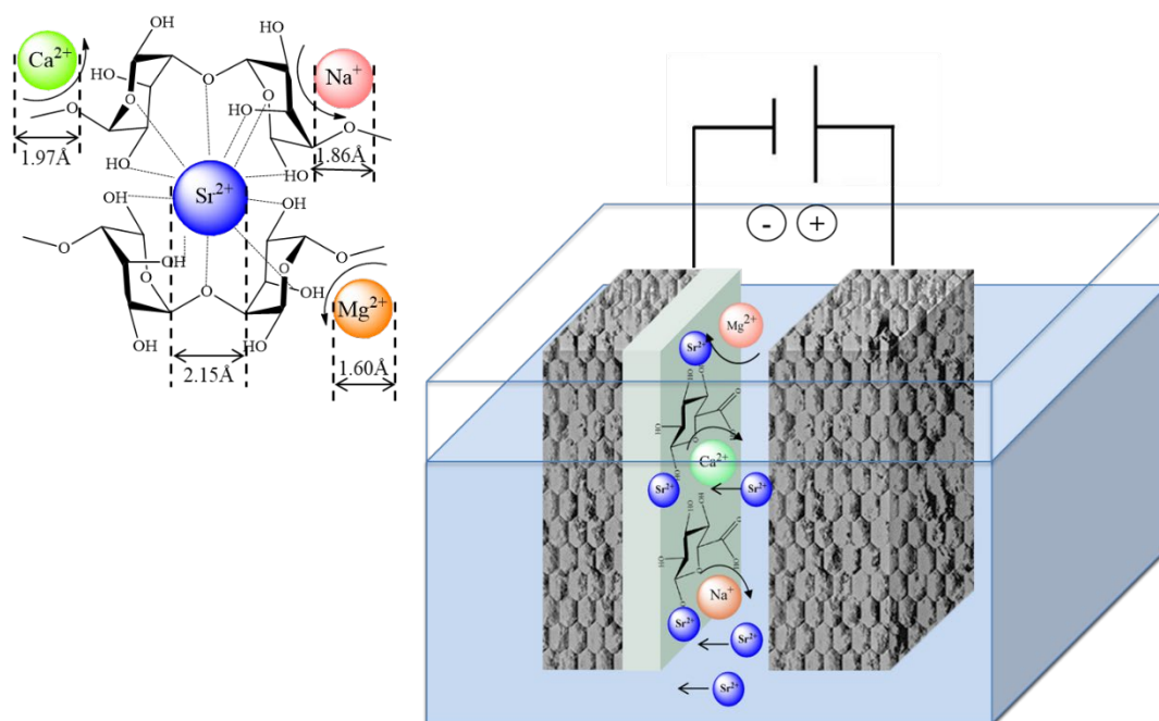
Scheme 1 Electrochemical system of Sr sorption by doped alginate with \text{TiO}_2 doped porous carbon electrode, composite absorbent as working electrode; and \text{TiO}_2 doped porous carbon as counter electrode.
