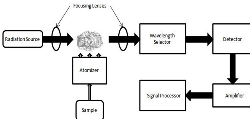
Figure 2.6 The principle of Atomic absorption spectroscopy measurement. [9]
