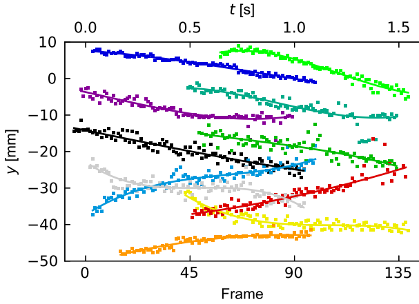
Fig. 10 Particle trajectories with respect to the depth coordinates. Particle positions originally estimated by the ANN are represented by squares, and fitted curves for each particle trajectory are shown as solid lines. The squares and lines are colored uniquely for each particle.
