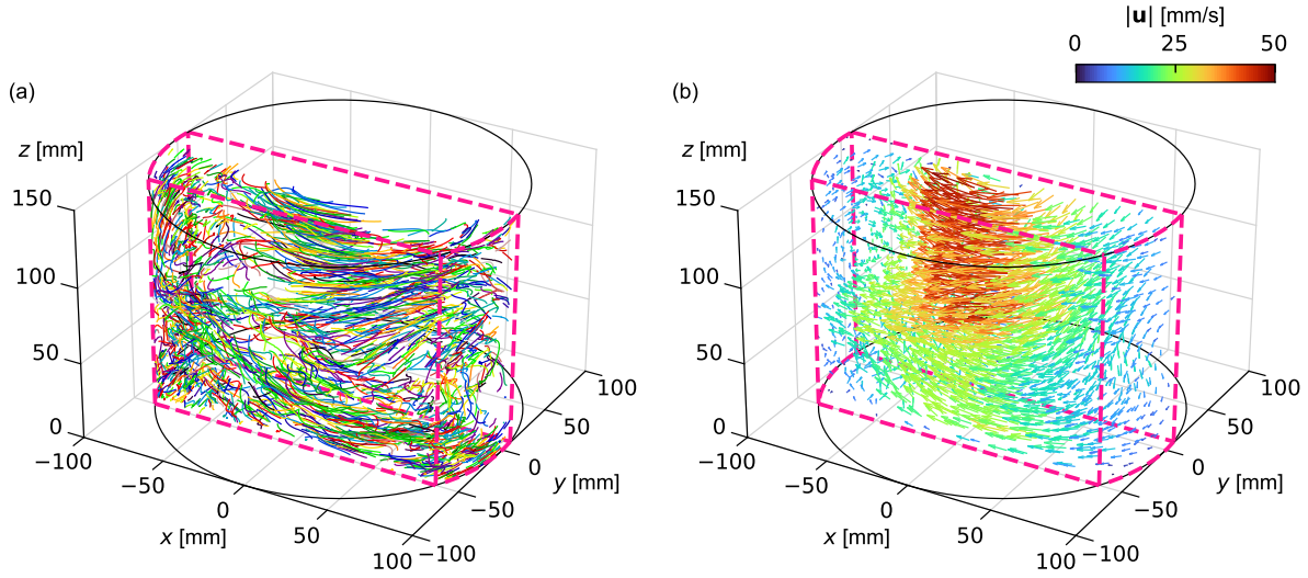
Fig. 12 Reconstructed 3D flow field in a rotating flow induced by an impeller: a 3D particle trajectories of 2,000 particles and b mean velocity field interpolated on a regular grid during 10 s (five cycles of the impeller). The trajectories in a are colored uniquely to identify each particle. The velocity vectors in b are colored by the velocity magnitude |u| , and only 1% of the interpolated vectors are shown for clearer visibility. The measurement volume of the color PTV is enclosed by pink dashed lines.
