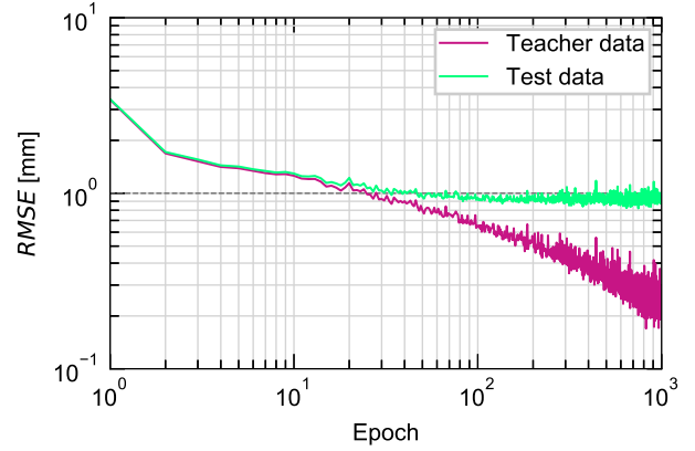
Fig. 8 Training progress of the constructed ANN according to the RMSE values for the training and test data.
