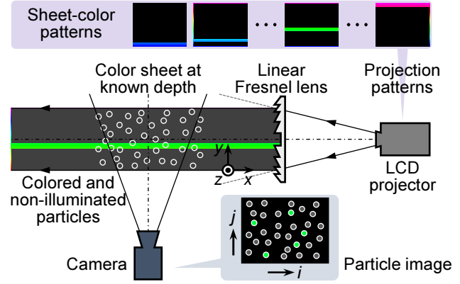
Fig. 6 Sheet-color illumination measurement for color-to-depth calibration.
