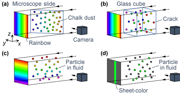
Fig. 2 Calibration methods for the color PTV: a oblique slide (McGregor et al. 2007); b calibration cube (Aguirre-Pablo et al. 2019); c in-plane rainbow (Watanura et al. 2013); and d sheet-color (the present study).
