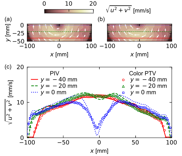
Fig. 14 Mean velocity fields measured by 2D PIV and color PTV at a horizontal cross-section of z = 25 mm: Velocity fields measured by a conventional PIV and b color PTV. c Velocity profiles at fixed horizontal lines of y = -40, -20 , and 0 mm.
