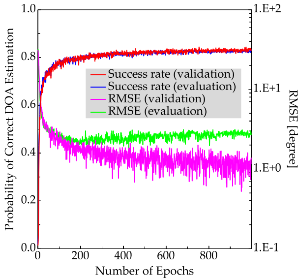
Fig. 4 Transition of estimation success rate and RMSE of DNN A in the training phase. For estimation performance confirmation, success rate and RMSE of DNN A fixed at the abscissa epoch obtained using 100,000 evaluation data are also shown.
