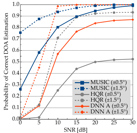
Fig. 5 Success rates of the DNN A, Root MUSIC, and HQR. As a special case, success rates when \pm 1.5^\circ is allowed are also shown.
