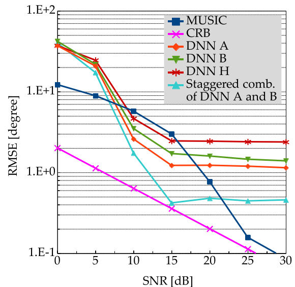
Fig. 10 RMSEs of DNN A, DNN B, staggered combination of DNN A and DNN B, DNN H, Root MUSIC, and CRB.
