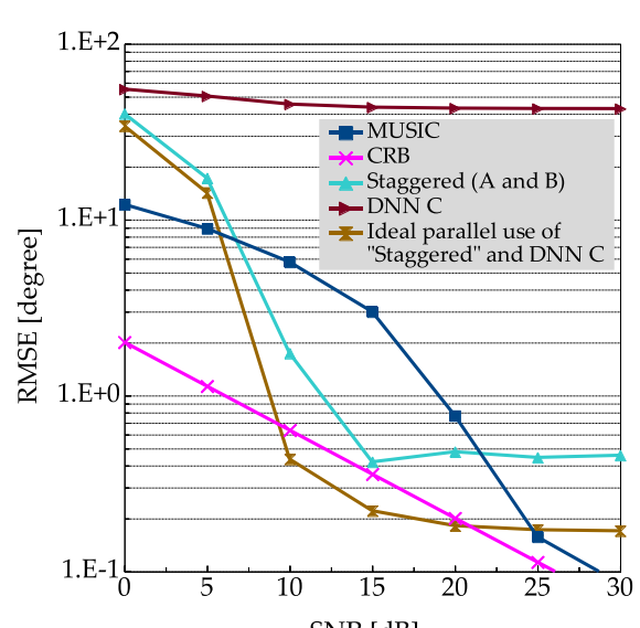
Fig. 15 RMSEs for the case switching the staggered combination of DNN A and DNN B or DNN C ideally.
