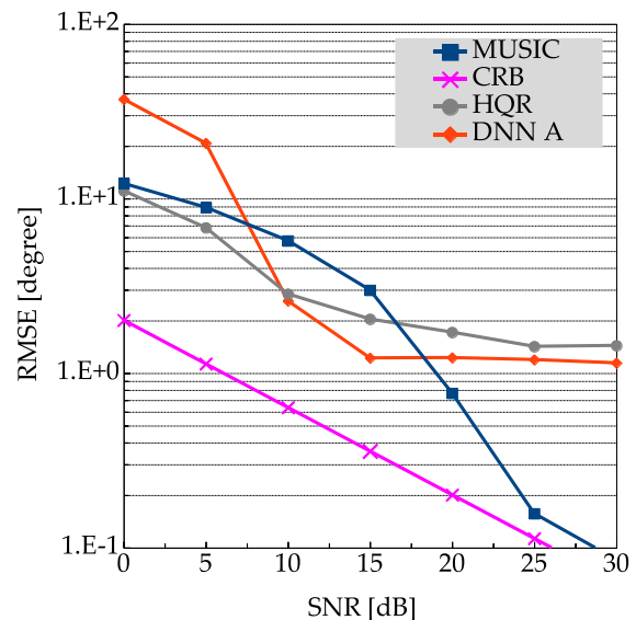
Fig. 6 RMSEs of DNN A, Root MUSIC, HQR, and CRB.
