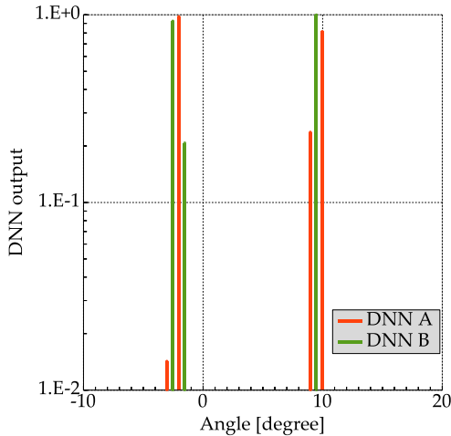
Fig. 11 An example of combined angular spectrum of DNN A and DNN B. True DOAs are -2.21^\circ and 9.49^\circ . Output units: -2^\circ and 9.5^\circ are selected correctly by searching peaks in this spectrum.
