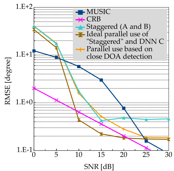
Fig. A·2 RMSEs for the case switching the staggered combination of DNN A and DNN B or DNN C based on close DOA detection.
