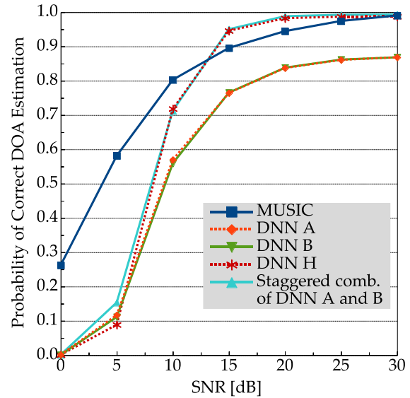
Fig. 9 Success rates of DNN A, DNN B, staggered combination of DNN A and DNN B, DNN H, and Root MUSIC.
