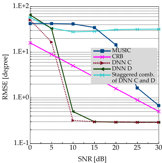
Fig. 13 RMSEs of several types of DNNs, Root MUSIC, and CRB for the case of 1° DOA difference.
