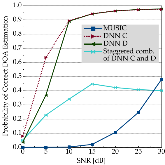
Fig. 12 Success rates of several types of DNNs and Root MUSIC for the case of 1° DOA difference.
