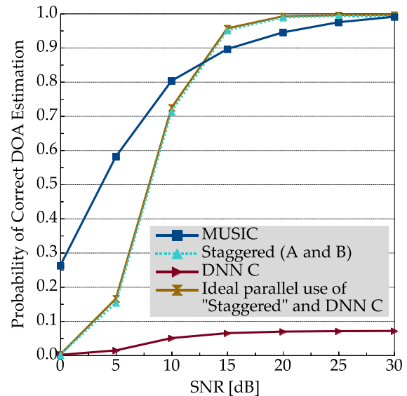
Fig. 14 Success rates for the case switching the staggered combination of DNN A and DNN B or DNN C ideally.
