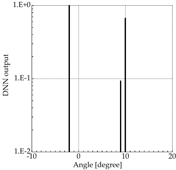
Fig. 7 Output example of DNN A when estimation fails. True DOAs: -2.21^\circ and 9.49^\circ , estimated DOAs: -2^\circ and 10^\circ .
