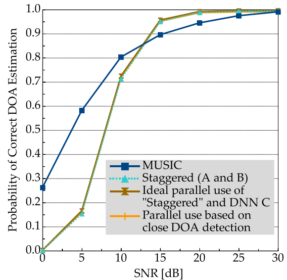
Fig. A·1 Success rates for the case switching the staggered combination of DNN A and DNN B or DNN C based on close DOA detection.
