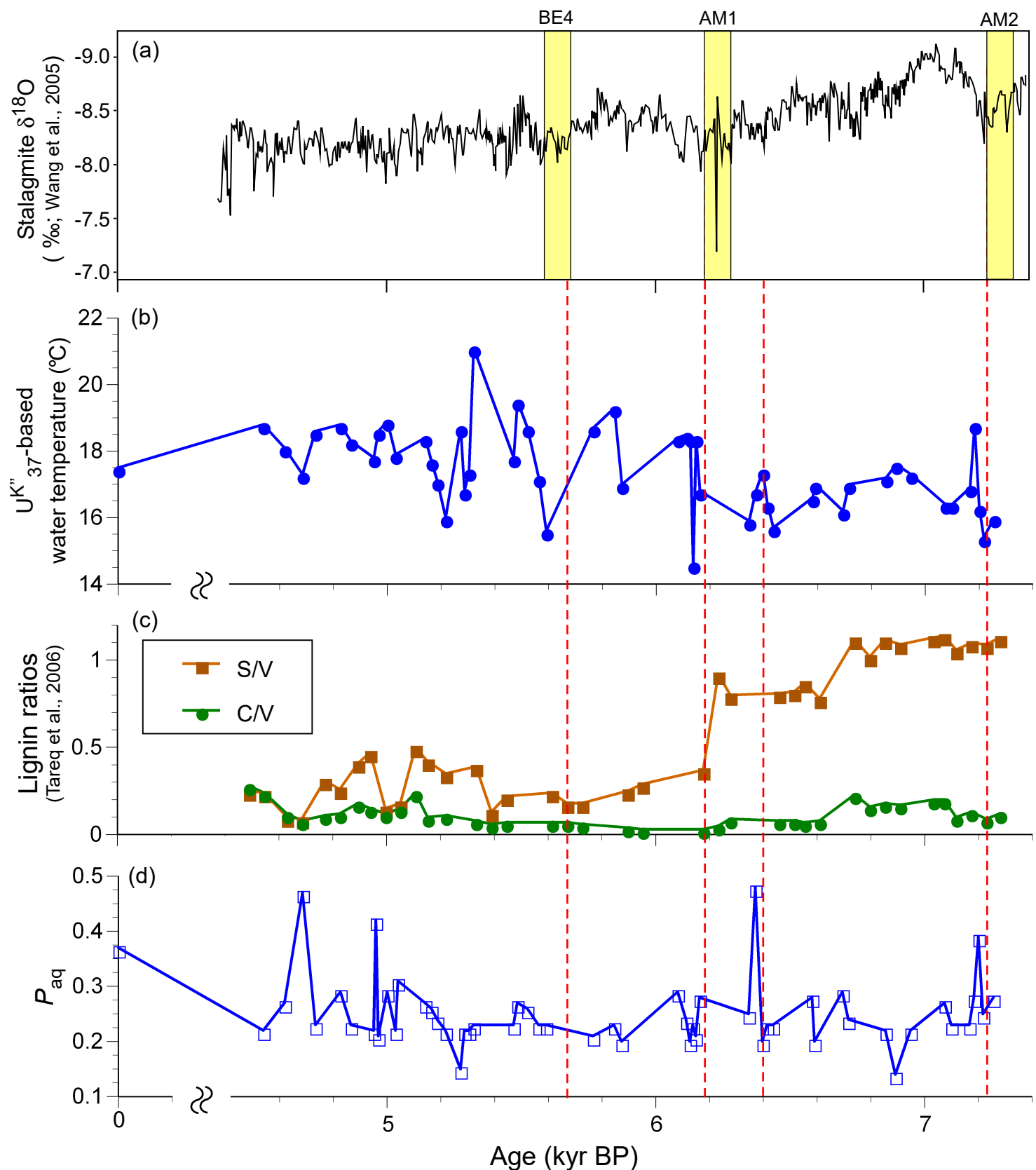
Figure 6 (a) Oxygen isotope ratio ( \delta^{18}\text{O} ) records in stalagmite of the Dongge Cave, southern China (Wang et al., 2005). AM 1 and AM 2 indicate Asian Monsoon events (Wang et al., 2005) and BE4 indicates Bond Event 4 (Bond et al., 2001). (b) Variations in \text{U}^{\text{K}^{37}} -based water temperatures estimated using the calibration obtained from R. lamellosa LG strain ( \text{U}^{\text{K}^{37}} = 0.045 T - 1.016 ; Zheng et al., 2014) in the DBB samples of Dabusu Lake. Paleovegetation records of a DBB core of Dabusu Lake; (c) variations in angiosperm / gymnosperm ratios estimated by the lignin ratios such as syringyl / vanillyl (S/V) and cinnamyl / vanillyl (C/V) ratios (Tareq et al., 2006), and (d) relative abundances of aquatic macrophytes estimated by P_{\text{aq}} values in the DBB samples of Dabusu Lake.
