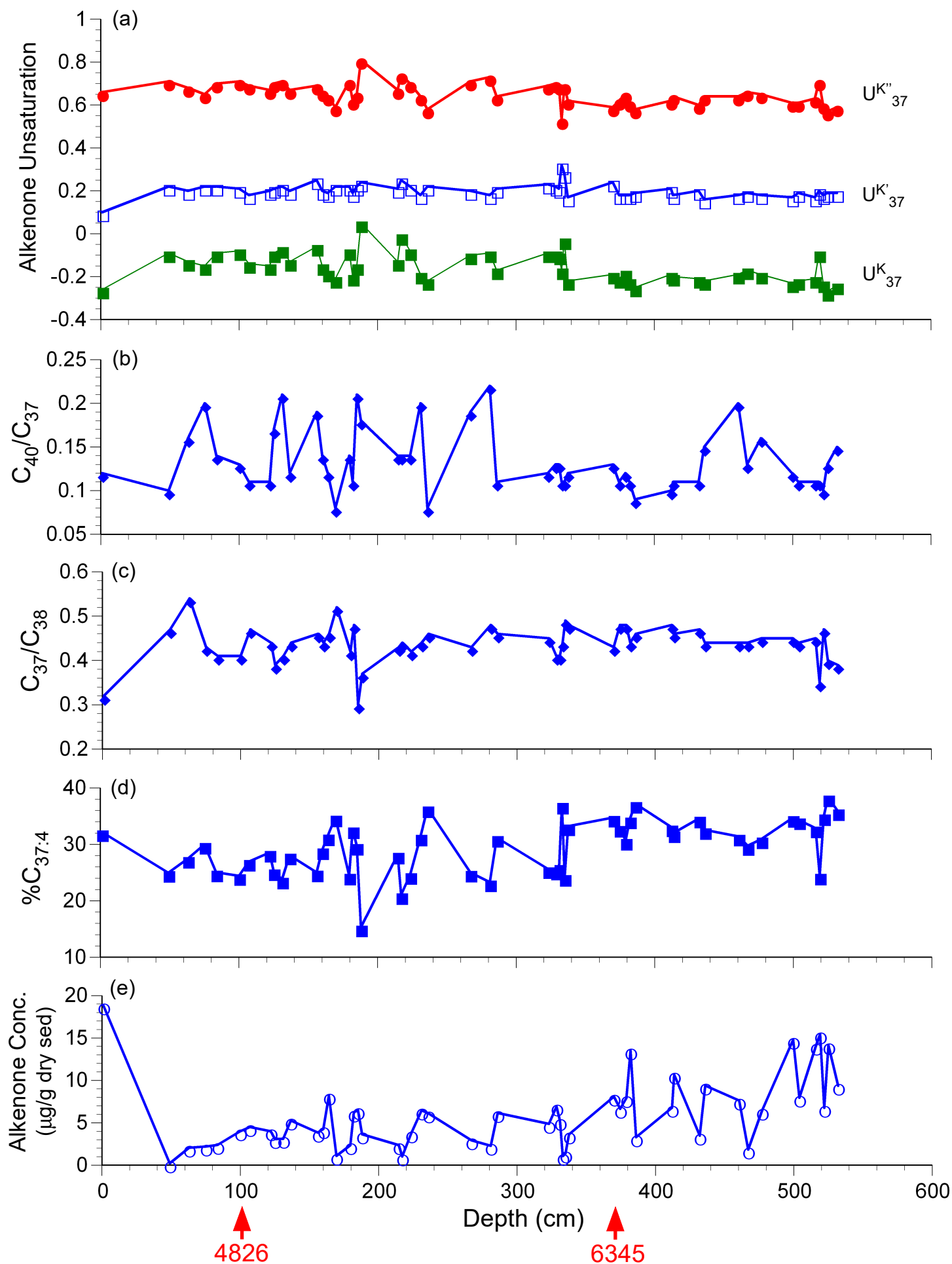
Figure 4 Depth profiles of (a) alkenone unsaturation indices ( U^K_{37} , U^{K'}_{37} , and U^{K''}_{37} ), chain length ratio of alkenones ((b) C_{40}/C_{37} , (c) C_{37}/C_{38} ), (d) the percentage of C_{37:4} alkenones ( \%C_{37:4} ), and (e) total alkenone concentrations. Calendar ages are also shown.
