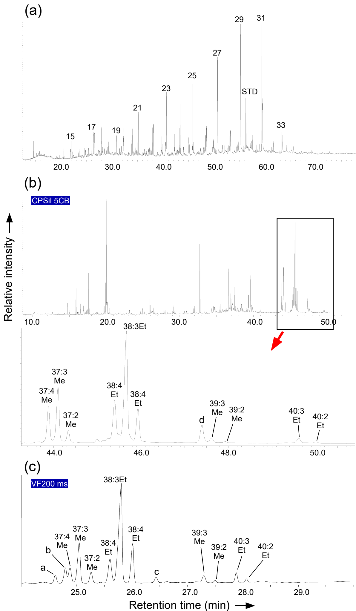
Figure 2 (a) Total ion chromatogram (TIC) of apolar fraction F1, and gas chromatograms of mid-polar fraction F3 measured with a CPSil 5CB column (b) and with a VF-200 ms column (c) of a sediment in DBB 10-4 (522 cm depth). Numbers in TIC are n -alkanes (carbon numbers). Peaks of x : y Me or Et are x carbon number methyl (Me) or ethyl (Et) alkenones with y double bonds (e.g. 37:3Me: C 37 tri-unsaturated methyl alkenone). Peaks a-d: unidentified compounds.
