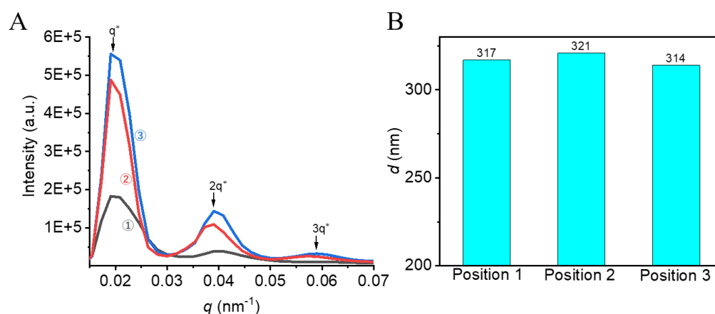
Figure S3. (A) The integrated one-dimensional (1D) SAXS intensity profiles from 2D small-angle X-ray scattering images and (B) the corresponding d -spacing at different distances from the centers shown in Figure 2A. The d is calculated by d = 2\pi/q^* . Where q^* is the first peak position in the 1D scattering profile.
