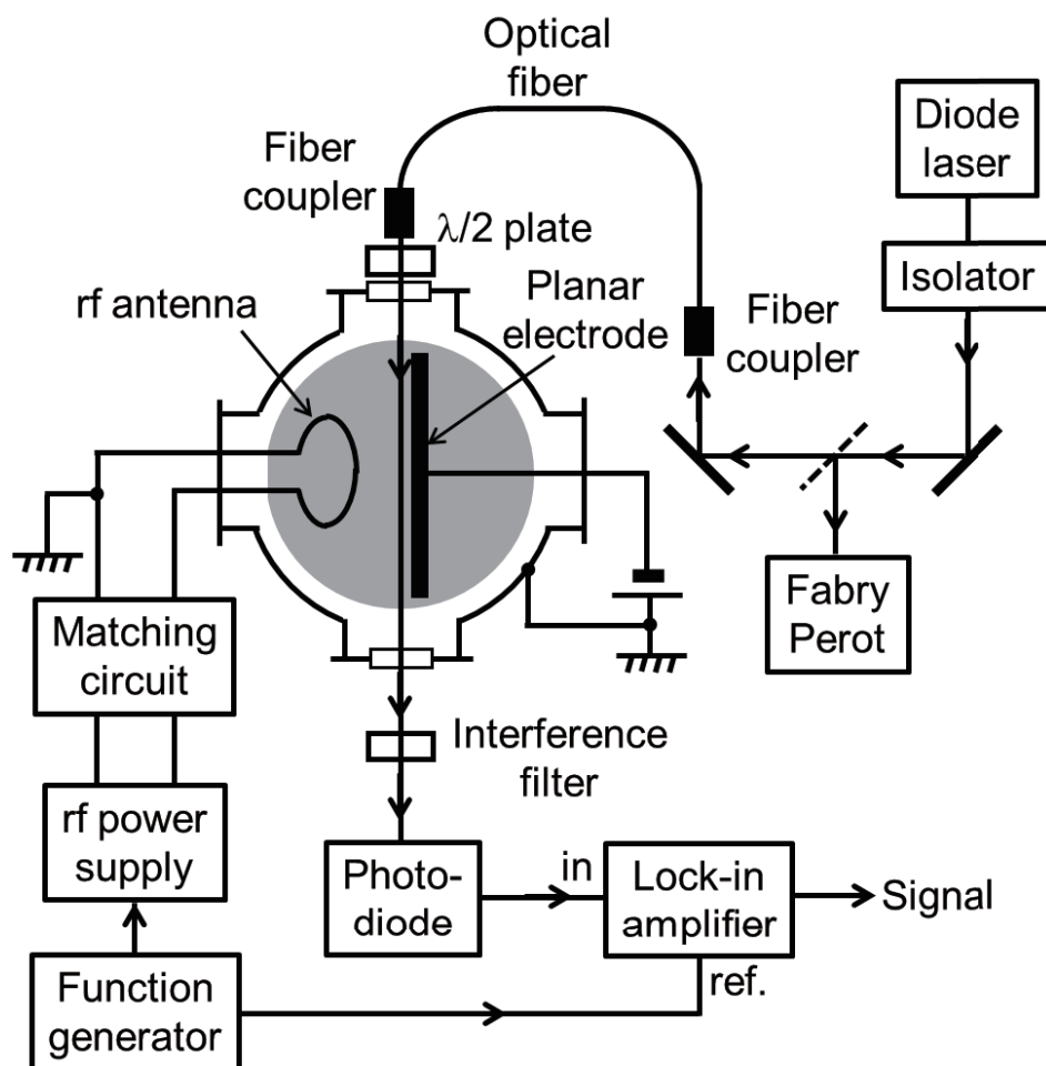
Fig. 4. Schematic of experimental apparatus.
