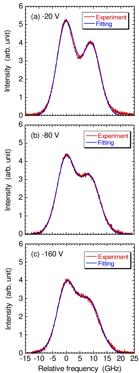
Fig. 5. Absorption spectra observed at electrode potentials of (a) -20 V, (b) -80 V, and (c) -160 V. The theoretical spectra which are fitted with experimental spectra are also shown.
