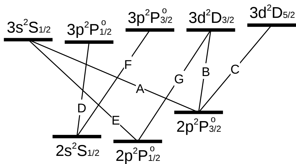
Fig. 1. Energy level diagram of atomic hydrogen relevant to the Balmer- \alpha line.
