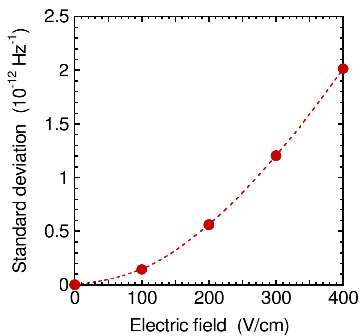
Fig. 7. Difference (given in standard deviation) between theoretical field-free spectrum and spectrum in electric fields.
