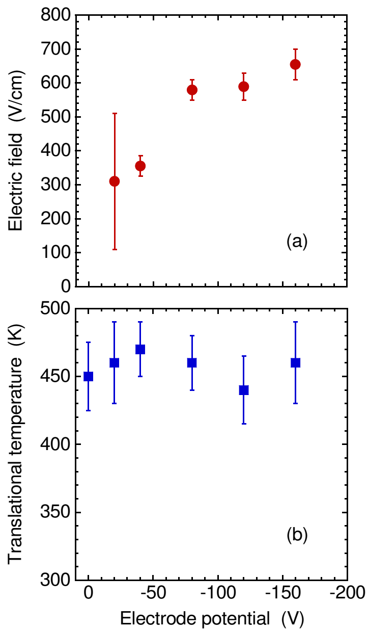
Fig. 6. (a) Electric field strength and (b) translational temperature, which are deduced by the fitting between experimental and theoretical spectra, as a function of the electrode potential.
