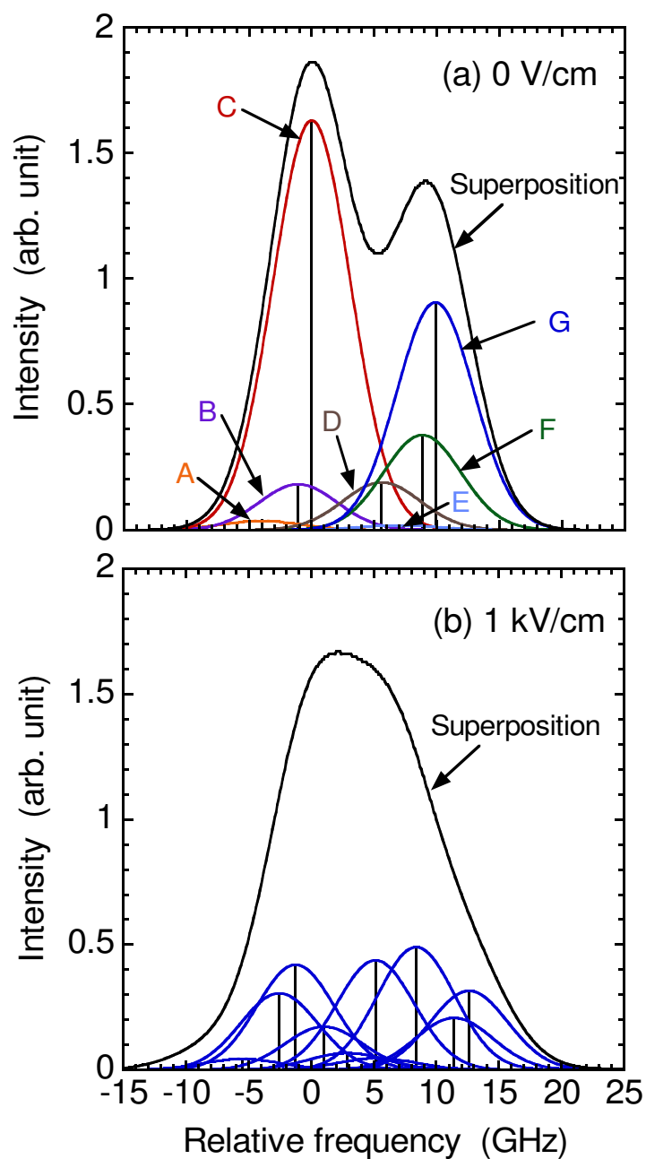
Fig. 2. Theoretical absorption spectra (a) in field-free condition and (b) in electric field of 1 kV/cm. The fine structure components (a) without and (b) with the Stark splitting are also illustrated. The Doppler broadening corresponding to 500 K is assumed for each fine structure component. The electric field of linearly polarized laser beam is assumed to be parallel to the sheath electric field. The labels A-G in (a) correspond to the transitions shown in Fig. 1.
