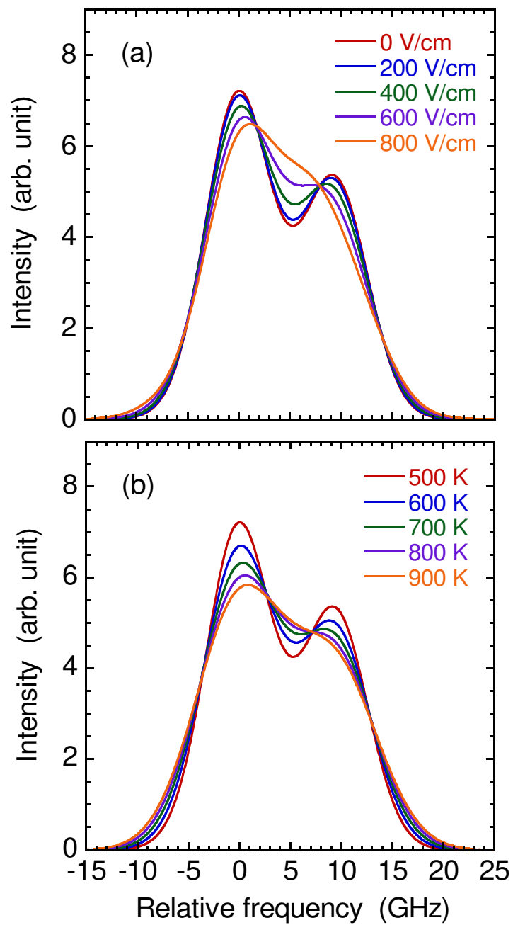
Fig. 3. Theoretical absorption spectra at (a) various electric fields and (b) various translational temperatures. The translational temperature is fixed at 500 K in (a), whereas the electric field is fixed at 0 V/cm in (b).
