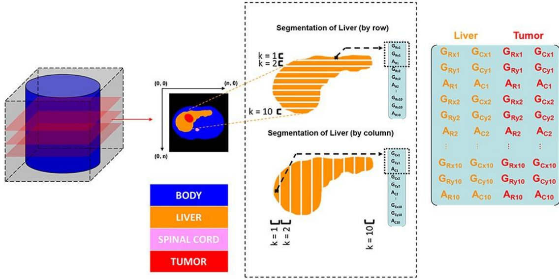
Figure 6. Profiling of the ROI from a CT slice. k : the total number of segmentations for profiling, G_{Rxi} ; The x-coordinate of the gravity center of the i th segment of liver in the horizontal segmentation. G_{Ryi} ; The y-coordinate of the gravity center of the i th segment of liver in the horizontal segmentation. A_{Ri} ; The corresponding partial area of the i th segment of liver. G_{Cxj} ; The x-coordinate of the gravity center of the j th segment of liver in the vertical segmentation. G_{Cyj} ; The y-coordinate of the gravity center of the j th segment of liver in the horizontal segmentation. A_{Cj} ; The corresponding partial area of the j th segment of liver. The parameters i and j are from 1 to 10 when we use k = 10 .
