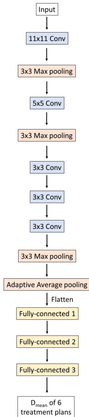
Figure 16. Alexnet-based liver D_{\text{mean}} prediction model architecture
