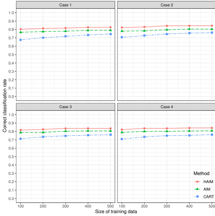
Fig. 3 The results of simulation data generated by model 3
