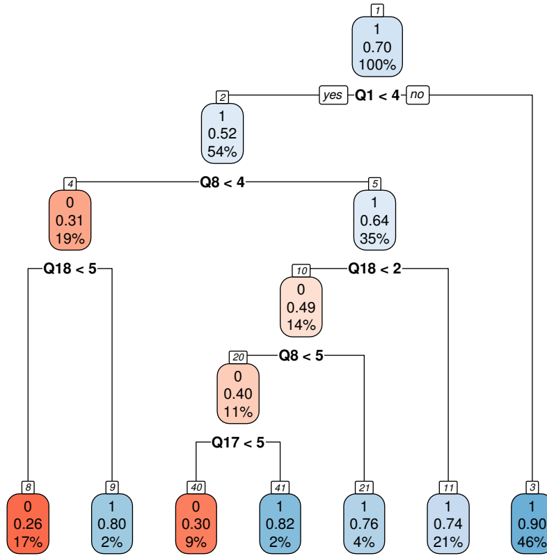
Fig. 7 The result of CART, blue boxes show the people who is satisfied with the tourist spot, red boxes show the people who is unsatisfied with the tourist spot. The middle of box shows the ratio of satisfaction(blue) or unsatisfaction(red) of tourist spot. The bottom of box shows the percentage of tourists, who satisfied the rules.
