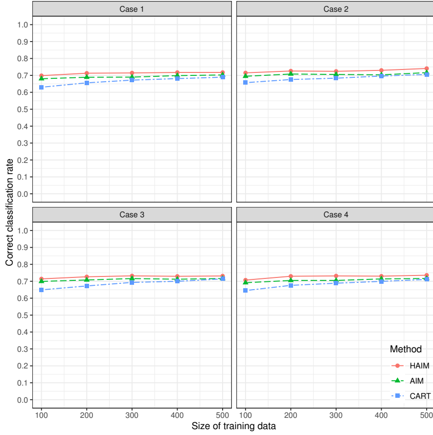
Fig. 2 The results of simulation data generated by model 2
