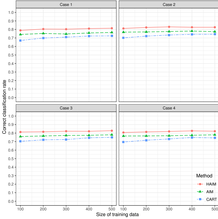
Fig. 4 The results of simulation data generated by model 4
