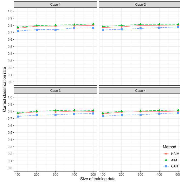
Fig. 1 The results of simulation data generated by model 1
