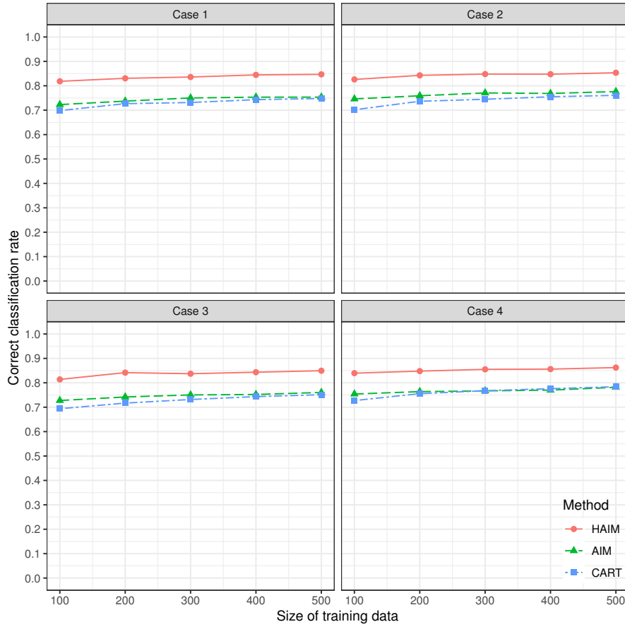
Fig. 5 The results of simulation data generated by model 5
