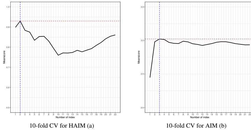
Fig. 6 The result of 10-fold-cross validation, (a) is the result of HAIM and (b) is the result of AIM. The horizontal axis shows the number of indices of HAIM and AIM. The vertical axis shows the corresponding means of score test statistics
