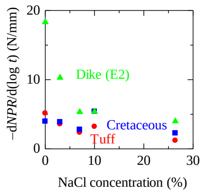
Fig. 8 Effect of salinity on the decrease rate of the needle penetration resistance.
