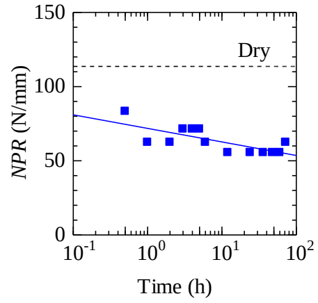
(b) Cretaceous sandstone
