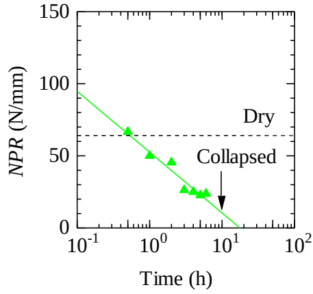
(c) Dike sandstone E2
