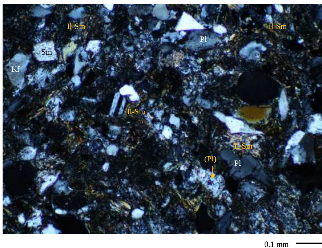
Fig. 1 A thin sectional image of the Cretaceous wacke fine-grained sandstone under crossed Nicols. Kf: potassium feldspar, PL: plagioclase, Sm: smectite, Il: illite and (): pseudomorph.
