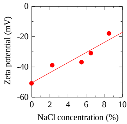
Fig. 9 Zeta potential of smectite (after Nara et al., 2014)
