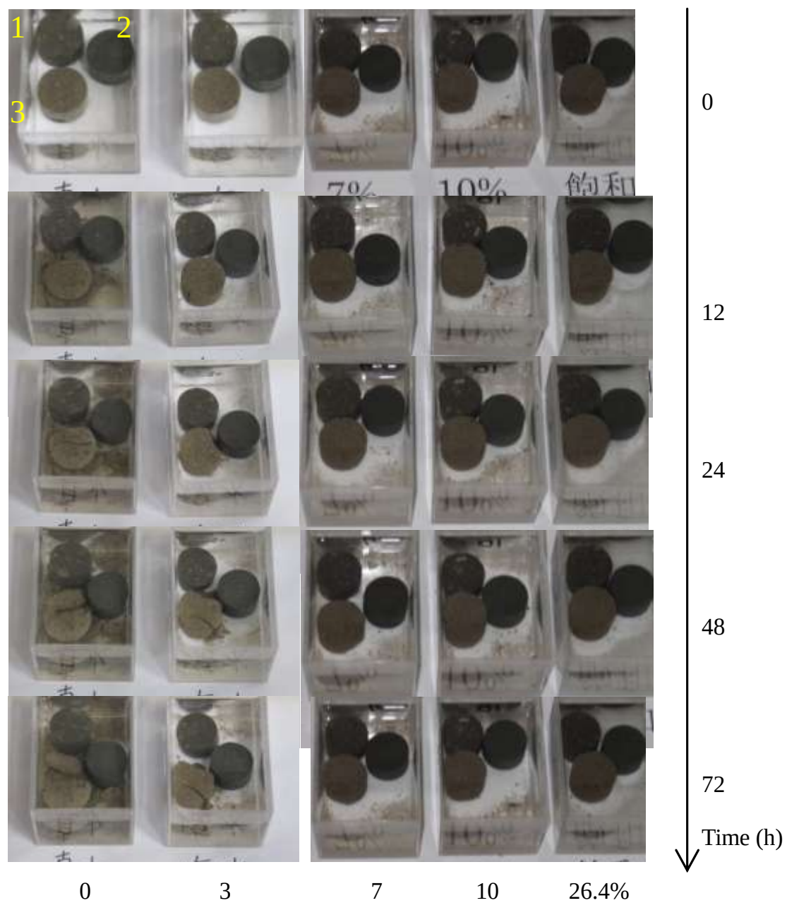
Fig. 5 Results of the jar test 1. 1: tuff, 2: Cretaceous sandstone and 3: dike sandstone E2.
