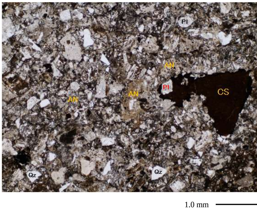
Fig. 3 A thin sectional image of the dike sandstone E2 under open Nicol. Qz: quartz, AN: andesite fragments, CS: claystone fragments.
