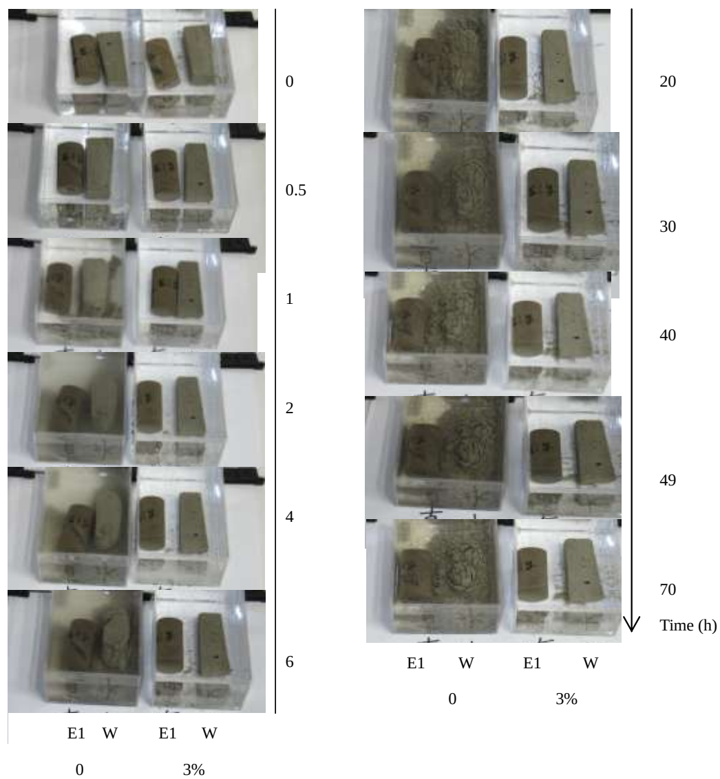
Fig. 6 Results of the jar test 2.
