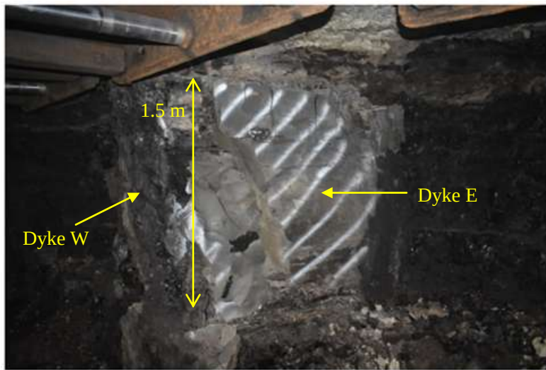
Fig. 2 Dikes E and W at the longwall coal mining face.
