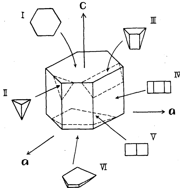
Fig. 1. Schematic diagrams of various shapes of etch pits.
