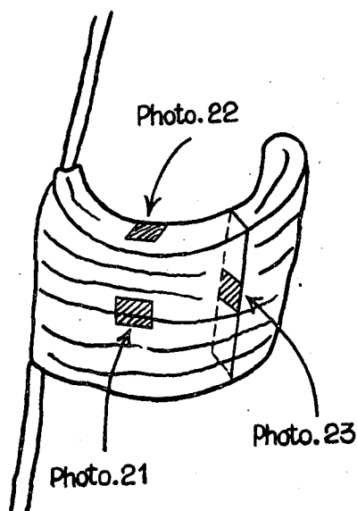
Fig. 6. Photographed parts of the ice filament grown from a plant.
