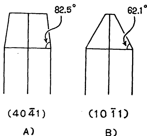
Fig. 3. Interfacial angle between crystal faces of ice.
