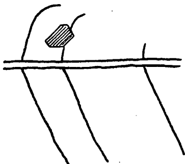
Fig. 4. Relation between the layer patterns of snow crystal and the etch pit.
