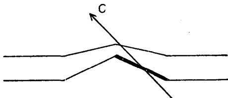
Fig. 2. Cross section of ice showing the radiating pattern.
