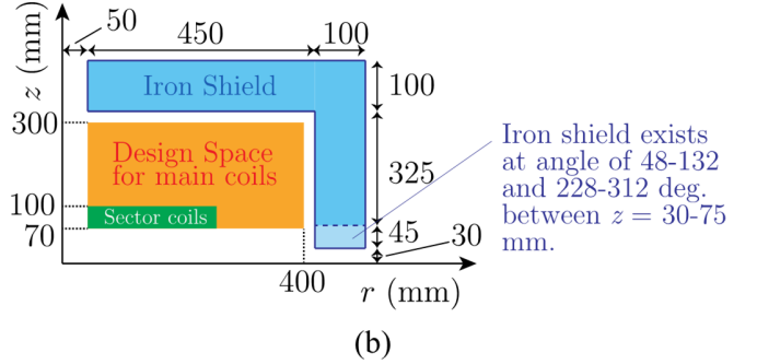
Fig. 3. (a) Top view of sector REBCO coils. (b) cross-sectional view of iron shield, sector coils, and design space for main coils. In the optimal design process, the position of the main coils to be designed is in the region of design space for main coils.
