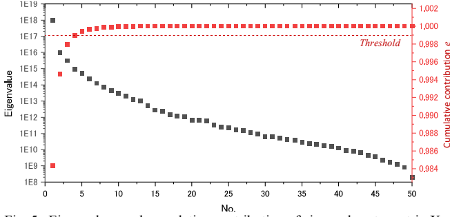
Fig. 5. Eigenvalues and cumulative contribution of eigenvalues to matrix X.
