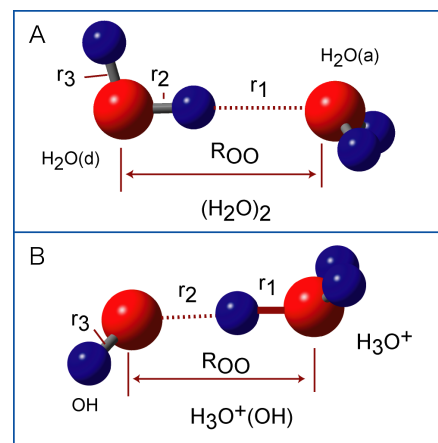
Figure 1. Optimized structures of neutral water dimer (A) and proton-transferred product (B) calculated at the MP2/6-311++G(d,p) level.
