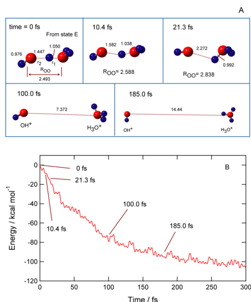
Figure 4. Snapshots (A) and potential energy curve (B) of (\text{H}_2\text{O})_2^{2+} following the vertical one-electron ionization from proton-transferred radical-ion pair ( \text{H}_3\text{O}^+-\text{OH} ). Direct AIMD calculations were carried out at the CAM-B3LYP/6-311++G(d,p) level. The MP2/6-311++G(d,p) optimized structure of \text{H}_3\text{O}^+-\text{OH} was chosen as initial structure at time zero. The values shown in (A) indicate the atomic distances in Å.
