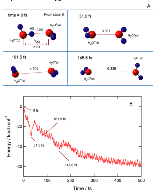
Figure 3. Snapshots (A) and potential energy curve (B) of (\text{H}_2\text{O})_2^{2+} following the vertical two-electron ionization from neutral water dimer. Direct AIMD calculations were carried out at the CAM-B3LYP/6-311++G(d,p) level. The MP2/6-311++G(d,p) optimized structure of the neutral water dimer was chosen as the initial structure at time zero. The values shown in (A) indicate the atomic distances in Å.
