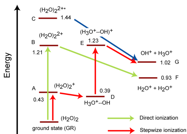
Figure 6. Summary of the present calculations. The values mean relative energies (in Hartree) calculated at the MP2/6-311++G(d,p) level.
