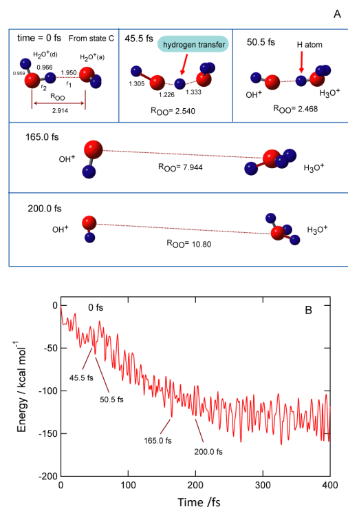
Figure 5. Snapshots (A) and potential energy curve (B) of (\text{H}_2\text{O})_2^{2+*} at first excited state following the vertical two-electron ionization from neutral water dimer. Direct AIMD calculations were carried out at the CAM-B3LYP/6-311++G(d,p) level. The MP2/6-311++G(d,p) optimized structure of neutral water dimer was chosen as initial structure at time zero. The values shown in (A) indicate the atomic distances in Å.
