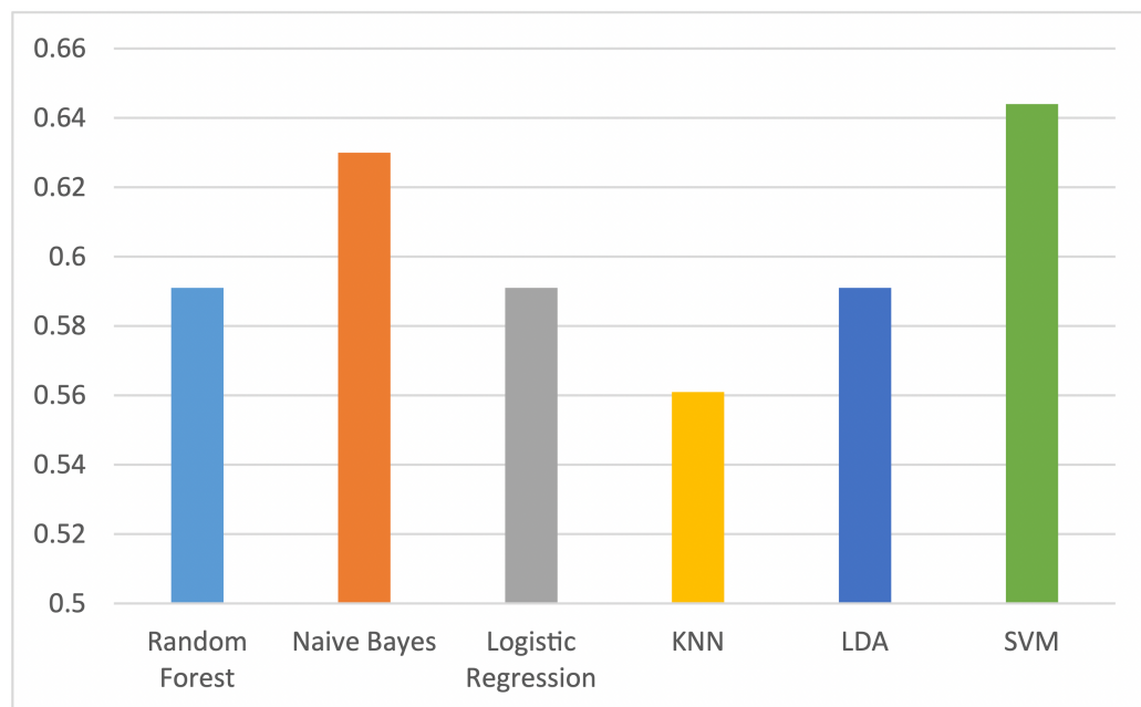
FIGURE 3.7: Results (F1-score) for all seven features
