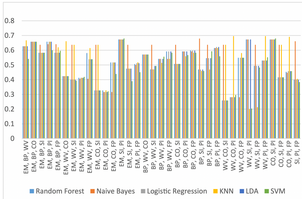
FIGURE 3.3: Results (F1-score) for three features
