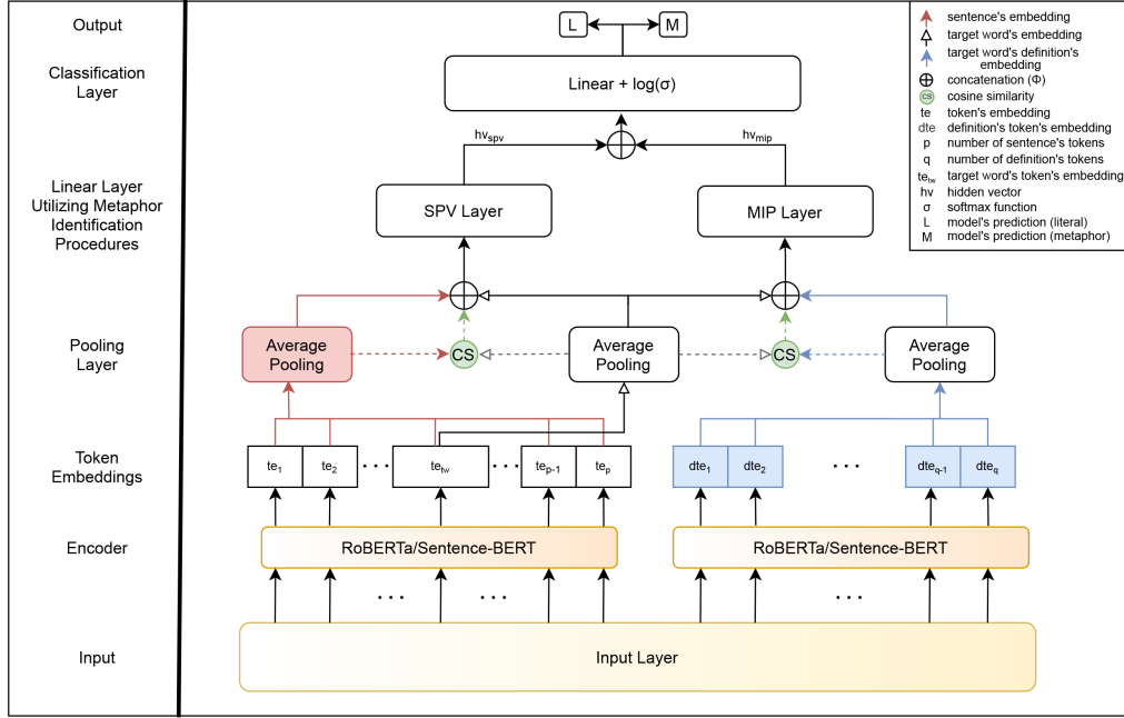
FIGURE 4.1: Model overview. Elements marked with colors other than black and white signify introduced innovations in relation to MelBERT [16]. Gradients stand for partial novelty.
