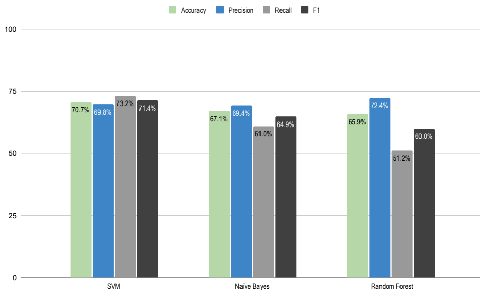
FIGURE 3.8: Bag-of-Words: Classification Results
