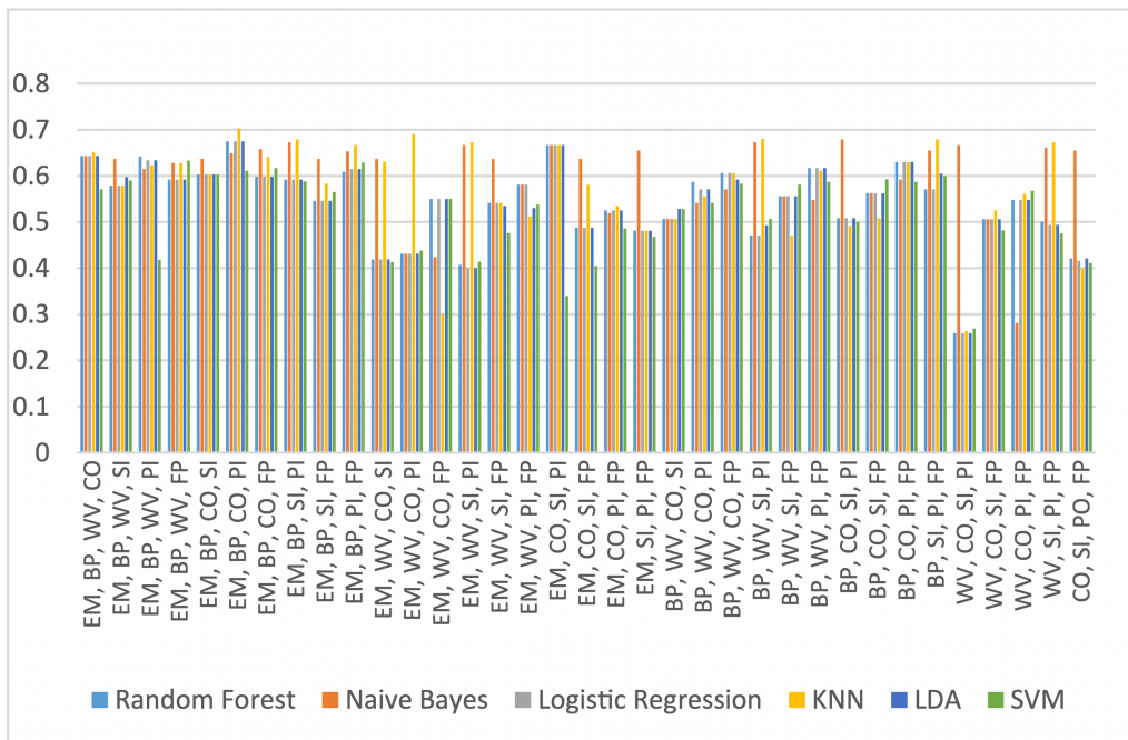
FIGURE 3.4: Results (F1-score) for four features
