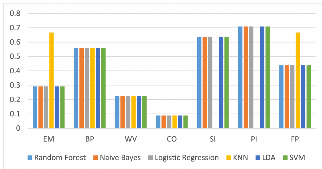
FIGURE 3.1: Results (F1-score) for a single feature
