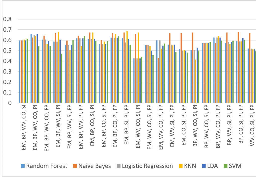
FIGURE 3.5: Results (F1-score) for five features
