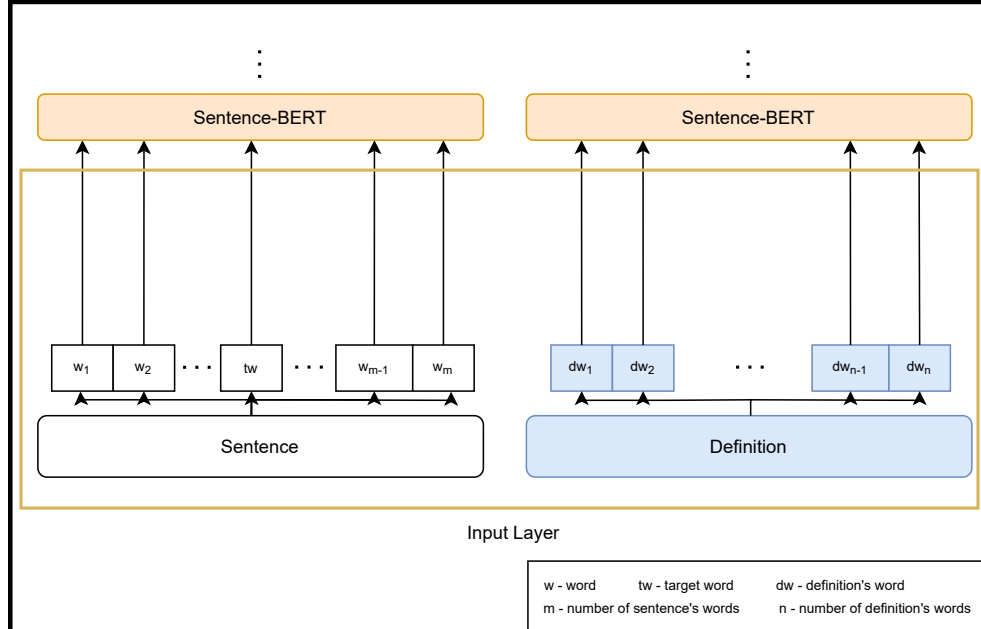
FIGURE 4.3: Input layer using Sentence-BERT. In one of the sub-models, Miss WiLDe takes advantage of Sentence-BERT instead of RoBERTa.
