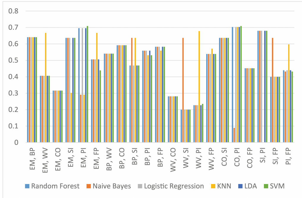
FIGURE 3.2: Results (F1-score) for two features
