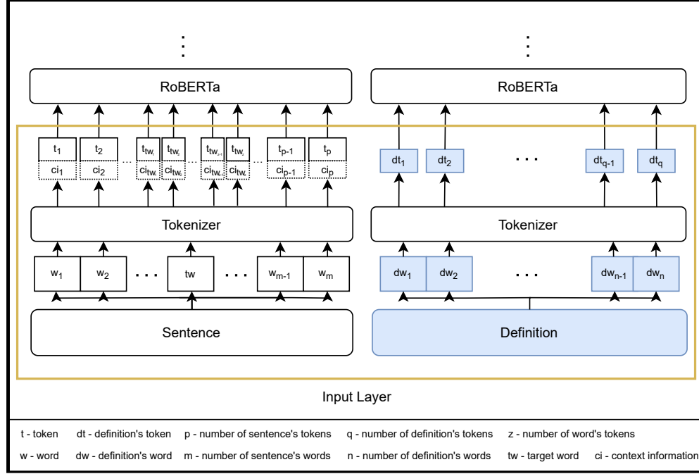
FIGURE 4.2: Input layer using RoBERTa. As single words are often divided into multiple tokens, most of the times the number of input words does not equal the number of output tokens. Context information is used to determine all the tokens that correspond to the target word.
