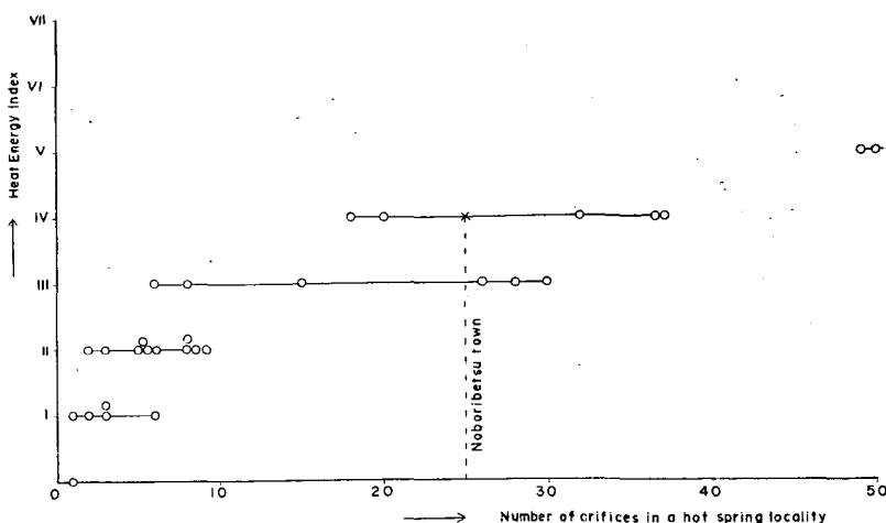
Fig. 4. Relation between the heat energy index and the corresponding number of orifices in a hot spring locality.
