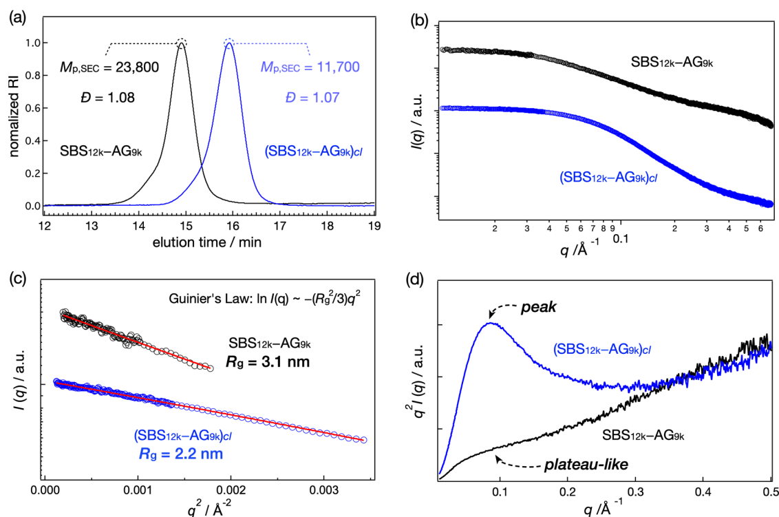
Figure 2. Structural analysis of (SBS 12k -AG 9k ) cl . (a) SEC traces (eluent, THF; flow rate, 1.0 mL min -1 ) of SBS 12k -AG 9k (black) and (SBS 12k -AG 9k ) cl (blue). (b) SAXS profiles of SBS 12k -AG 9k (black) and (SBS 12k -AG 9k ) cl (blue) in DMF (3.0 wt%). (c) Guinier plots and (d) Kratky plots of SBS 12k -AG 9k (black) and (SBS 12k -AG 9k ) cl (blue), obtained from corresponding SAXS profiles. R_g values were calculated based on Guinier's law: \ln I(q) \sim -(R_g^2/3)q^2 .
