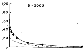
Fig. 2-5. Examples of T_{d=1}/T_0 curves for x .
