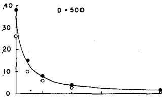
Fig. 4-3. Examples of T_{d=1}/T_0 curves for r' .
