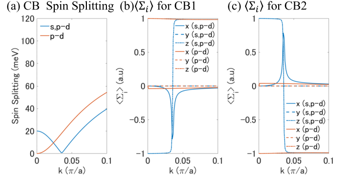
FIG. 7. (a) Spin splitting of the conduction band, and the spin orientation in (b) the lower spin state CB1 and (c) the upper spin state CB2 when 6A_{s-d} = 0.02 ( s , p - d , blue line) compared with those when A_{s-d} = 0 ( p - d , red line). Other parameter values and \mathbf{k} direction are identical to Fig. 5.
