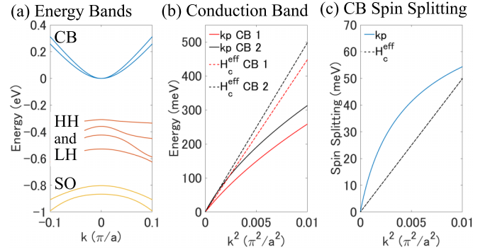
FIG. 5. (a) Energy bands, (b) the spin-split conduction bands, and (c) the spin splitting of the conduction bands in InFeAs at x = 3.8\% (solid lines) calculated in the \mathbf{k} \cdot \mathbf{p} Hamiltonian [Eq. (3)]. \mathbf{k} is in the [101] direction, and a is the lattice constant of InAs. Parameter values are given in Table II. The s - d exchange interaction is not considered ( A_{s-d} = 0 ). Dashed lines in (b) and (c) represent values obtained using H_c^{\text{eff}} [Eq. (14)].
