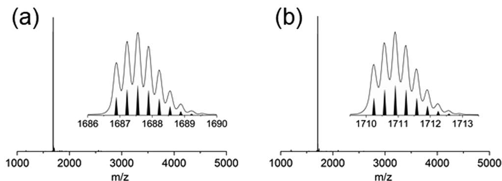
FIG. 1. ESI mass spectra of (a) 2 and (b) 3 . The insets show the comparison between experimental data and calculated isotope patterns.
