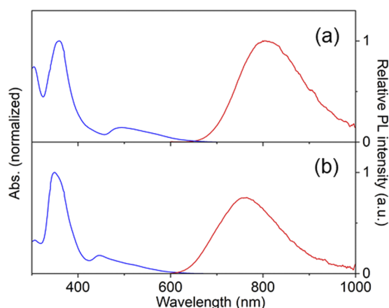
FIG. 3. Absorption (blue line) and photoluminescence (red line) spectra of (a) 1 · (\text{SbF}_6)_3 ( \lambda_{\text{ex}} = 490 nm) and (b) 3 · (\text{SbF}_6)_3 ( \lambda_{\text{ex}} = 445 nm) in MeCN.
