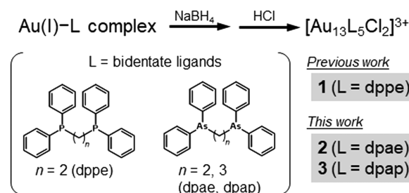
SCHEME 1. Two-step synthesis of [\text{Au}_{13}\text{L}_5\text{Cl}_2]^{3+} clusters (top). The bidentate ligands used in the previous (bottom left) and this (bottom middle) works.
