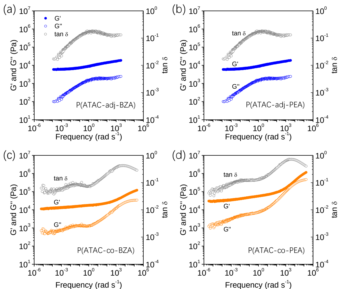
Figure 6. Master curves of storage modulus G' , loss modulus G'' , and loss factor ( \tan\delta = G''/G' ) of (a, b) P(cation-adj- \pi ) hydrogels and (c, d) P(cation-co- \pi ) hydrogels. All hydrogels were equilibrated in a 0.7 M NaCl solution.
