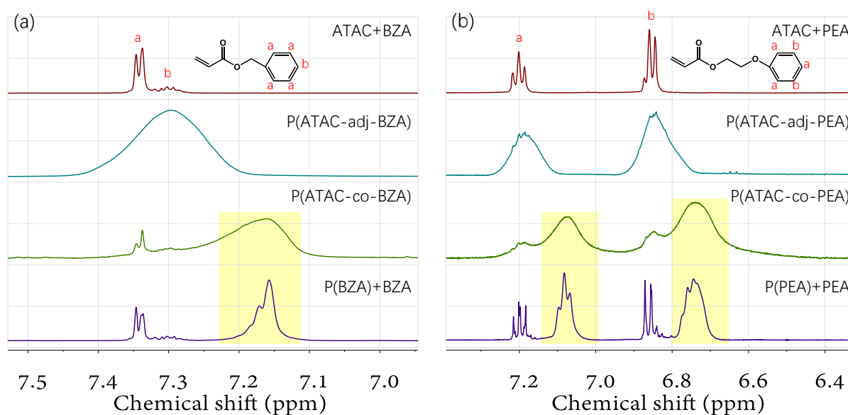
Figure 3. Partial (aromatic protons) ^1\text{H} NMR spectra of monomer mixtures, P(cation-adj- \pi ), P(cation-co- \pi ), and aromatic homopolymers containing a small number of aromatic monomers in \text{DMSO-d}_6 solution. (a) ATAC-BZA and (b) ATAC-PEA pairs. The yellow backgrounds highlight the proton peaks of long aromatic segments in polymer chains.
