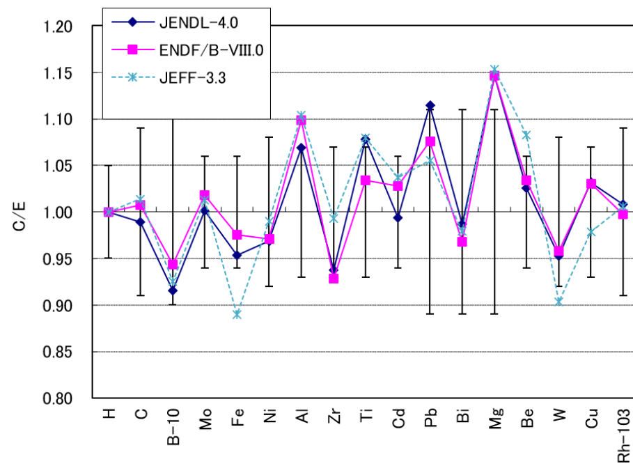
Figure 8 Normalized C/E values of the sample reactivity at SEG-6/10 with the recent nuclear data
