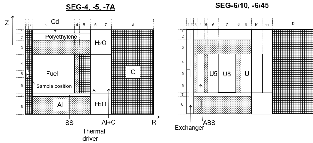
Figure 1 Cylindrical whole-core model of the SEG cores
