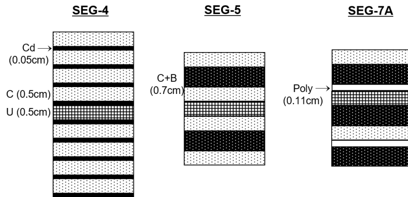
Figure 2 Unit cell configuration
