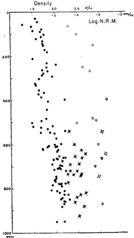
Fig. 13. Core specimens of the boring dug at the middle of Kuttuyaro Caldera. Solid circle: density saturated with water Hollow circle: intensity of N.R.M. at room temperature. Crosses denote gravel or lava fragment.
