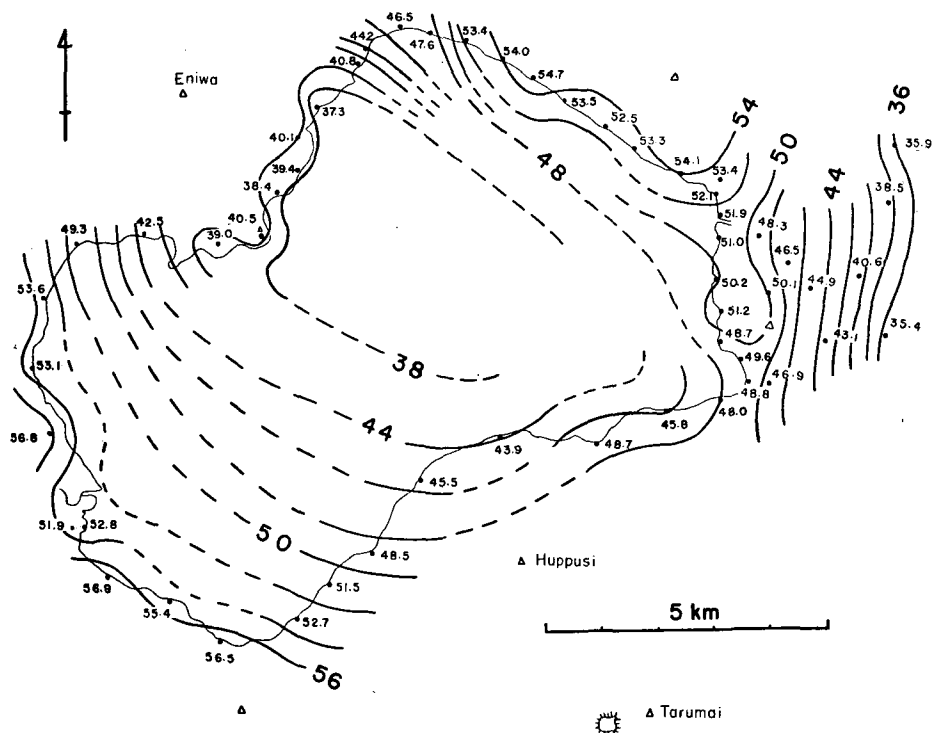
Fig. 6. Bouguer gravity anomaly in milligal (not corrected for topography).
