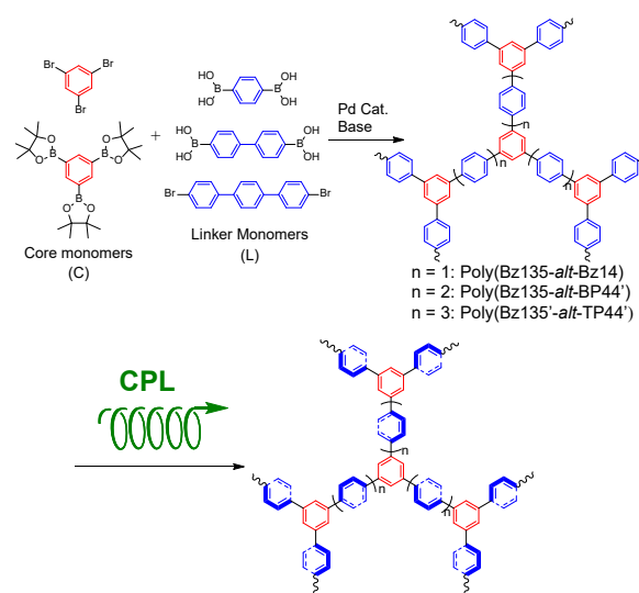
Scheme 1. Synthesis of COF's and HBP's composed of benzene rings and chirality induction them by CPL.
