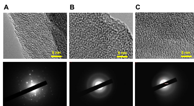
Fig. 2. TEM images (top) and electron diffraction profiles (bottom) of poly(Bz135- alt -Bz14) COF (run 4 in Table S1 in ESI) (A), poly(Bz135- alt -BP44') COF (run 3 in Table S2 in ESI) (B), and poly(Bz135- alt -TP44'') COF (run 3 in Table S3-2 in ESI) (C).
