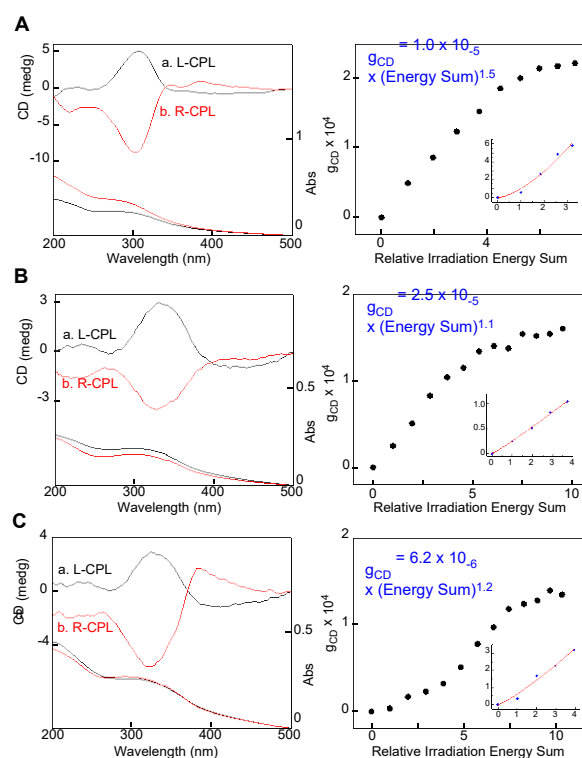
Fig. 4. CD-UV spectra observed on L-CPL (a) and R-CPL (b) irradiation [left] and g_{CD} -vs.-relative irradiation energy sum plots with curve fitting results (inset plots and corresponding equation) [right] of poly(Bz135- alt -Bz14) HBP (run 4 in Table S1 in ESI) (A), poly(Bz135- alt -BP44') HBP (run 3 in Table S2 in ESI) (B), and poly(Bz135- alt -TP44'') HBP (run 3 in Table S3-2 in ESI) (C). Maximum g_{CD} was +2.2 \times 10^{-4} at 308 nm (A), +1.6 \times 10^{-4} at 331 nm (B), and +1.4 \times 10^{-4} at 323 nm (C).
