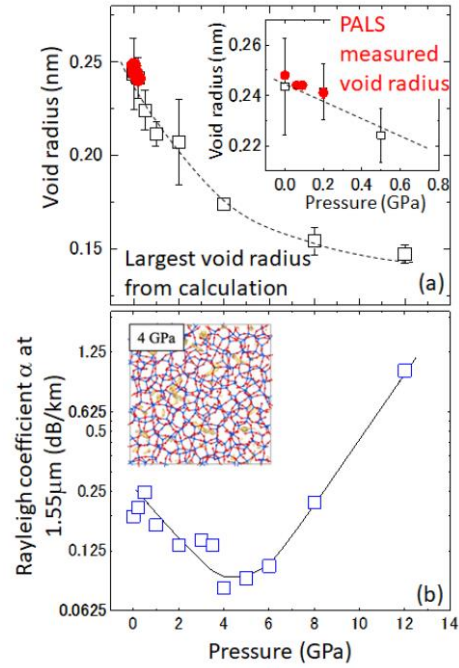
Fig. 9 Calculation results [17] . (a) Pressure dependence of the largest void radius from calculation (black) compared to the PALS-measured ones (red, data same as Fig.5 (b)). Voids continue decreasing due to pressure. Insert is the expansion of the small pressure region. (b) Calculated Rayleigh scattering coefficient at 1.55 μm, \alpha , against quenching pressure. From density fluctuation, \alpha is predicted to reduce up to the pressure of 4 GPa, but start to increase under higher pressure. Insert is the network picture of 4 GPa quenched glass. Voids are few but exist. Note that the absolute value of \alpha deviates from experimental one [15] . The minimum loss by calculation was 0.08 dB/km at 4.0 GPa.
