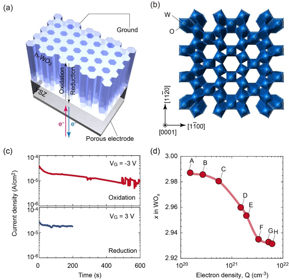
Figure 1. Solid-state electrochemical redox treatment of a h-WO x epitaxial film. (a) Schematic illustration of the solid-state electrochemical cell composed of h-WO 3 /YSZ substrate. (b) Honeycomb lattice of h-WO 3 crystal with periodic holes along the c -axis. (c) Change in the current density through the h-WO 3 /YSZ bilayer at 300 °C in air. (d) Change in the oxygen content x in h-WO x as a function of the electron density during the electrochemical reduction treatment.
