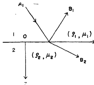
Fig. 1. Reflection and refraction of SH-waves.
