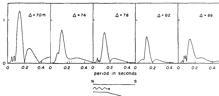
Fig. 22. Spectra at various distances for wave group III propagated from N to S.
