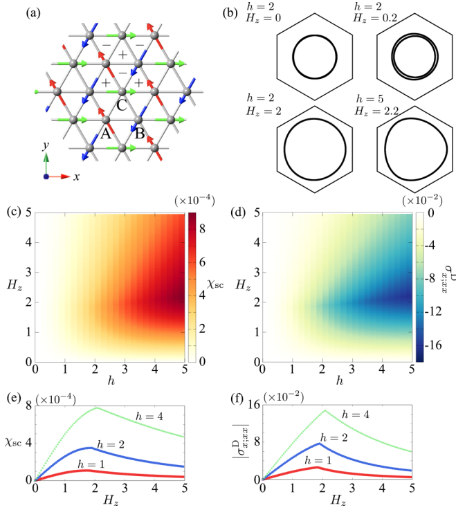
FIG. 1. (a) 120°-AFM structure on the TL. Here, + or − on the triangle represents the sign of the local spin scalar chirality \chi_{sc} under H_z . (b) Fermi surfaces at 1/10 filling for several h and H_z . (c) and (d) Contour plots of \chi_{sc} (c) and \sigma^D_{xcxc} (d) in the plane of h and H_z at 1/10 filling. (e) and (f) H_z dependences of \chi_{sc} (e) and \sigma^D_{xcxc} (f) for several h .
