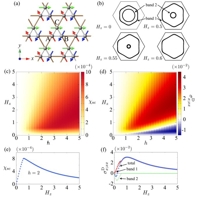
FIG. 2. (a) 120°-AFM structure in the BKL system. (b) Fermi surfaces at 1/10 filling for several H_z at h = 3 . (c) and (d) Contour plots of \chi_{sc} (c) and \sigma^D_{xcxc} (d) in the plane of h and H_z at 1/10 filling. (e) and (f) H_z dependences of \chi_{sc} (e) and \sigma^D_{xcxc} (f) for h = 2 . In (b) and (f), band 1 and band 2 represent the contributions from the lowest and second-lowest bands, respectively.
