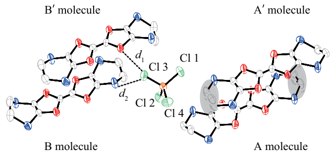
FIG. 5. ORTEP drawing of \lambda -(BEST) 2 FeCl 4 at 108 K. d_1 and d_2 represent the shortest distances from the inner and outer chalcogens to the Cl atom, respectively. Disordered ethylene groups are shaded in gray.
