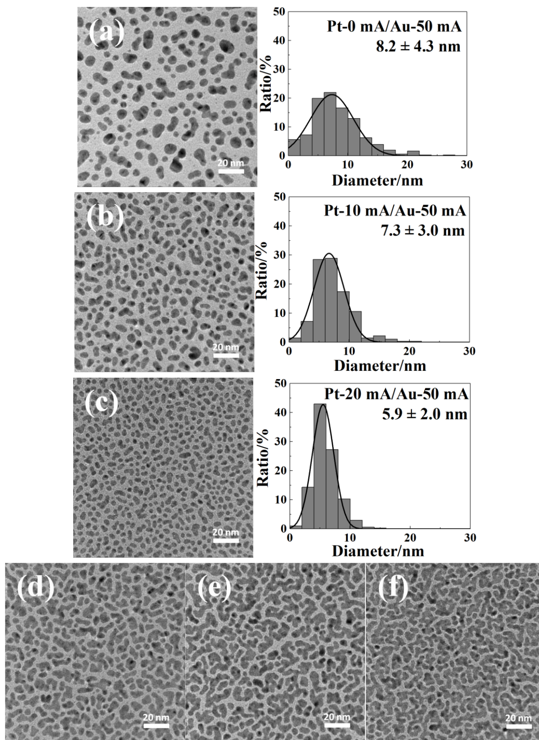
Figure S16. TEM images of NPs obtained by sputtering onto TEM grid for 30 s under various sputtering current of Pt target from 0 (a), 10 (b), 20 (c), 30 (d), 40 (e) and 50 mA (f) while keeping sputtering current of Au target constant at 50 mA.
