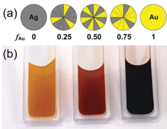
Figure 1.3 Schematic illustrations of Au-Ag foil binary targets having various f_{Au} . (b) Photographs of BMI-PF 6 obtained after the sputter deposition of Ag ( f_{Au} = 0 , left), Au/Ag ( f_{Au} = 0.50 , center) and Au ( f_{Au} = 1 , right) NPs.
