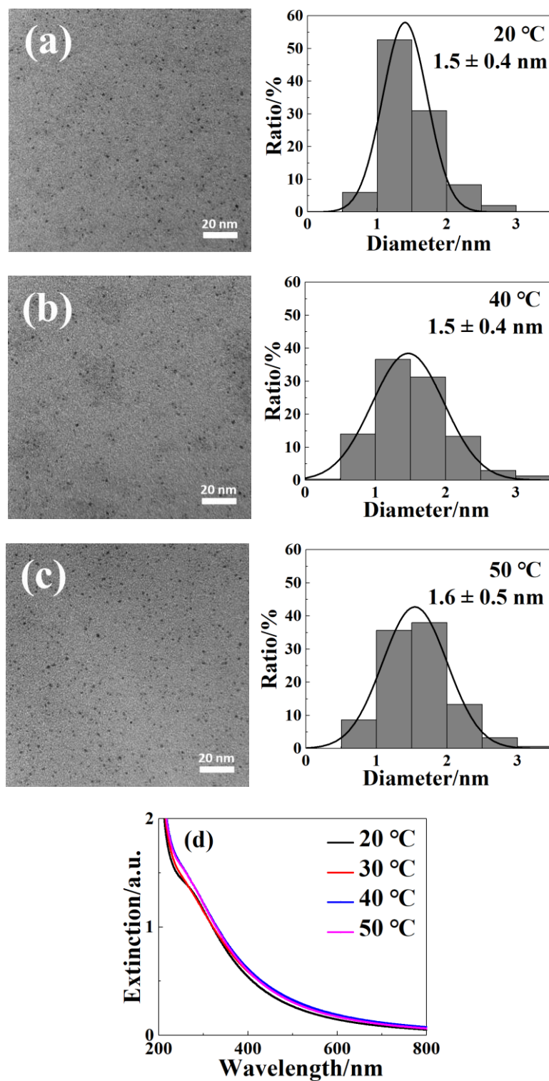
Figure S9. TEM images and the corresponding size histograms of Pt/Cu NPs obtained by continuous sputtering onto PEG at a fixed sputtering current of 30 mA and rotation speed of 80 rpm for 30 min at different PEG temperatures: (a) 20, (b) 40, and (c) 50 °C. (d) Corresponding UV-Vis absorption spectra of Pt/Cu NPs.
