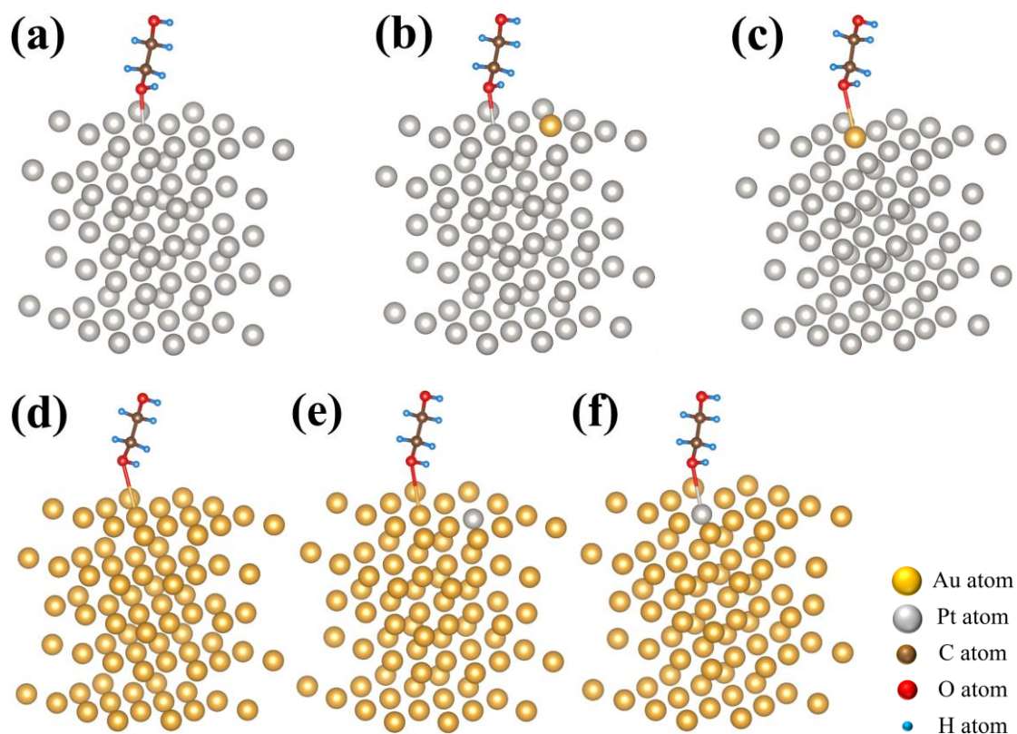
Figure S11. Final relaxed structure for PEG molecule adsorbed on Pt in Pt (111) surface (a), Pt in Pt/Au (111) surface (one Pt atom substituted by one Au atom in structure (a)) (b), Au in Pt/Au (111) surface (one Pt atom substituted by one Au atom in structure (a)) (c), Au in Au (111) surface (d), Au in Pt/Au (111) surface (one Au atom substituted by one Pt atom in structure (d)) (e), and Pt in Pt/Au (111) surface (one Au atom substituted by one Pt atom in structure (d)) (f).
