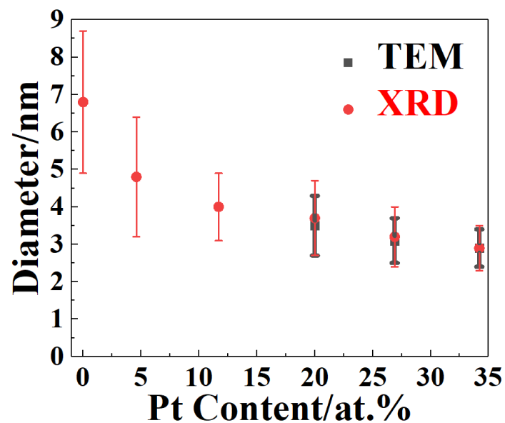
Figure S3. Changes in crystallite diameter and particle diameter with changes in proportion of Pt (at.%) in NPs. Crystallite diameter of Pt/Au NPs, calculated based on the measured 2\theta values of (111) and (200) diffraction lines.
