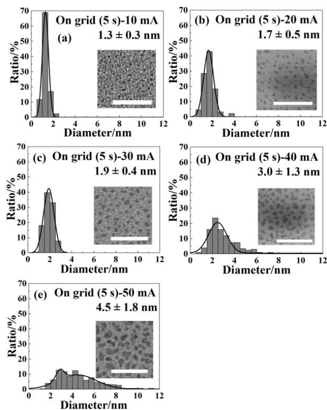
Figure 3.6 Size histograms of NPs obtained by sputtering onto TEM grids for 5 s at different sputtering currents: (a) 10 mA, (b) 20 mA, (c) 30 mA, (d) 40 mA, (e) 50 mA.
