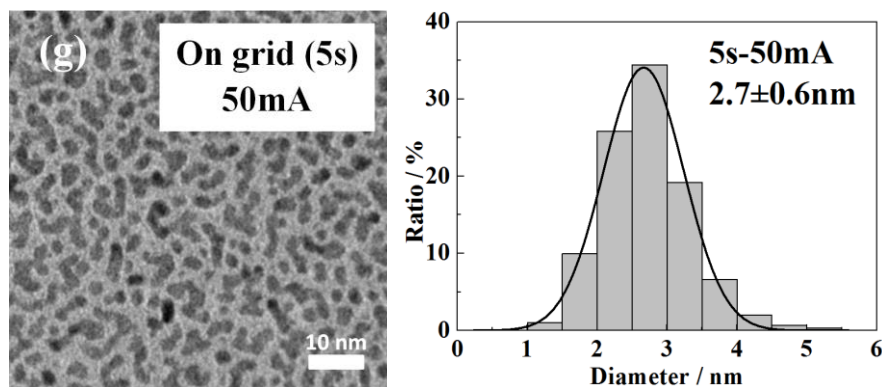
Figure S2. TEM images and size distributions of NPs obtained by sputtering on TEM grid for 5 s under sputtering current of (a) 5 mA, (b) 10 mA, (c) 15 mA, (d) 20 mA, (e) 30 mA, (f) 40 mA, (g) 50 mA.
