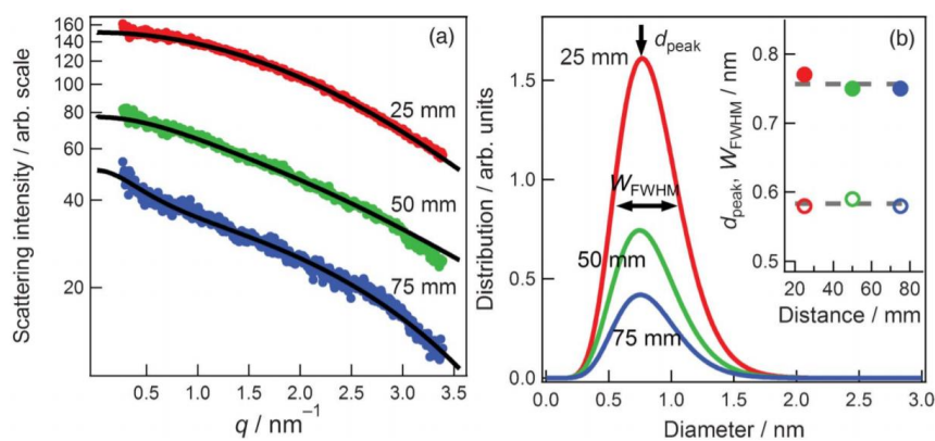
Figure 1.5 (a) The scattering profiles of the Au NPs in [\text{C}_4\text{mim}]\text{BF}_4 that were generated at working distances of 25 (red points), 50 (green points), and 75 mm (blue points). The black curves are theoretical fittings, which were obtained with the assumption that the NPs are spherical and the size distribution is expressed by C distribution. (b) The particle size distributions against the diameter for the scattering profiles of Fig. 2(a). The working distance dependences of d_{\text{peak}} (closed circles) and W_{\text{FWHM}} (open circles) are shown in the inset.
