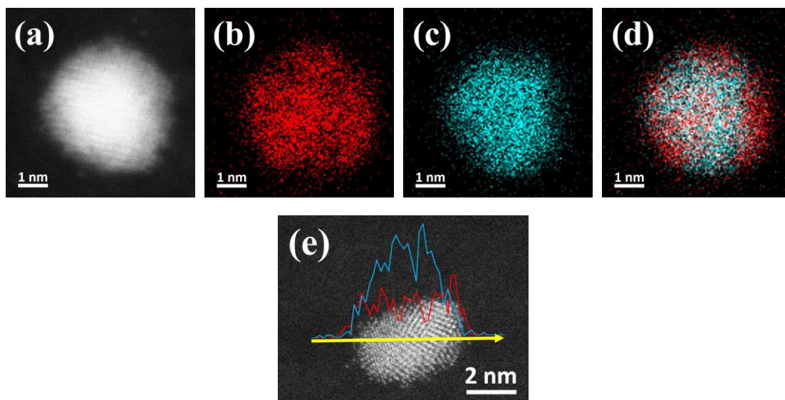
Figure 4.7 HAADF image (a) and EDX mapping results of the sample obtained by sputtering onto PEG at sputtering current of Pt-50 mA/Au-50 mA for Pt L (b), Au L (c), and overlap image of Pt and Au (d). EDX-line profile results (e) of the Pt L (red line)/Au L (blue line) for another nanoparticle of the sample. ((a)-(d) were obtained by JEOL JEM-ARM200F, operating at 80 kV, (e) were obtained by JEOL JEM-ARM200F, operating at 200 kV.)
