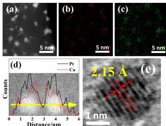
Figure 3.2 Pt/Cu NPs prepared by continuous sputtering onto PEG at a sputtering current of 50 mA for 30 min, with a rotation speed of 80 rpm at 30 °C. (a) HAADF-STEM image, corresponding EDX mapping images of (b) Pt L and (c) Cu K, (d) STEM-EDX line profile measured across two NPs; the inset shows the STEM-HAADF image of the analyzed NPs (the yellow arrow shows the scanning path for the line profile). (e) HR-TEM image of a Pt/Cu NP.
