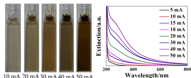
Figure 3.4 Photographs of PEG dispersions of Pt/Cu NPs under ambient light (left) and UV-Vis absorption spectra of the NPs (right) obtained by continuous sputter deposition onto PEG at different sputtering currents for 30 min at 30 °C with a rotation speed of 80 rpm.
